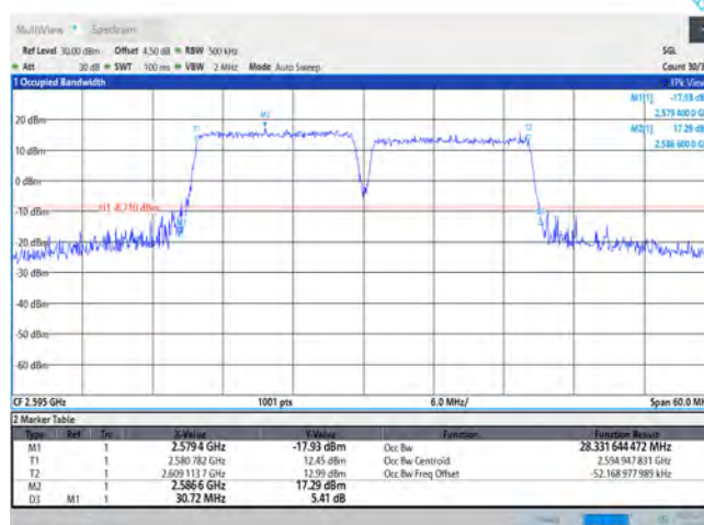
CA_38C-15MHz-15MHz-QPSK-QPSK-37925-38075-75RB#0-75RB#0
