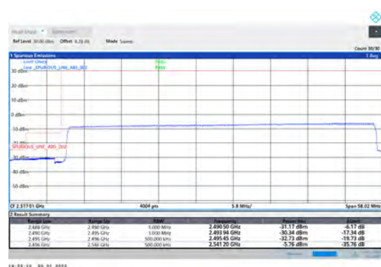
1-N41-PC3-30-50-L-6-CP-QPSK-Outer_Full-133@0-Ant1-PASS-see graph
