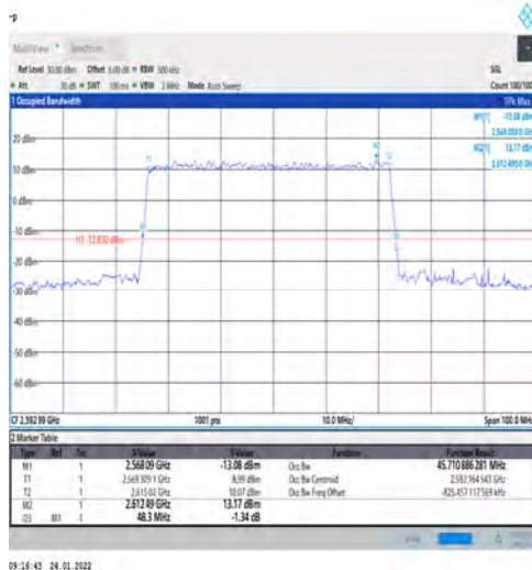
1-N41-PC3-30-50-M-4-DFT-64QAM-Outer_Full-128 @0-Ant1-45.711-48.300-≤50-PASS
