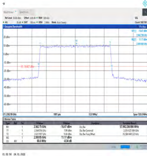
1-N41-PC3-30-60-M-5-DFT-256QAM-Outet_Full-162@ @0-Ant1-57.942-60.600-≤60-PASS
