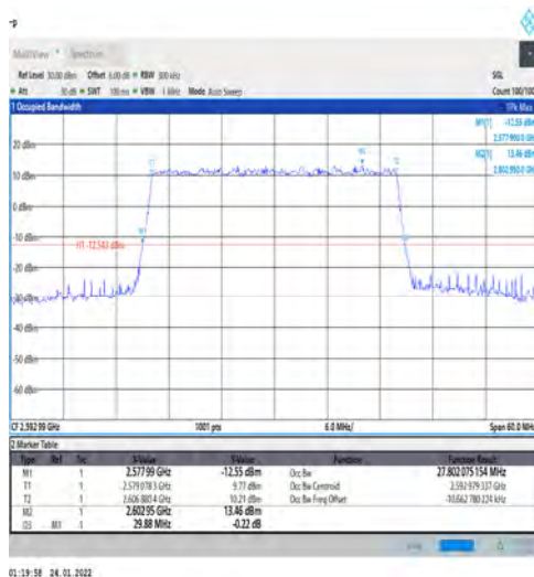
1-N41-PC3-30-30-M-6-CP-QPSK-Outer_Full-78@0- Ant1-27.802-29.880-≤30-PASS
