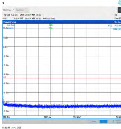
1-N41-PC3-30-100-M-1-DFT-PI2BPSK-Edge_1RB_L Left-1@0-30-1000-Ant1--58.23--35-PASS
