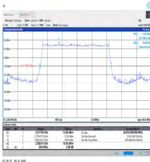
1-N41-PC3-30-30-M-2-DFT-PI2BPSK-Outer_Full-75@ 0-Ant1-26.816-28.800-≤30-PASS
