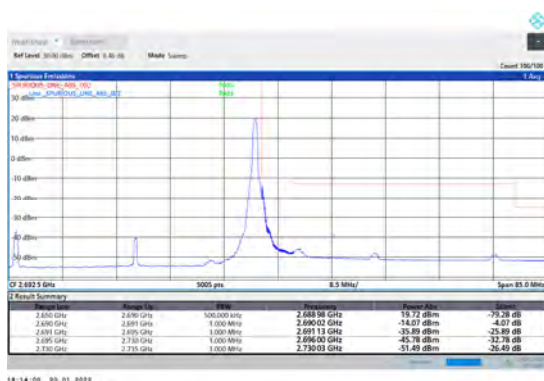
1-N41-PC3-30-40-H-2-DFT-PI2BPSK-Edge_1RB_Ri ght-1@105-Ant1-PASS-see graph
