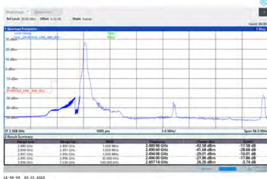
1-N41-PC3-30-40-L-1-CP-QPSK -Edge_1RB_Left-1@0-Ant1-PASS-see graph
