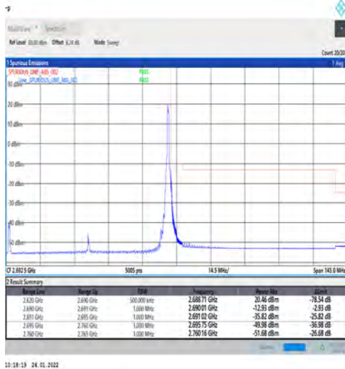
1-N41-PC3-30-70-H-2-DFT-PI2BPSK-Edge_1RB_Right@N/A-Ant1-PASS-see graph
