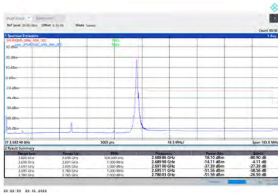
1-N41-PC3-30-90-H-5-CP-QPSK-Edge_1RB_Right-1@244-Ant1-PASS-see graph
