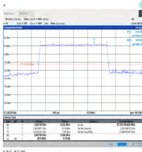
1-N41-PC3-30-50-M-7-CP-16QAM-Outer_Full-133@ 0-Ant1-47.376-49.900-≤50-PASS
