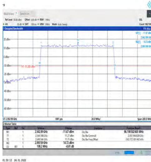
1-N41-PC3-30-100-M-3-DFT-16QAM-Outter_Full-270 @0-Ant1-96.199-100.200-≤100-PASS
