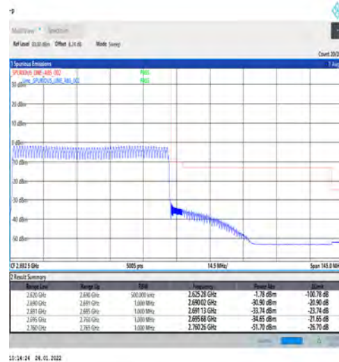
1-N41-PC3-30-70-H-6-CP-QPSK-Outer_Full-Outer_Full@N/A-Ant1-PASS-see graph
