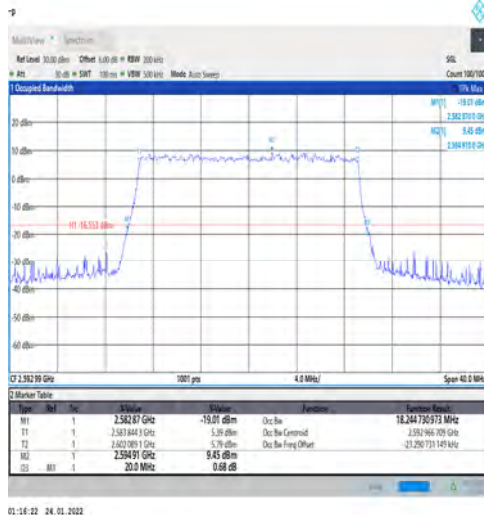
1-N41-PC3-30-20-M-9-CP-256QAM-Outer_Full-51@ 0-Ant1-18.245-20.000-≤20-PASS
