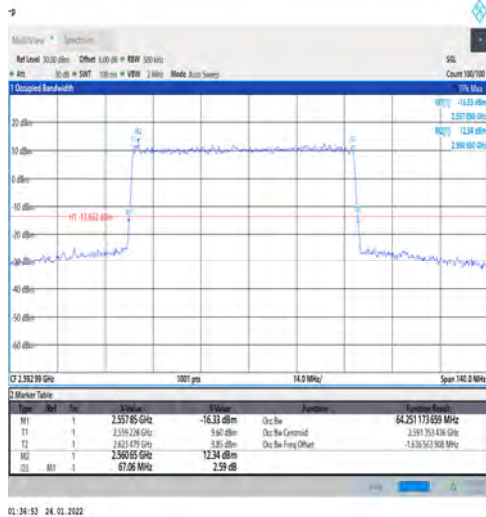
1-N41-PC3-30-70-M-4-DFT-64QAM-Outer_Full-Oute r_Full@N/A-Ant1-64.251-67.060-≤70-PASS
