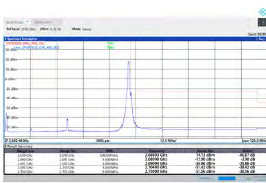
1-N41-PC3-30-60-H-5-CP-QPSK-Edge_1RB_Right-1@161-Ant1-PASS-see graph
