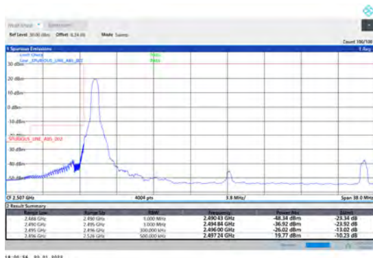
1-N41-PC3-30-30-L-1-DFT-PI2BPSK-Edge_1RB_Left-1@0-Ant1-PASS-see graph
