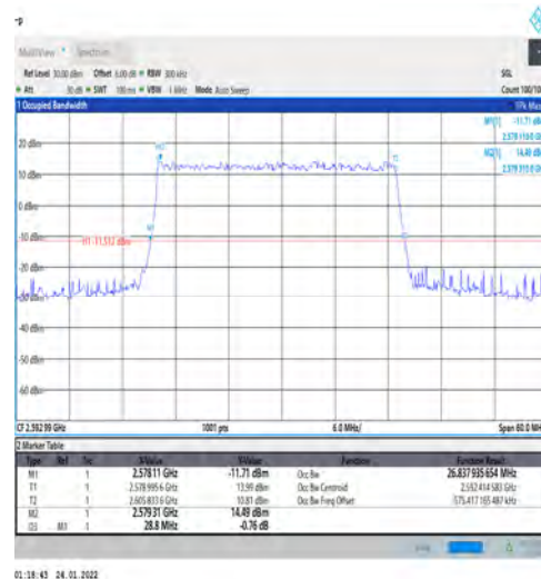
1-N41-PC3-30-30-M-3-DFT-16QAM-Outer_Full-75@ 0-Ant1-26.838-28.800-≤30-PASS
