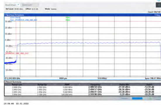
1-N41-PC3-30-100-L-6-CP-QPSK-Outer_Full-273@ 0-Ant1-PASS-see graph
