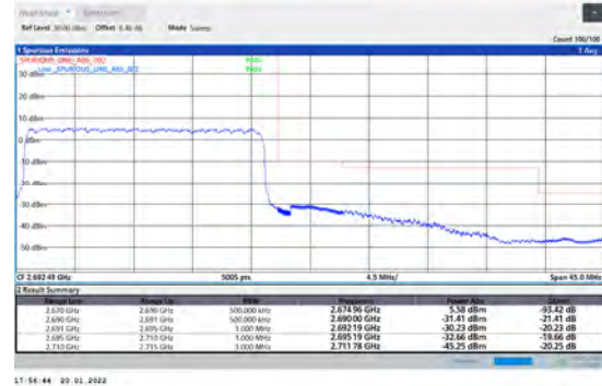
1-N41-PC3-30-20-H-3-DFT-PI2BPSK-Outer_Full-50@0-Ant1-PASS-see graph
