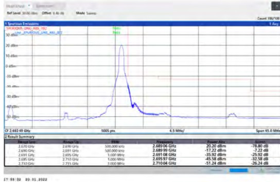
1-N41-PC3-30-20-H-2-DFT-PI2BPSK-Edge_1RB_Right-1@50-Ant1-PASS-see graph
