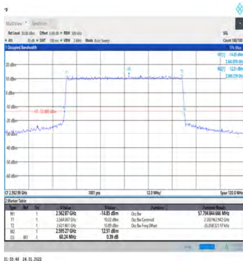
1-N41-PC3-30-60-M-7-CP-16QAM-Outet_Full-162@ 0-Ant1-57.795-60.240-≤60-PASS
