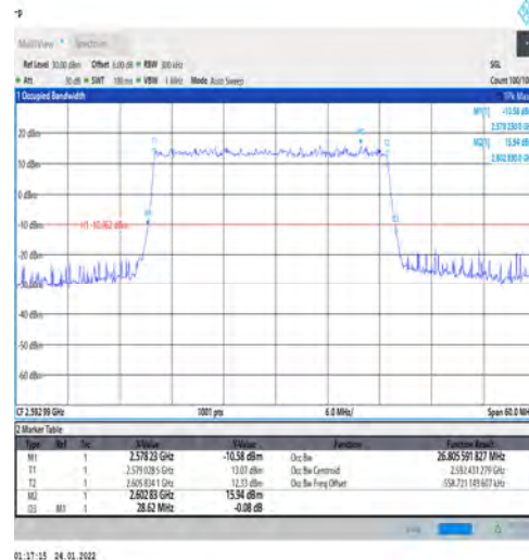
1-N41-PC3-30-30-M-1-DFT-QPSK-Outer_Full-75@0- Ant1-26.806-28.620-≤30-PASS
