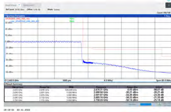
1-N41-PC3-30-40-H-6-CP-QPSK-Outer_Full-106@0-Ant1-PASS-see graph
