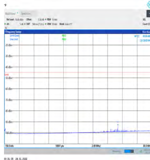
1-N41-PC3-30-100-M-1-DFT-PI2BPSK-Edge_1RB_L eft-1@0-0.15-30-Ant1--93.60--45-PASS
