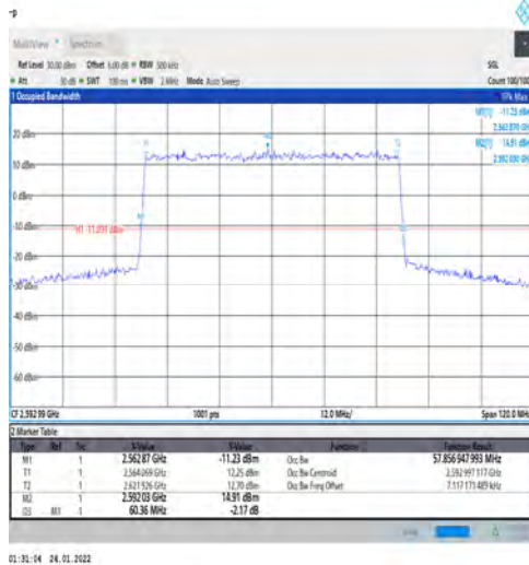
1-N41-PC3-30-60-M-1-DFT-QPSK-Outer_Full-162@ 0-Ant1-57.857-60.360-≤60-PASS
