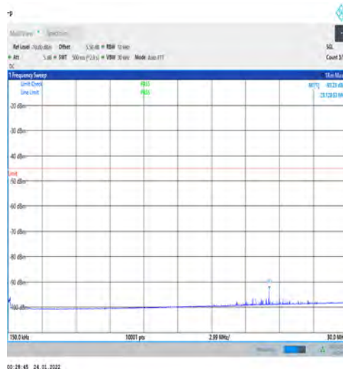
1-N41-PC3-30-100-L-1-DFT-PI2BPSK-Edge_1RB_L eft-1@0-0.15-30-Ant1--93.23--45-PASS
