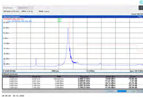
1-N41-PC3-30-50-H-2-DFT-PI2BPSK-Edge_1RB_Ri ght-1@132-Ant1-PASS-see graph
