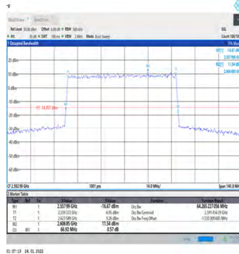
1-N41-PC3-30-70-M-5-DFT-256QAM-Outer_Full-Out er_Full@N/A-Ant1-64.265-66.920-≤70-PASS
