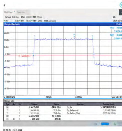
1-N41-PC3-30-60-M-4-DFT-64QAM-Outer_Full-162@ 0-Ant1-57.843-60.600-≤60-PASS
