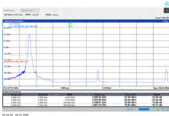
1-N41-PC3-30-50-L-1-DFT-PI2BPSK-Edge_1RB_Lef t-1@0-Ant1-PASS-see graph
