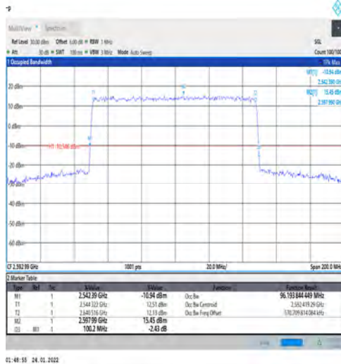
1-N41-PC3-30-100-M-1-DFT-QPSK-Outter_Full-270 @0-Ant1-96.194-100.200-≤100-PASS
