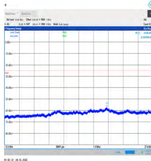
1-N41-PC3-30-100-M-1-DFT-PI2BPSK-Edge_1RB_L eft-1@0-12000-27000-Ant1--56.98--25-PASS
