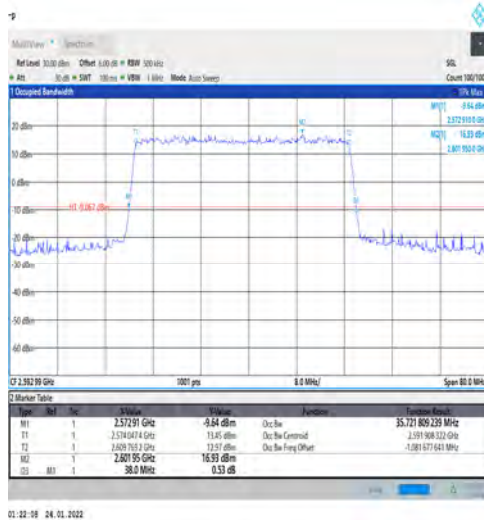
1-N41-PC3-30-40-M-1-DFT-QPSK-Outer_Full-100@0-Ant1-35.722-38.000-≤40-PASS
