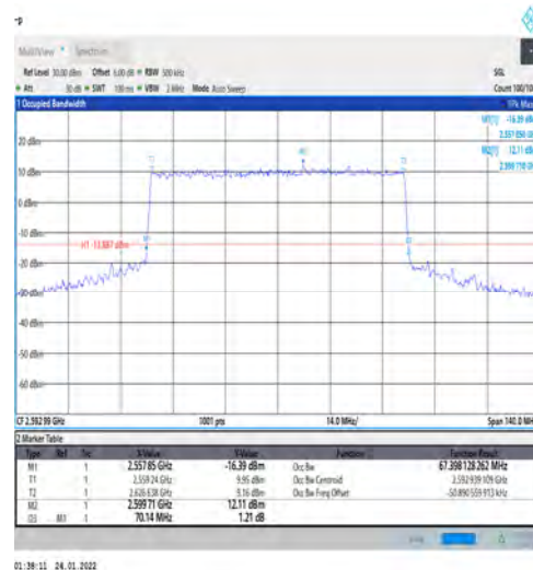
1-N41-PC3-30-70-M-7-CP-16QAM-Outer_Full-Outer Full@N/A-Ant1-67.398-70.140-≤70-PASS
