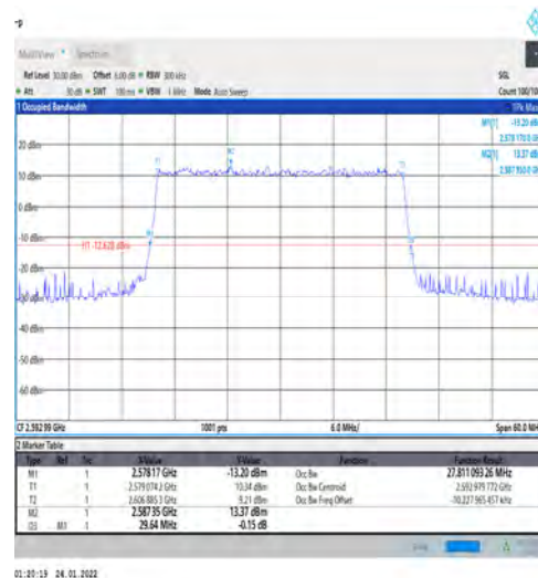
1-N41-PC3-30-30-M-7-CP-16QAM-Outer_Full-78@0- Ant1-27.811-29.640-≤30-PASS
