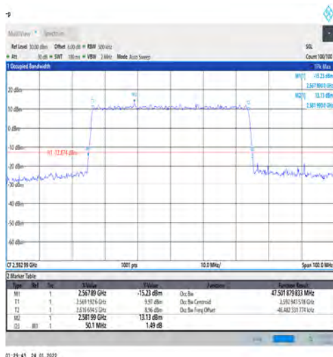
1-N41-PC3-30-50-M-8-CP-64QAM-Outer_Full-133@ 0-Ant1-47.502-50.100-≤50-PASS
