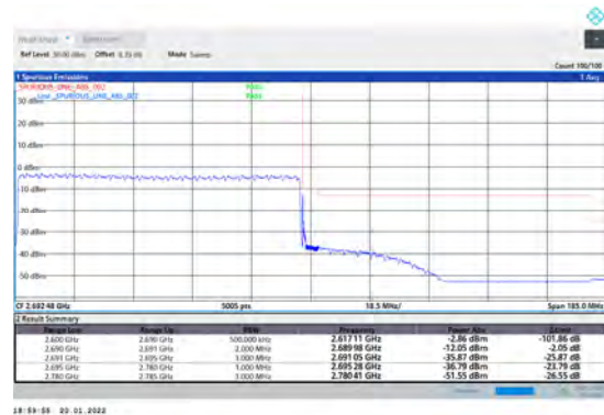
1-N41-PC3-30-90-H-6-CP-QPSK-Outer_Full-245@0-Ant1-PASS-see graph
