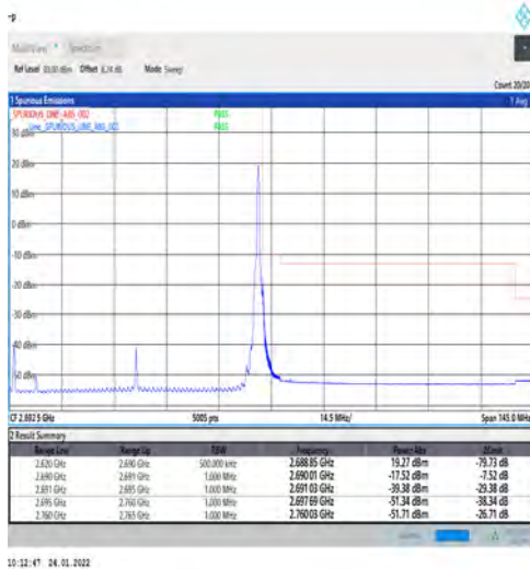
1-N41-PC3-30-70-H-5-CP-QPSK-Edge_1RB_Right-Edge_1_Right@N/A-Ant1-PASS-see graph
