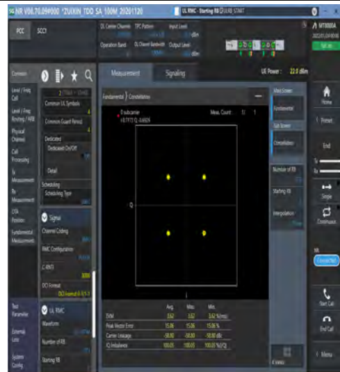
1-N41-PC3-30-100-M-6-CP-QPSK-Outer_Full-273 @0-Ant1-see graph-PASS
