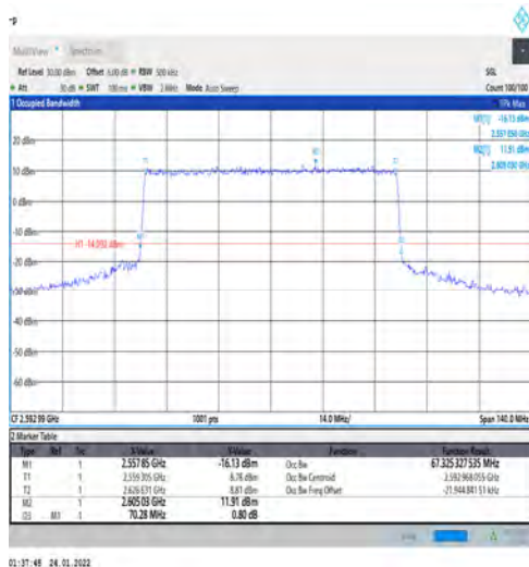
1-N41-PC3-30-70-M-6-CP-QPSK-Outer_Full-Outer_ Full@N/A-Ant1-67.325-70.280-≤70-PASS
