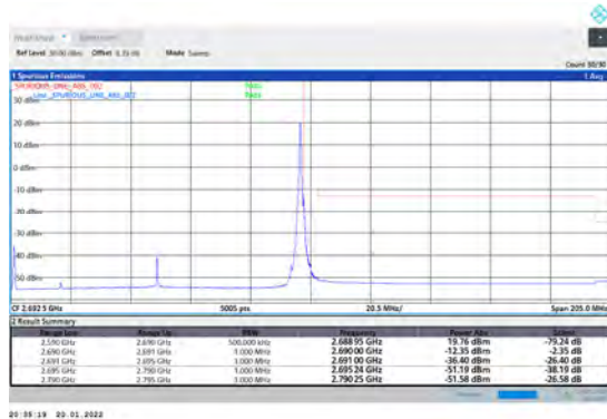
1-N41-PC3-30-100-H-2-DFT-PI2BPSK-Edge_1RB_ Right-1@272-Ant1-PASS-see graph
