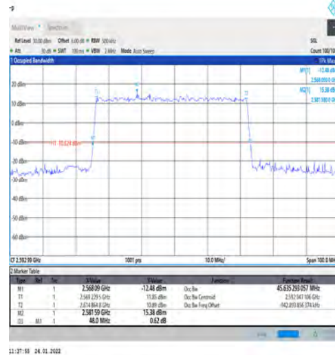
1-N41-PC3-30-50-M-3-DFT-16QAM-Outer_Full-128 @0-Ant1-45.635-48.000-≤50-PASS
