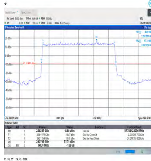
1-N41-PC3-30-60-M-2-DFT-PI2BPSK-Outer_Full-162@ 0-Ant1-57.785-60.240-≤60-PASS
