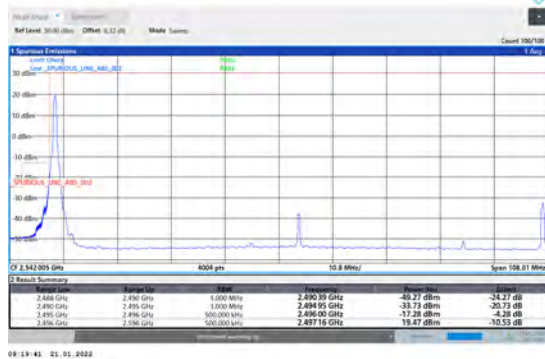
1-N41-PC3-30-100-L-4-CP-QPSK-Edge_1RB_Left-1 @0-Ant1-PASS-see graph
