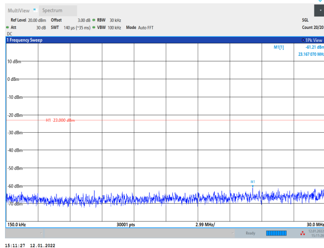
Band2-9262-0.15~30MHz
