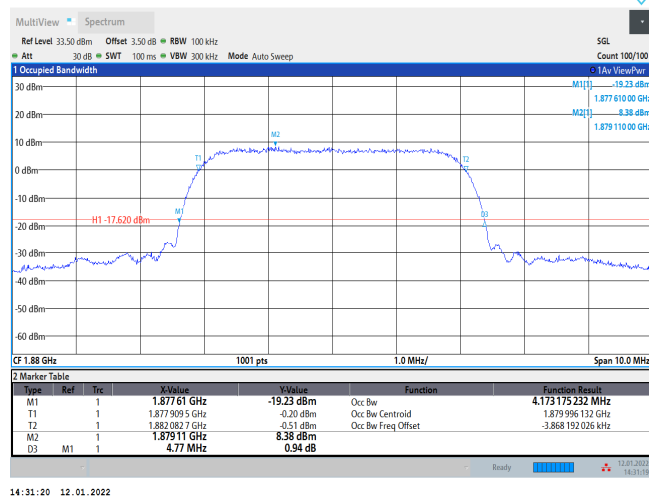
Band2-9400-4.77
