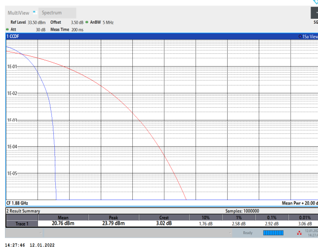
Band2-9400
