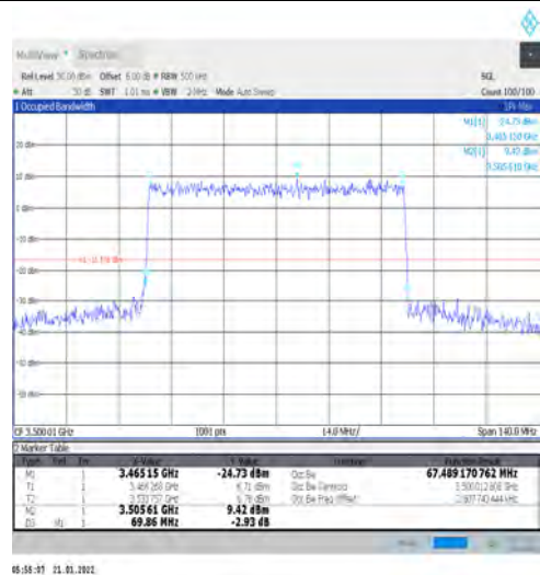
1-N78-3450-3550-PC2-30-70-M-9-CP-256QAM-Outer_Full-Outer_Full@N/A-Ant1-67.489-69.860-≤70-PASS
