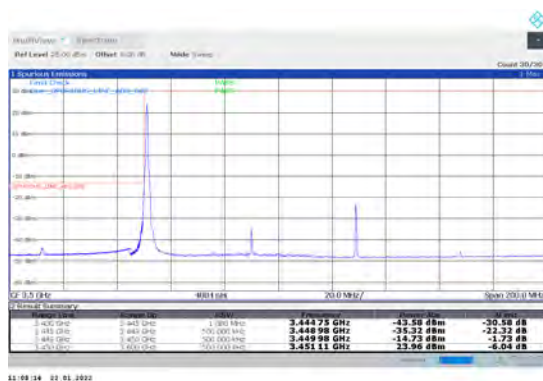
1-N78-3450-3550-PC2-30-80-L-4-CP-QPSK-Edge_1R
