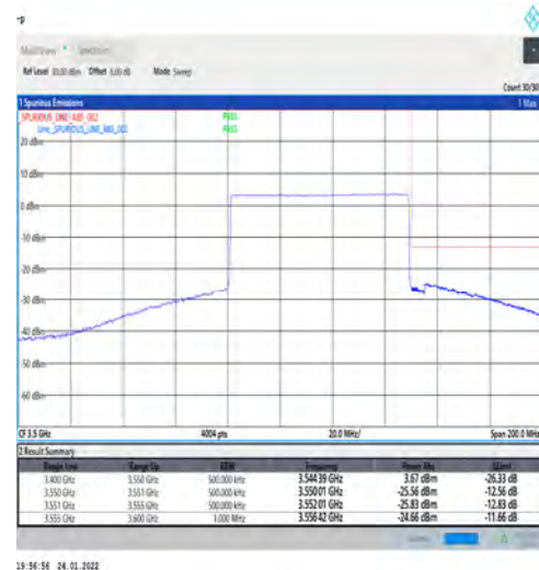
1-N78-3450-3550-PC2-30-70-H-6-CP-QPSK-Outer _Full-189@0-Ant1-PASS-see graph
