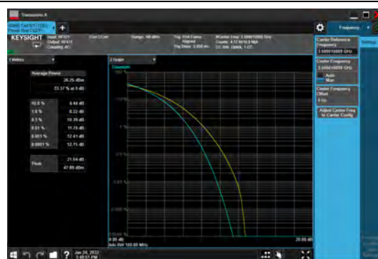
1-N78-3450-3550-PC2-30-100-M-6-CP-QPSK-Out er_Full
