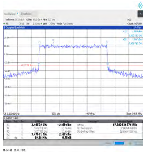
1-N78-3450-3550-PC2-30-70-M-7-CP-16QAM-Outer_Full-Outer_Full@N/A-Ant1-67.381-69.580-≤70-PASS
