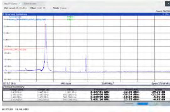
1-N78-3450-3550-PC2-30-50-L-1-DFT-PI2BPSK-Edge_1RB_Left-1@0-Ant1-PASS-see graph
