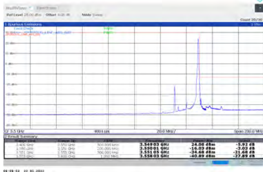
1-N78-3450-3550-PC2-30-20-H-5-CP-QPSK-Edge_1R B Right-1@50-Ant1-PASS-see graph
