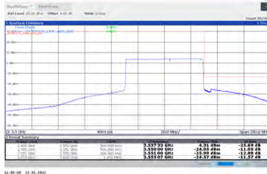
1-N78-3450-3550-PC2-30-60-H-6-CP-QPSK-Outer Full-162@0-Ant1-PASS-see graph
