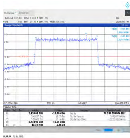
1-N78-3450-3550-PC2-30-80-M-4-DFT-64QAM-Out er_Full-216@0-Ant1-77.182-80.320-≤80-PASS
