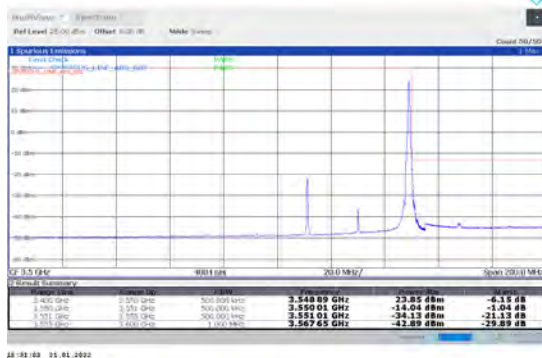
1-N78-3450-3550-PC2-30-40-H-2-DFT-PI2BPSK-Edge_1RB_Right-1@105-Ant1-PASS-see graph
