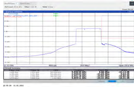
1-N78-3450-3550-PC2-30-40-H-6-CP-QPSK-Outer_Full-106@0-Ant1-PASS-see graph
