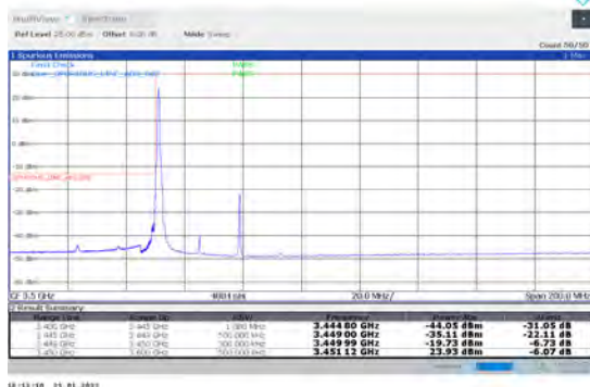
1-N78-3450-3550-PC2-30-30-L-1-DFT-PI2BPSK-Edge 1RB Left-1@0-Ant1-PASS-see graph
