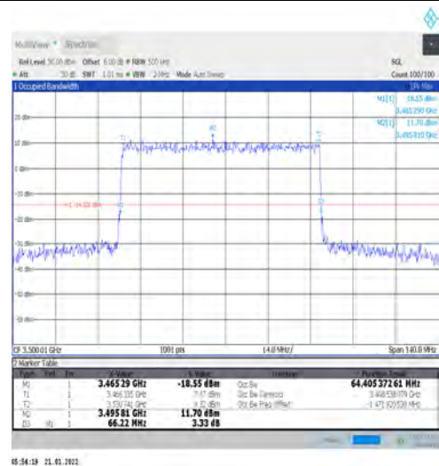
1-N78-3450-3550-PC2-30-70-M-5-DFT-256QAM-Out_Full-Outer_Full@N/A-Ant1-64.405-66.220-≤70-P ASS
