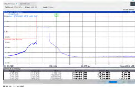
1-N78-3450-3550-PC2-30-20-L-6-CP-QPSK-Outer_Full-51@0-Ant1-PASS-see graph
