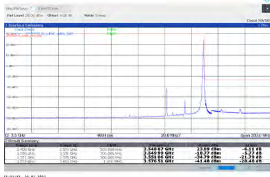
1-N78-3450-3550-PC2-30-30-H-5-CP-QPSK-Edge_1R B Right-1@77-Ant1-PASS-see graph
