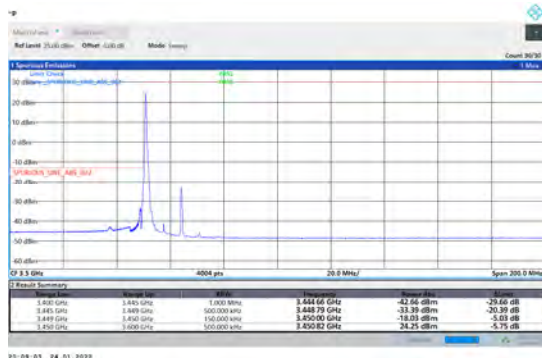
1-N78-3450-3550-PC2-30-15-L-1-DFT-PI2BPSK-Edge_1RB_Left-1@0-Ant1-PASS-see graph
