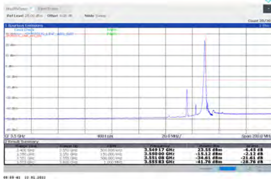
1-N78-3450-3550-PC2-30-15-H-2-DFT-PI2BPSK-Edge _1RB_Right-1@37-Ant1-PASS-see graph
