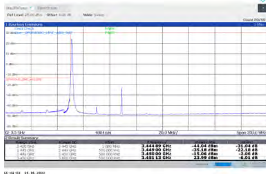
1-N78-3450-3550-PC2-30-40-L-1-DFT-PI2BPSK-Edge 1RB Left-1@0-Ant1-PASS-see graph
