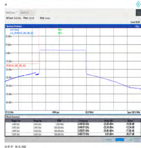
1-N78-3450-3550-PC2-30-70-L-6-CP-QPSK-Outer _Full-189@0-Ant1-PASS-see graph
