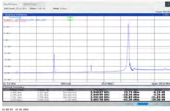
1-N78-3450-3550-PC2-30-90-H-2-DFT-PI2BPSK-Edge_1RB_Right-1@244-Ant1-PASS-see graph
