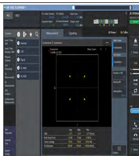
1-N78-3450-3550-PC2-30-100-M-2-DFT-QPSK-Out er_Full-270@0-Ant1-see graph-PASS
