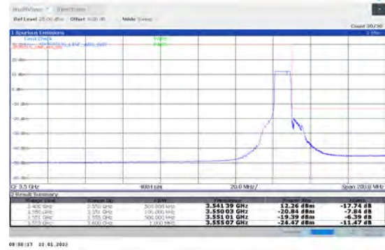
1-N78-3450-3550-PC2-30-10-H-6-CP-QPSK-Outer_Full-24@0-Ant1-PASS-see graph
