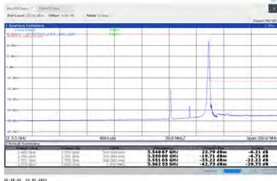
1-N78-3450-3550-PC2-30-30-H-2-DFT-PI2BPSK-Edge 1RB Right-1@77-Ant1-PASS-see graph
