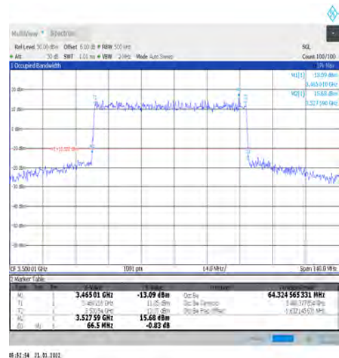
1-N78-3450-3550-PC2-30-70-M-1-DFT-QPSK-Outer_Full-Outer_Full@N/A-Ant1-64.325-66.500-≤70-PASS
