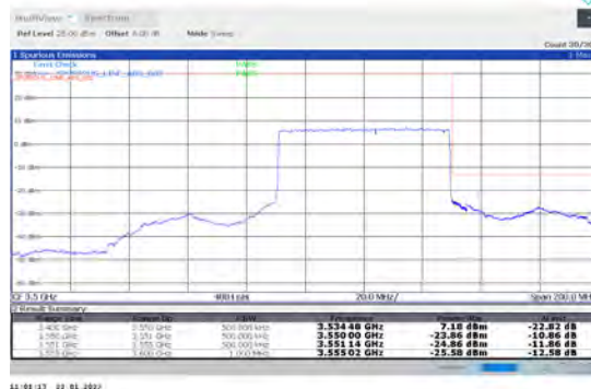
1-N78-3450-3550-PC2-30-60-H-3-DFT-PI2BPSK- Outer Full-162@0-Ant1-PASS-see graph
