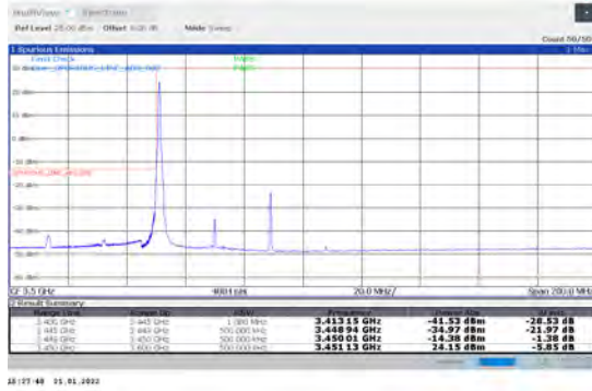
1-N78-3450-3550-PC2-30-40-L-4-CP-QPSK-Edge_1R_B_Left-1@0-Ant1-PASS-see graph
