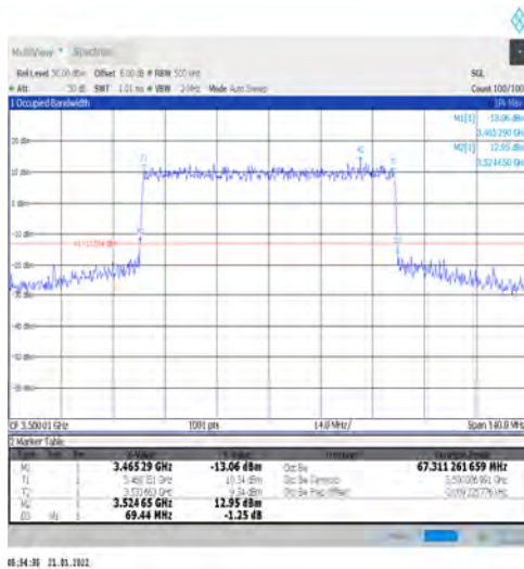
1-N78-3450-3550-PC2-30-70-M-6-CP-QPSK-Outer_Full-Outer_Full@N/A-Ant1-67.311-69.440-≤70-PASS
