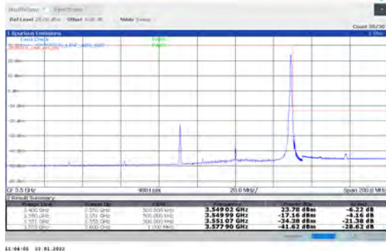
1-N78-3450-3550-PC2-30-60-H-5-CP-QPSK-Edge_1R B Right-1@161-Ant1-PASS-see graph
