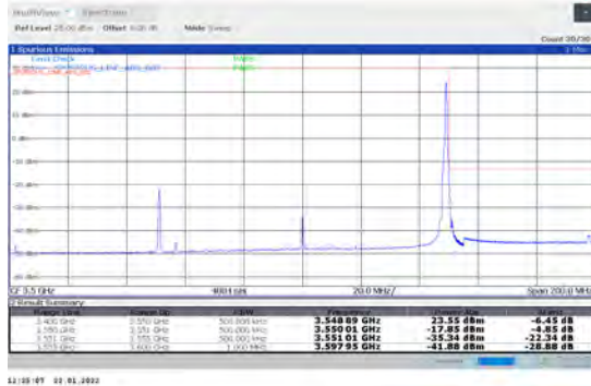
1-N78-3450-3550-PC2-30-100-H-5-CP-QPSK-Edge_1 RB_Right-1@272-Ant1-PASS-see graph
