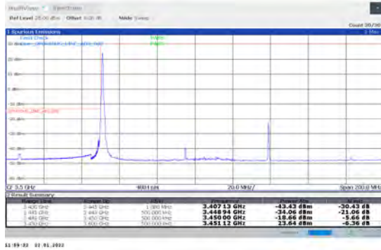
1-N78-3450-3550-PC2-30-90-L-4-CP-QPSK-Edge_1R_B_Left-1@0-Ant1-PASS-see graph
