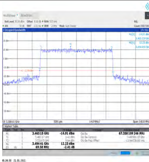
1-N78-3450-3550-PC2-30-70-M-8-CP-64QAM-Outer_Full-Outer_Full@N/A-Ant1-67.358-69.580-≤70-PASS
