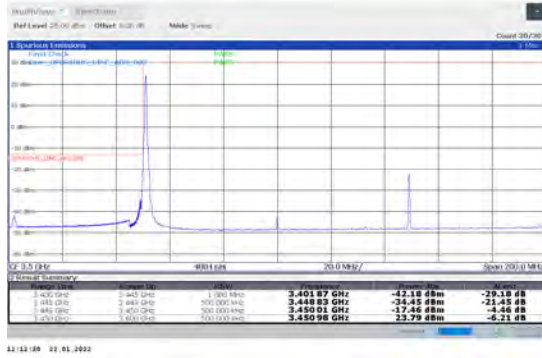
1-N78-3450-3550-PC2-30-100-L-1-DFT-PI2BPSK-Edge_1RB_Left-1@0-Ant1-PASS-see graph
