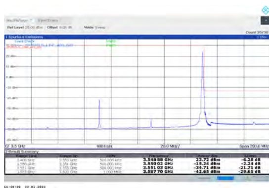
1-N78-3450-3550-PC2-30-80-H-2-DFT-PI2BPSK-Edge 1RB Right-1@216-Ant1-PASS-see graph
