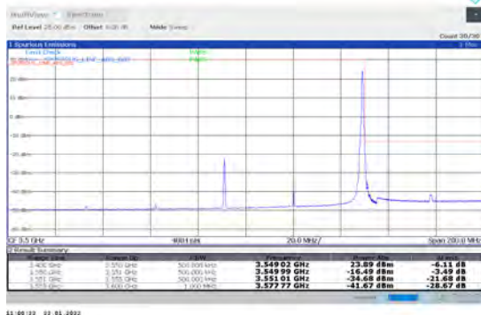
1-N78-3450-3550-PC2-30-60-H-2-DFT-PI2BPSK-Edge 1RB Right-1@161-Ant1-PASS-see graph
