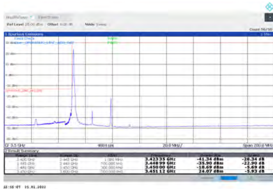
1-N78-3450-3550-PC2-30-30-L-4-CP-QPSK-Edge_1R B Left-1@0-Ant1-PASS-see graph
