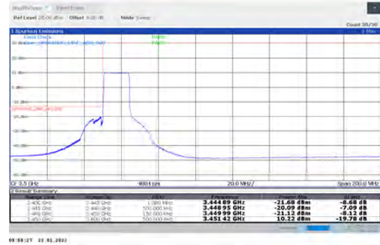
1-N78-3450-3550-PC2-30-15-L-6-CP-QPSK-Outer _Full-38@0-Ant1-PASS-see graph
