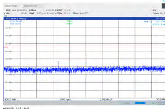
1-N78-3450-3550-PC3-30-100-M-1-DFT-PI2BPSK-E dge_1RB_Left-1@0-0.15-30
