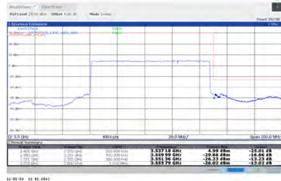
1-N78-3450-3550-PC2-30-90-H-2-DFT-PI2BPSK-Outer_Full-245@0-Ant1-PASS-see graph
