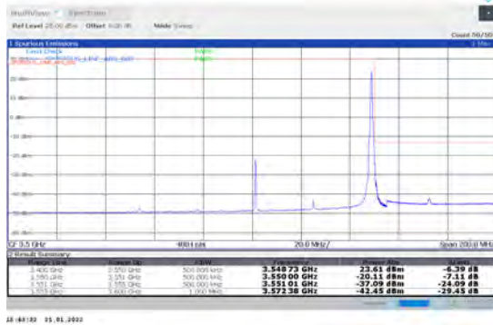
1-N78-3450-3550-PC2-30-50-H-2-DFT-PI2BPSK-Edge_1RB_Right-1@132-Ant1-PASS-see graph
