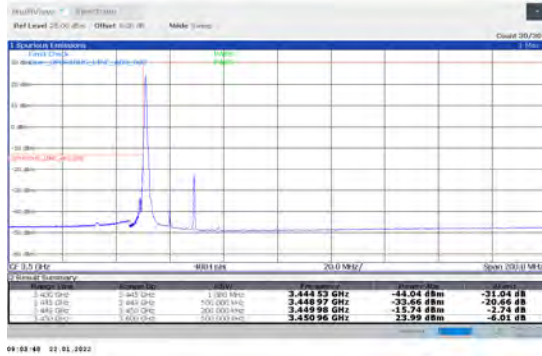
1-N78-3450-3550-PC2-30-20-L-1-DFT-PI2BPSK-Edge_1RB_Left-1@0-Ant1-PASS-see graph
