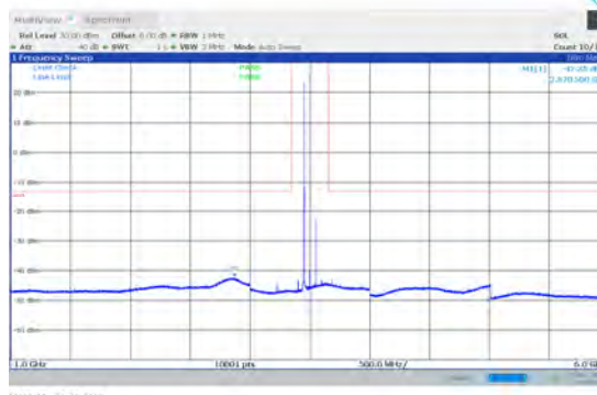
1-N78-3450-3550-PC3-30-100-M-1-DFT-PI2BPSK-E dge_1RB_Left-1@0-1000-6000
