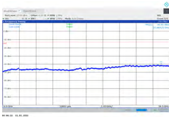
1-N78-3450-3550-PC3-30-100-M-1-DFT-PI2BPSK-E dge_1RB_Left-1@0-6000-26500
