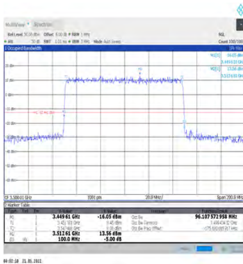
1-N78-3450-3550-PC2-30-100-M-5-DFT-256QAM-Out uter_Full-270@0-Ant1-96.108-100.000-≤100-PASS
