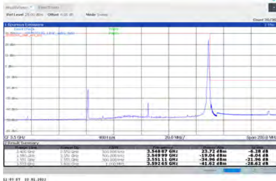
1-N78-3450-3550-PC2-30-90-H-6-CP-QPSK-Edge_1RB_Right-1@244-Ant1-PASS-see graph
