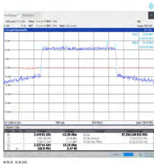
1-N78-3450-3550-PC2-30-100-M-6-CP-QPSK-Outer _Full-273@0-Ant1-97.346-100.800-≤100-PASS
