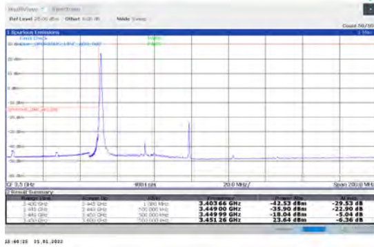
1-N78-3450-3550-PC2-30-50-L-4-CP-QPSK-Edge_1RB_Left-1@0-Ant1-PASS-see graph
