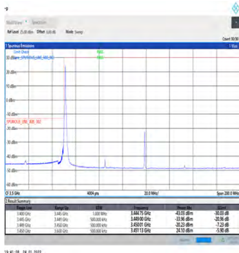
1-N78-3450-3550-PC2-30-70-L-1-DFT-PI2BPSK-Edge
