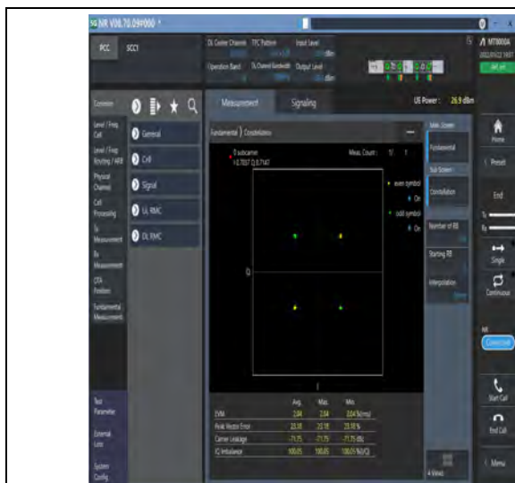
1-N78-3450-3550-PC2-30-100-M-1-DFT-PI2BPSK-Out uter_Full-270@0-Ant1-see graph-PASS
