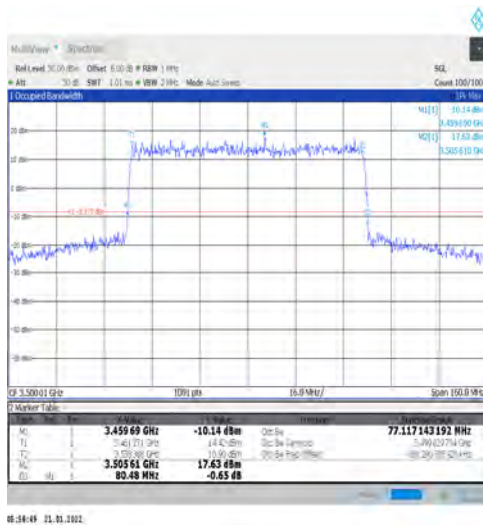
1-N78-3450-3550-PC2-30-80-M-3-DFT-16QAM-Oute r_Full-216@0-Ant1-77.117-80.480-≤80-PASS
