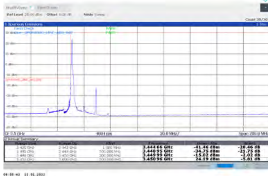
1-N78-3450-3550-PC2-30-20-L-4-CP-QPSK-Edge_1RB_Left-1@0-Ant1-PASS-see graph
