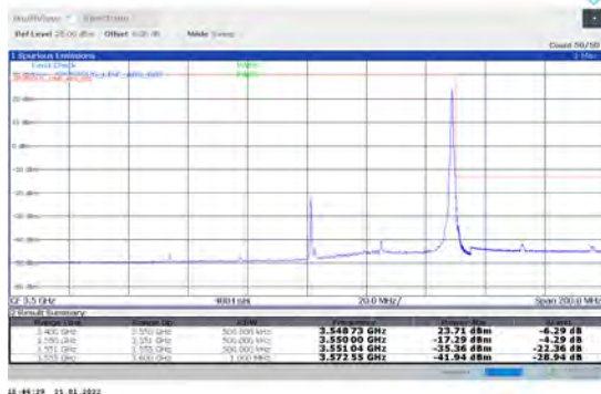
1-N78-3450-3550-PC2-30-50-H-5-CP-QPSK-Edge_1R B Right-1@132-Ant1-PASS-see graph
