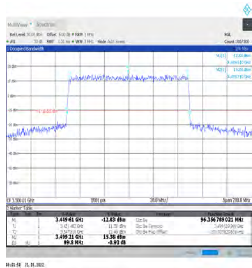
1-N78-3450-3550-PC2-30-100-M-4-DFT-64QAM-Out er_Full-270@0-Ant1-96.357-99.800-≤100-PASS
