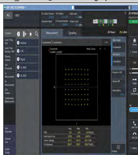
1-N78-3450-3550-PC2-30-100-M-4-DFT-64QAM-Out er_Full-270@0-Ant1-see graph-PASS
