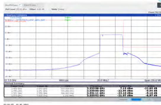
1-N78-3450-3550-PC2-30-30-H-6-CP-QPSK-Outer Full-78@0-Ant1-PASS-see graph
