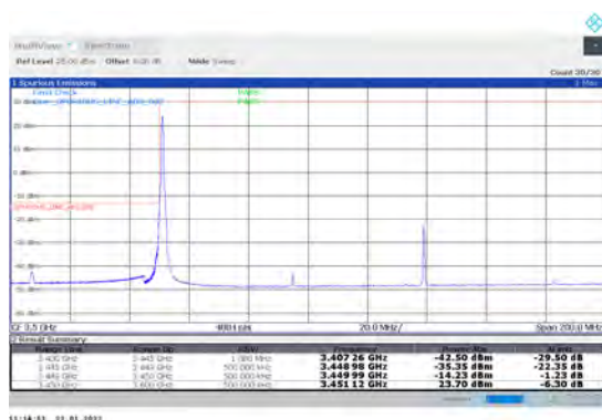
1-N78-3450-3550-PC2-30-90-L-1-DFT-PI2BPSK-Edge 1RB Left-1@0-Ant1-PASS-see graph
