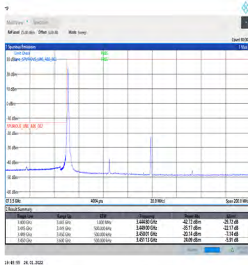
1-N78-3450-3550-PC2-30-70-L-4-CP-QPSK-Edge_1R B_Left-1@0-Ant1-PASS-see graph
