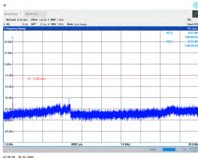
Band2-20MHz-256QAM-19100-1RB#0-Range4:1000~20000MHz
