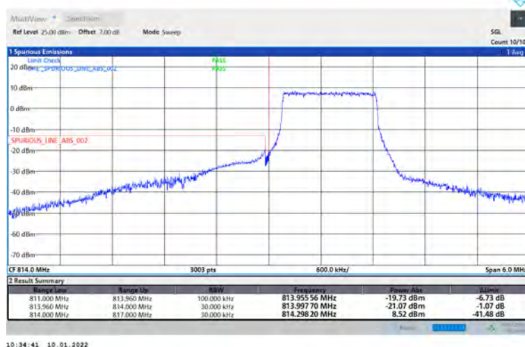
Band26-1.4MHz-QPSK-26697-6RB#0
