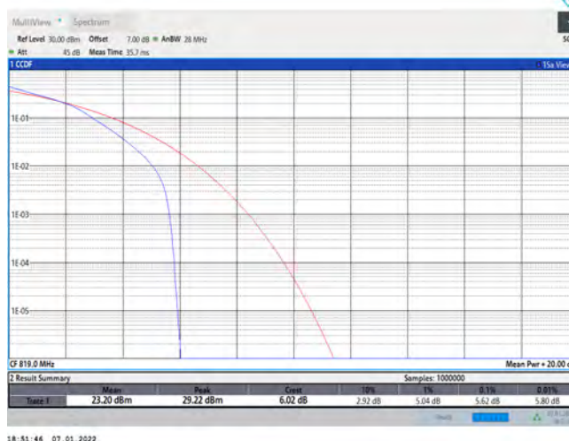
Band26-10MHz-16QAM-26740-50RB#0
