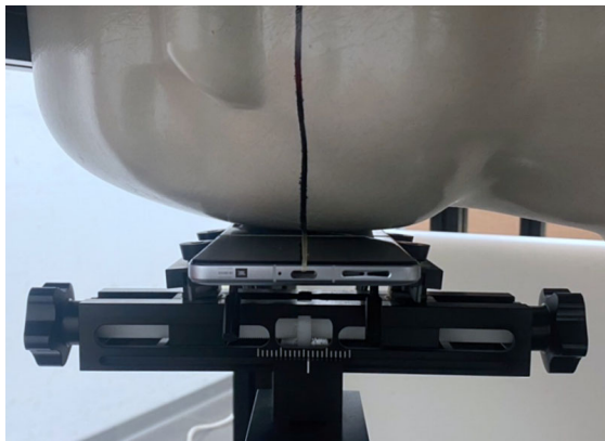
Photograph 1. Head, Right Touch, 0mm
