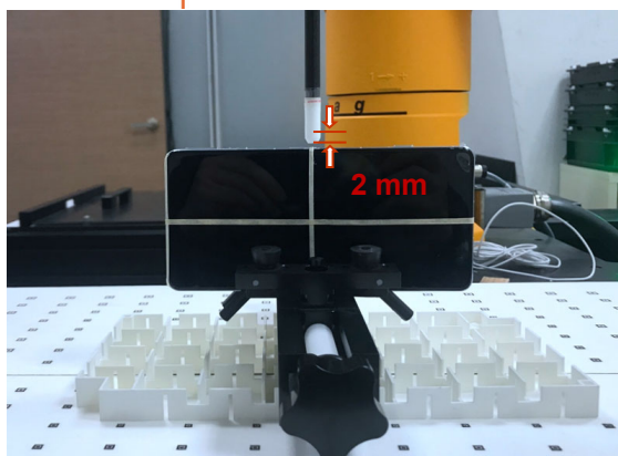
Photograph 25. PD, Right Edge, 2mm
