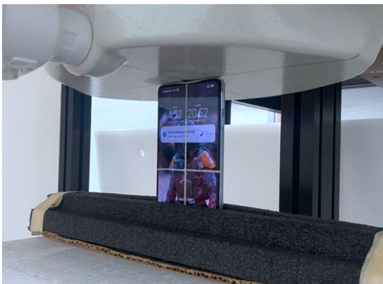
Photograph 17. Product specific 10-g SAR, Top Edge, 0mm
