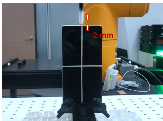
Photograph 27. PD, Top Edge, 2mm
