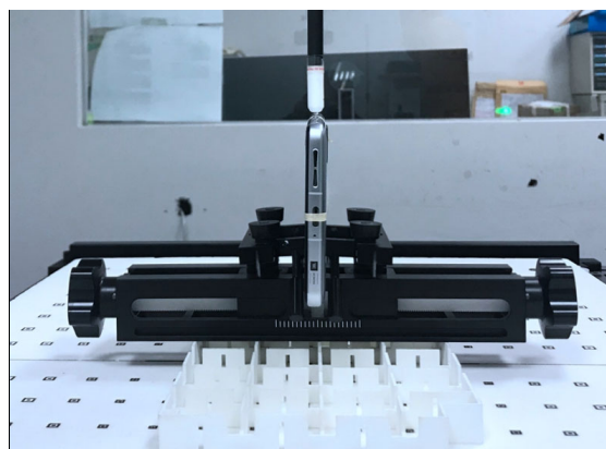
Photograph 26. PD, Right Edge, 2mm
