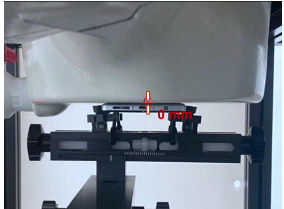
Photograph 16. Product specific 10-g SAR, Back Surface, 0mm
