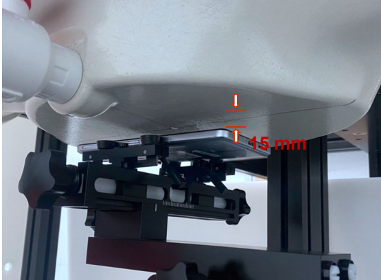
Photograph 9. Body-worn, Front Surface, 15mm
