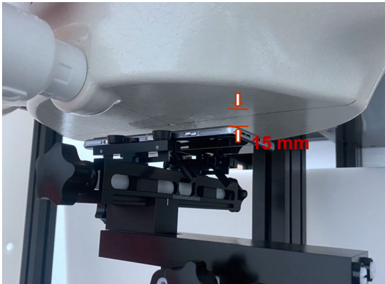
Photograph 11. Body-worn, Back Surface, 15mm
