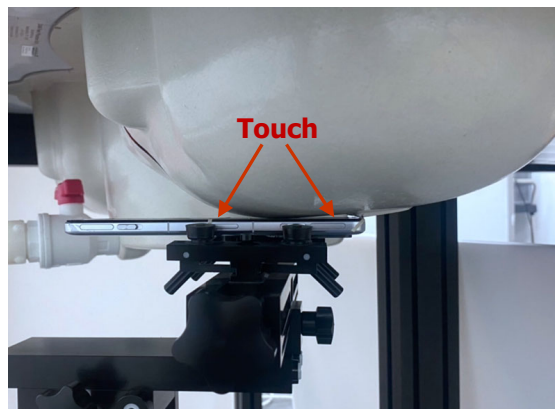
Photograph 6. Head, Left Touch, 0mm
