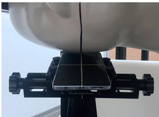
Photograph 3. Head, Right Tilt, 0mm
