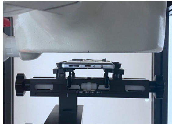
Photograph 12. Body-worn, Back Surface, 15mm
