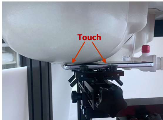
Photograph 2. Head, Right Touch, 0mm
