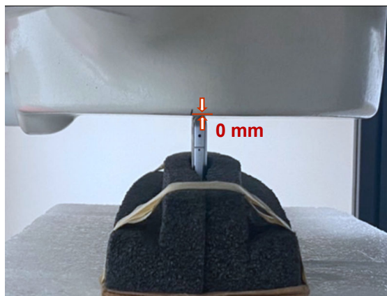
Photograph 24. Product specific 10-g SAR, Left Edge, 0mm
