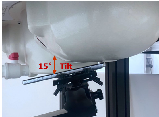
Photograph 8. Head, Left Tilt, 0mm
