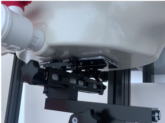
Photograph 15. Product specific 10-g SAR, Back Surface, 0mm
