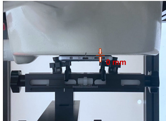
Photograph 14. Product specific 10-g SAR, Front Surface, 0mm
