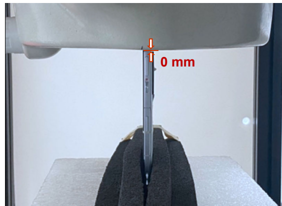
Photograph 18. Product specific 10-g SAR, Top Edge, 0mm
