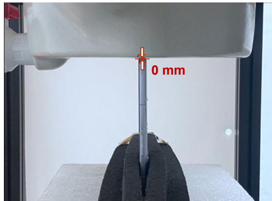
Photograph 20. Product specific 10-g SAR, Bottom Edge, 0mm
