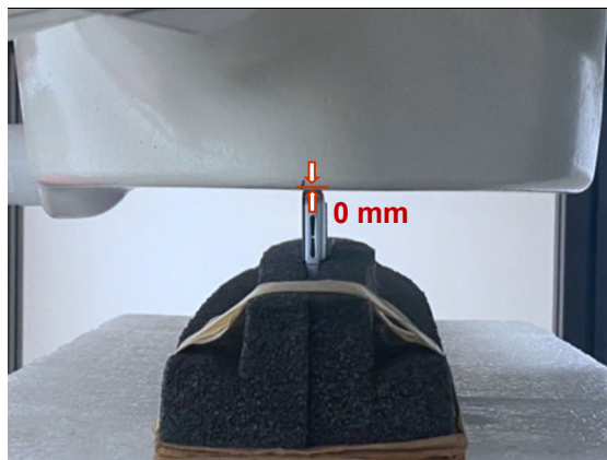
Photograph 22. Product specific 10-g SAR, Right Edge, 0mm
