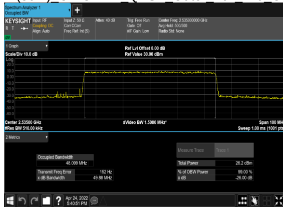
N7(50M)_CP-OFDM_64QAM_Outer_Full_Mid_CH
