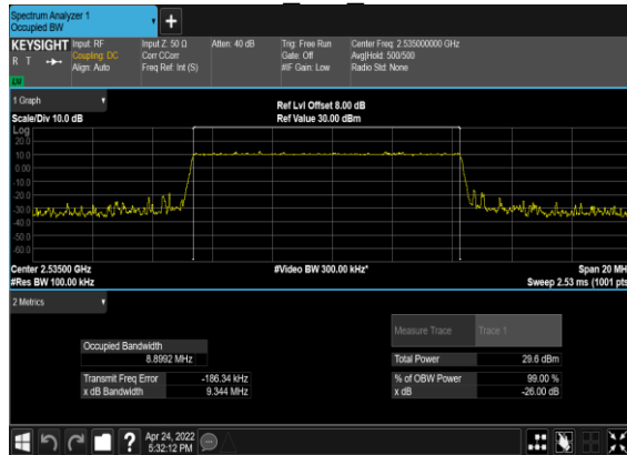
N7(10M)_CP-OFDM_QPSK_Outer_Full_Mid_CH
