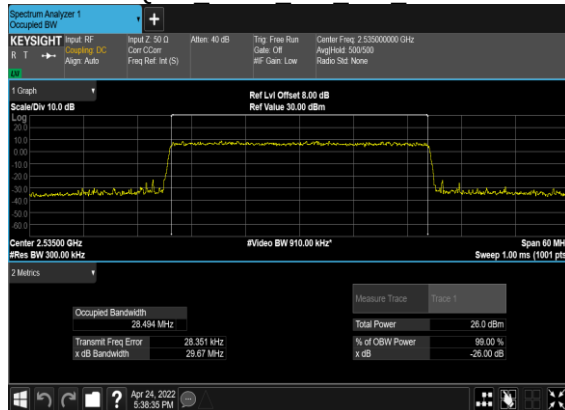
N7(30M)_CP-OFDM_64QAM_Outer_Full_Mid_CH
