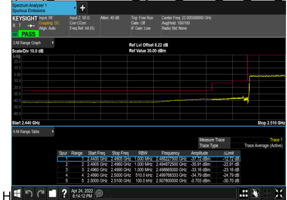
N7(25M)_DFT-s-OFDM_QPSK_Outer_Full_Low_CH
