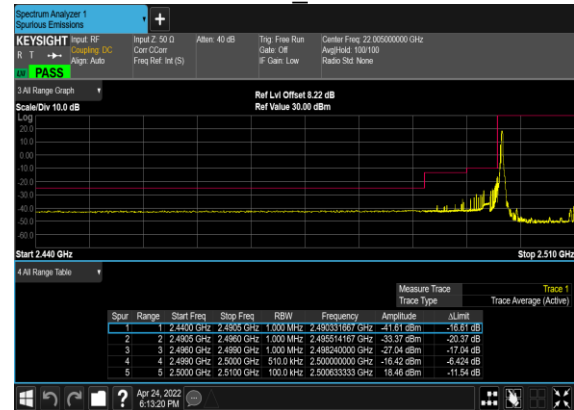
N7(25M)_DFT-s-OFDM_QPSK_Outer_Full_Low_CH
