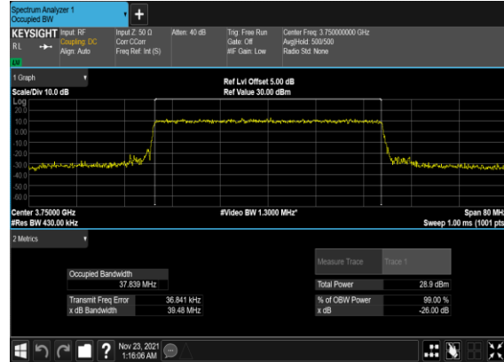
N78(40M)_CP-OFDM_64 QAM_Outer_Full_Mid_CH
