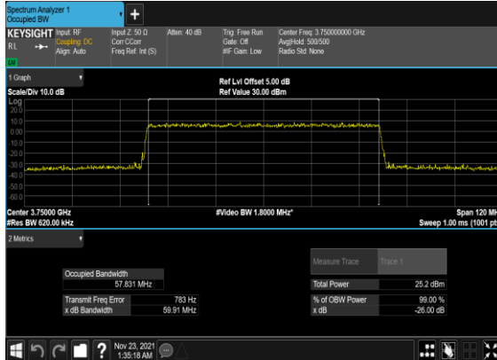
N78(60M)_CP-OFDM_256 QAM_Outer_Full_Mid_CH
