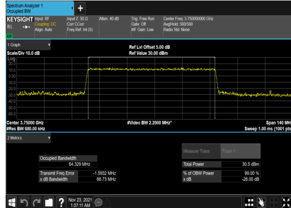
N78(70M)_DFT-s- OFDM_QPSK_Outer_Full_Mid_CH
