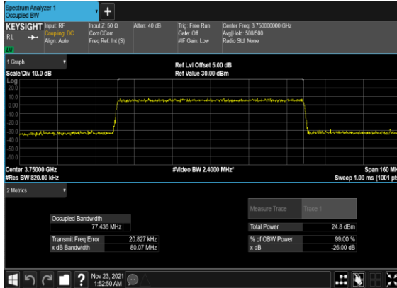
N78(80M)_CP-OFDM_256 QAM_Outer_Full_Mid_CH
