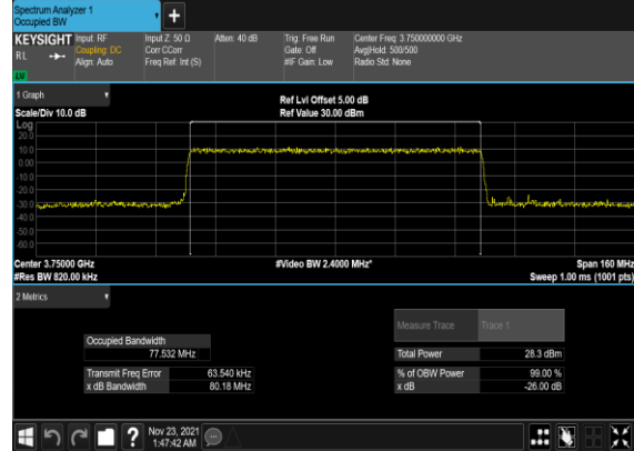
N78(80M)_CP- OFDM_QPSK_Outer_Full_Mid_CH
