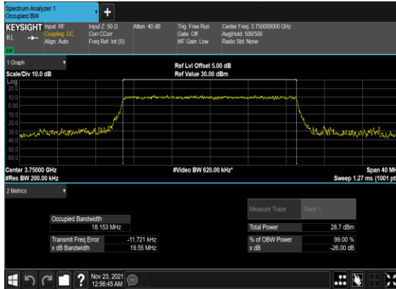
N78(20M)_CP-OFDM_16 QAM_Outer_Full_Mid_CH
