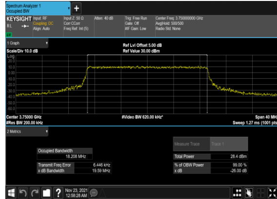
N78(20M)_CP-OFDM_64 QAM_Outer_Full_Mid_CH
