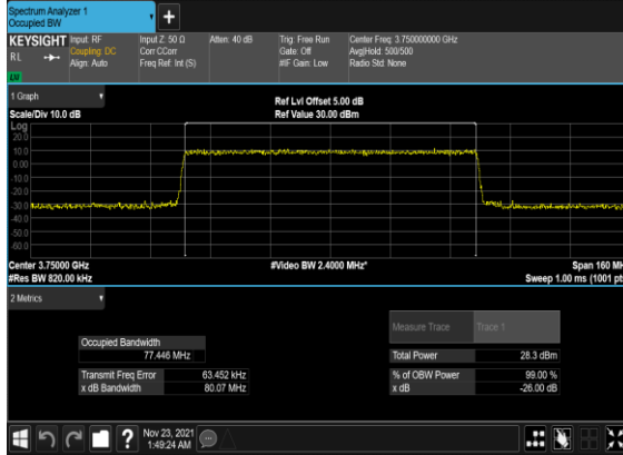
N78(80M)_CP-OFDM_16 QAM_Outer_Full_Mid_CH
