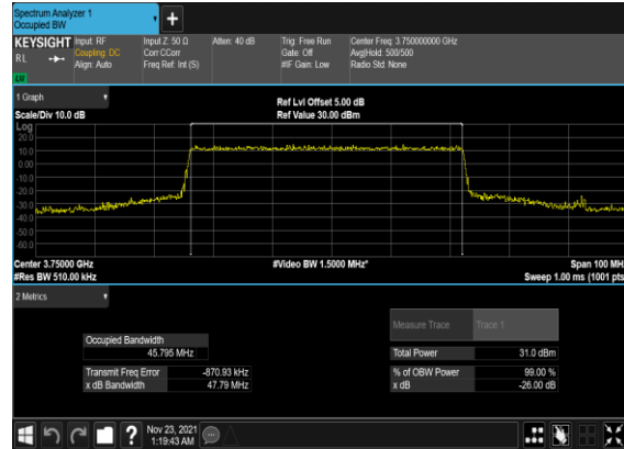
N78(50M)_DFT-s- OFDM_QPSK_Outer_Full_Mid_CH
