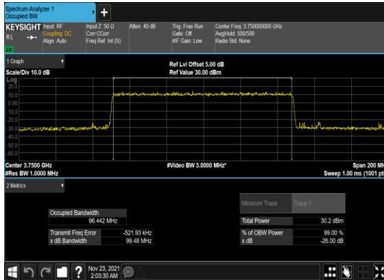
N78(100M)_DFT-s- OFDM_QPSK_Outer_Full_Mid_CH
