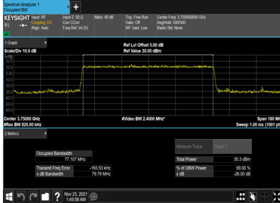
N78(80M)_DFT-s- OFDM_QPSK_Outer_Full_Mid_CH
