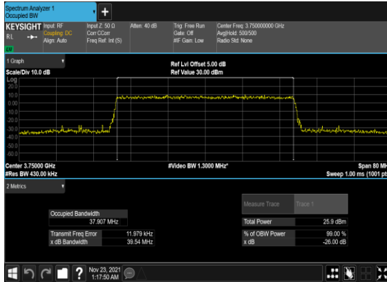
N78(40M)_CP-OFDM_256 QAM_Outer_Full_Mid_CH
