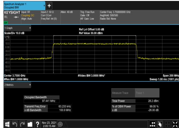
N78(100M)_CP- OFDM_QPSK_Outer_Full_Mid_CH
