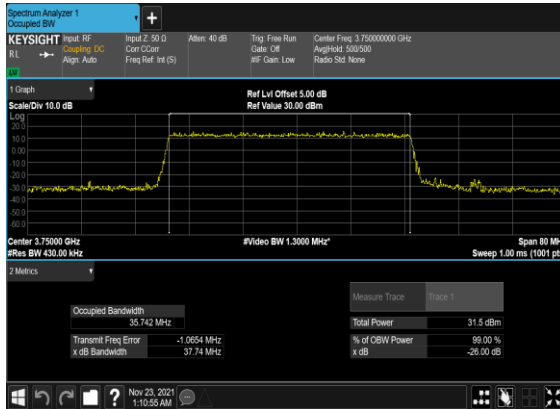
N78(40M)_DFT-s- OFDM_QPSK_Outer_Full_Mid_CH
