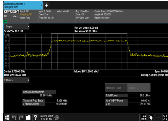
N78(40M)_CP- OFDM_QPSK_Outer_Full_Mid_CH
