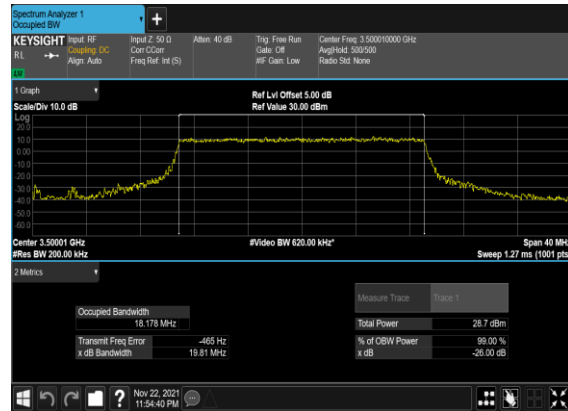
N78(20M)_CP- OFDM_QPSK_Outer_Full_Mid_CH
