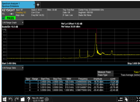
N78(20M)_DFT-s- OFDM_QPSK_Edge_1RB_Right_High_CH
