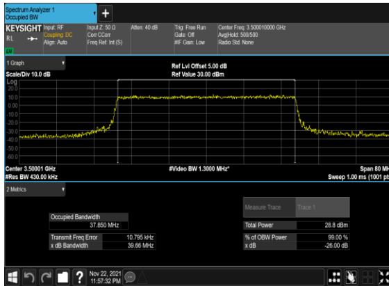
N78(40M)_CP-OFDM_16 QAM_Outer_Full_Mid_CH
