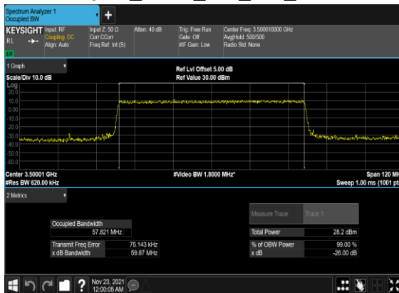
N78(60M)_CP-OFDM_16 QAM_Outer_Full_Mid_CH
