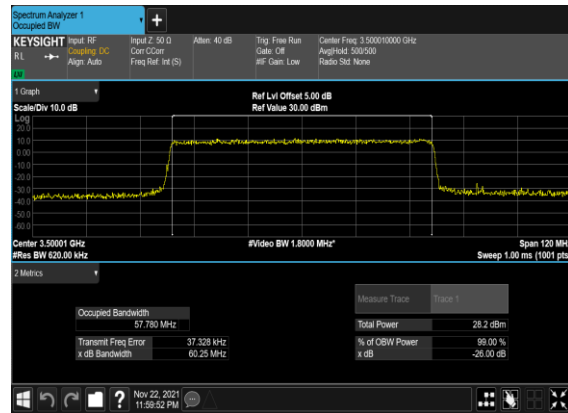
N78(60M)_CP- OFDM_QPSK_Outer_Full_Mid_CH
