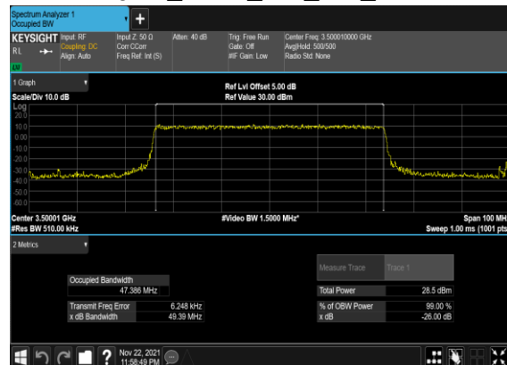
N78(50M)_CP-OFDM_16 QAM_Outer_Full_Mid_CH
