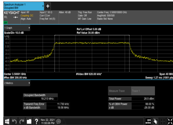
N78(20M)_CP-OFDM_64 QAM_Outer_Full_Mid_CH
