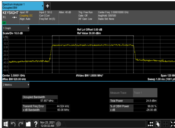
N78(60M)_CP-OFDM_256 QAM_Outer_Full_Mid_CH
