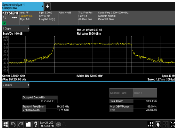
N78(20M)_CP-OFDM_16 QAM_Outer_Full_Mid_CH
