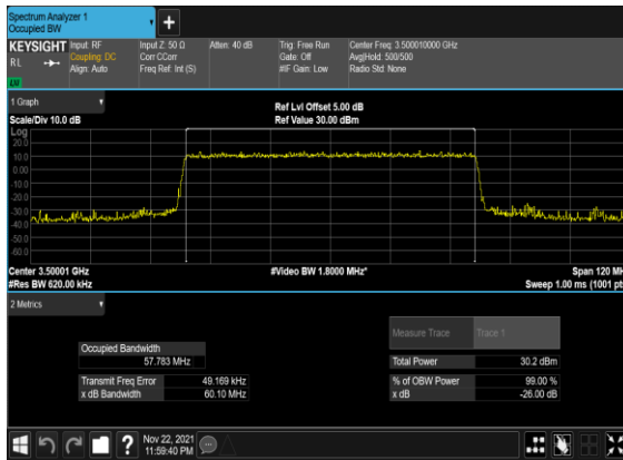
N78(60M)_DFT-s- OFDM_QPSK_Outer_Full_Mid_CH
