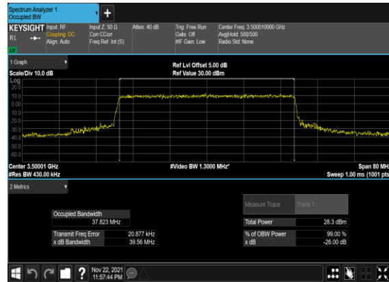
N78(40M)_CP-OFDM_64 QAM_Outer_Full_Mid_CH
