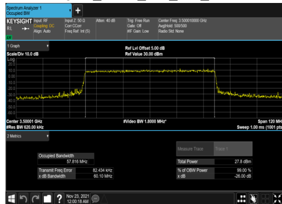
N78(60M)_CP-OFDM_64 QAM_Outer_Full_Mid_CH
