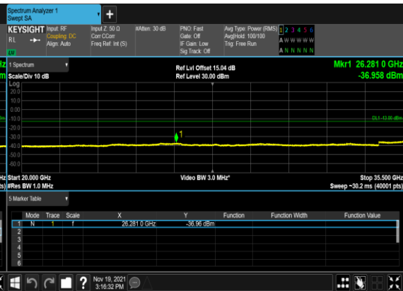
N78(20M)_CP- OFDM_QPSK_Edge_1RB_Left_Low_C H
