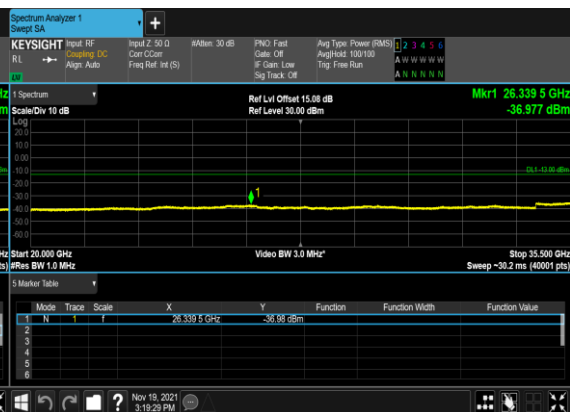
N78(20M)_CP- OFDM_QPSK_Edge_1RB_Left_High_C H
