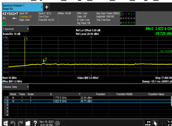
B5_N66(5M)_DFT-s-OFDM_QPSK_Edge_1RB_Left_High_CH
