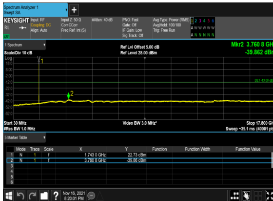
B5_N66(5M)_DFT-s-OFDM_QPSK_Edge_1RB_Left_Mid_CH
