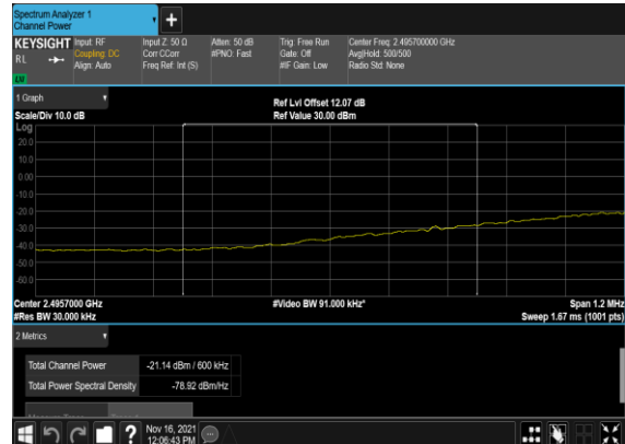
N41(60M)_DFT-s- OFDM_QPSK_Edge_1RB_Left_Low_CH_chp _PASS
