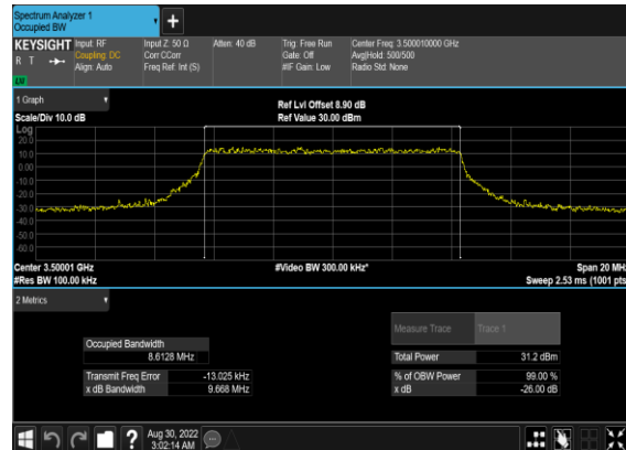
N78(10M)_DFT-s- OFDM_QPSK_Outer_Full_Mid_CH
