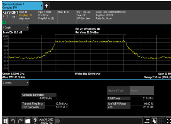
N78(10M)_DFT-s-OFDM_PI_2- BPSK_Outer_Full_Mid_CH
