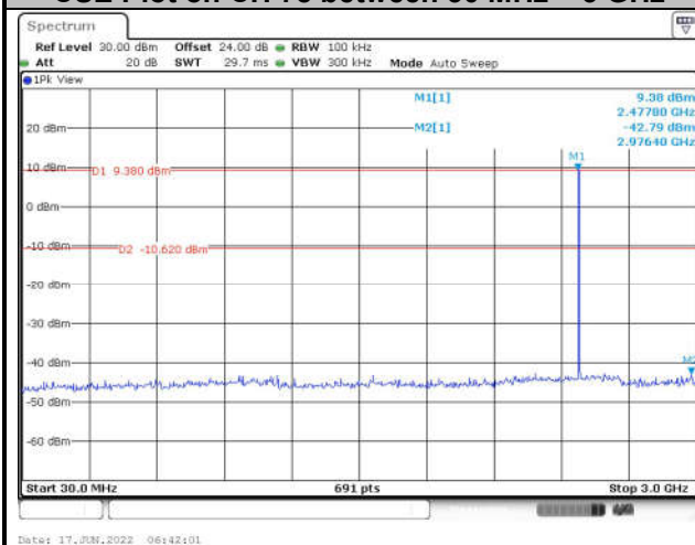
CSE Plot on CH 78 between 30 MHz ~ 3 GHz
