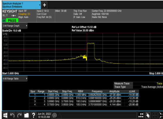
N77(10M)_DFT-s- OFDM_BPSK_Outer_Full_Low_CH
