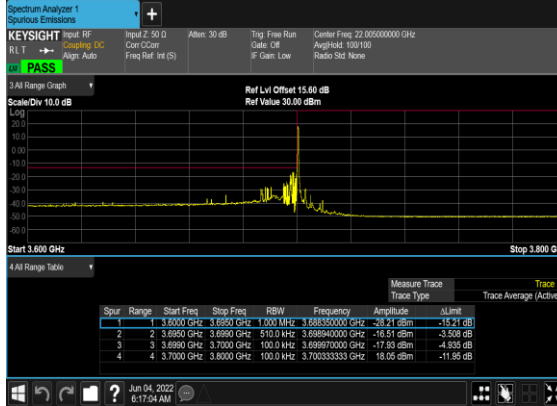
N77(10M)_DFT-s- OFDM_BPSK_Edge_1RB_Left_Low_CH
