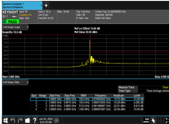
N77(10M)_DFT-s- OFDM_BPSK_Edge_1RB_Right_High_CH
