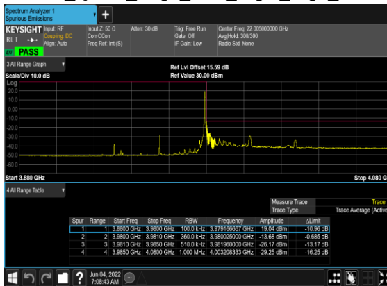
N77(50M)_DFT-s- OFDM_QPSK_Edge_1RB_Right_High_CH
