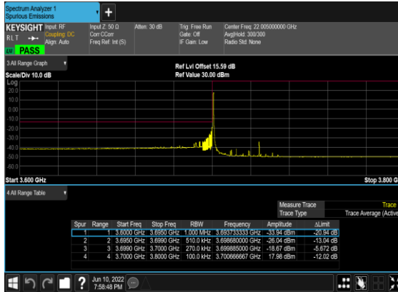
N77(25M)_DFT-s- OFDM_BPSK_Edge_1RB_Left_Low_CH
