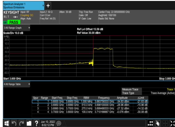
N77(25M)_DFT-s- OFDM_QPSK_Outer_Full_Low_CH
