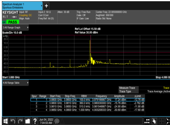
N77(50M)_DFT-s- OFDM_BPSK_Edge_1RB_Right_High_CH
