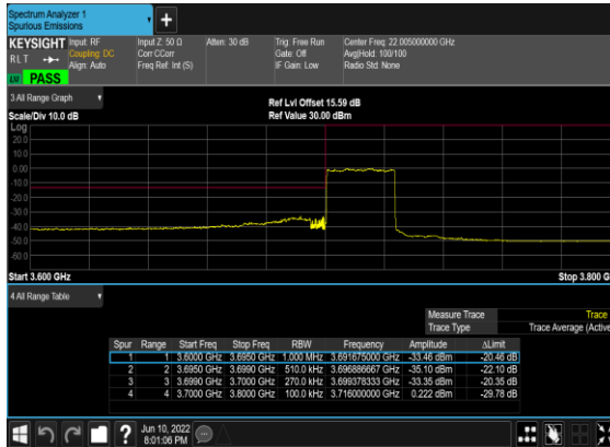
N77(25M)_DFT-s- OFDM_BPSK_Outer_Full_Low_CH
