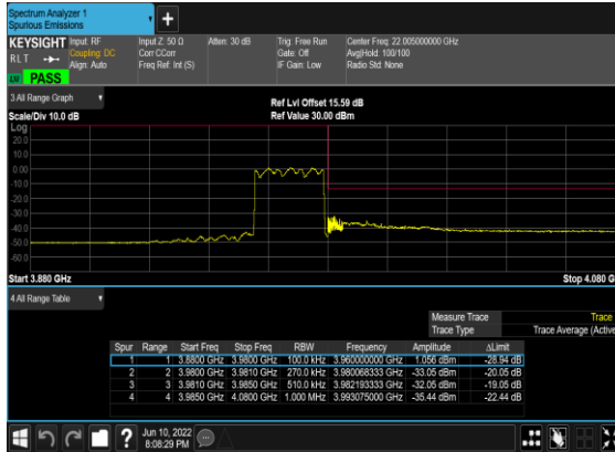
N77(25M)_DFT-s- OFDM_BPSK_Outer_Full_High_CH
