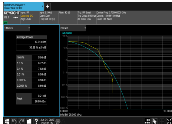
N78(20M)_DFT-s-OFDM_PI_2-BPSK_Edge_1RB_Left_Mid_CH
