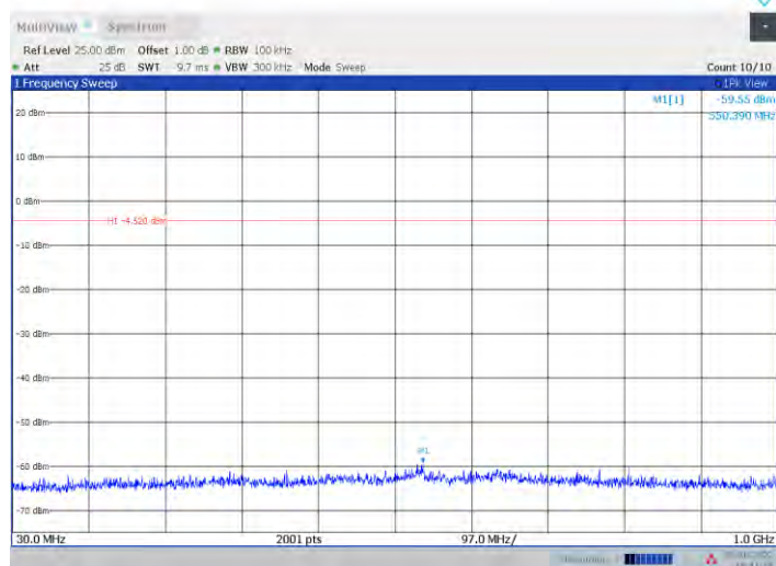
DH5_Ant7_2402_30~1000
