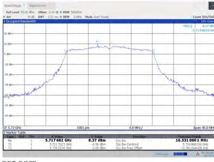
11a-CDD Ant8 5720
