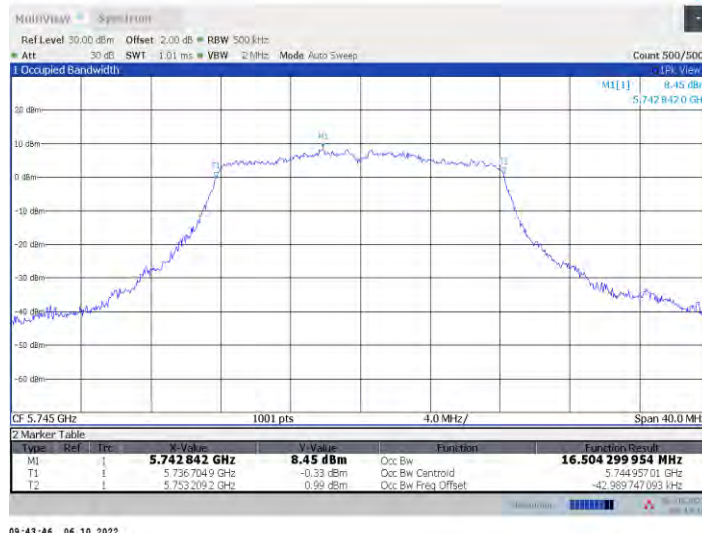
11a-CDD Ant8 5745
