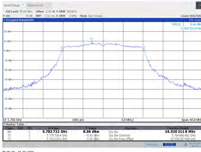
11a-CDD Ant8 5785
