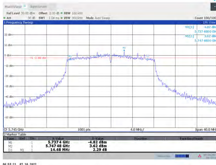
11a-CDD Ant8 5745
