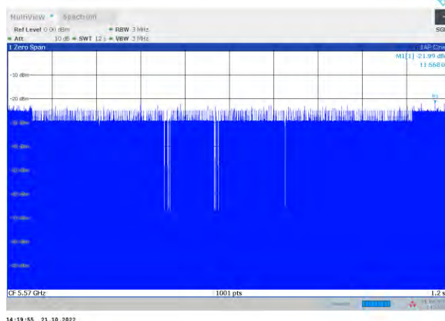
Master—11ax160MIMO_5570
