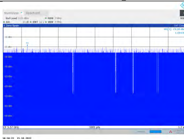
Master—11ax160MIMO_5570
