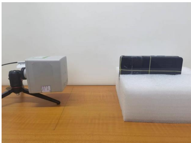
Position E, test separation 15cm
