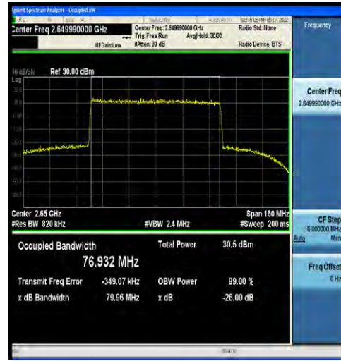
1-N41-30-80-H-5-DFT-256QAM-Outer_Full-216@0-A Ant2-76.932-79.96-<80-PASS
