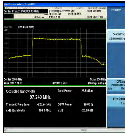
1-N41-30-100-H-9-CP-256QAM-Outer_Full-273@0-A Ant2-97.240-100.6-≤100-PASS
