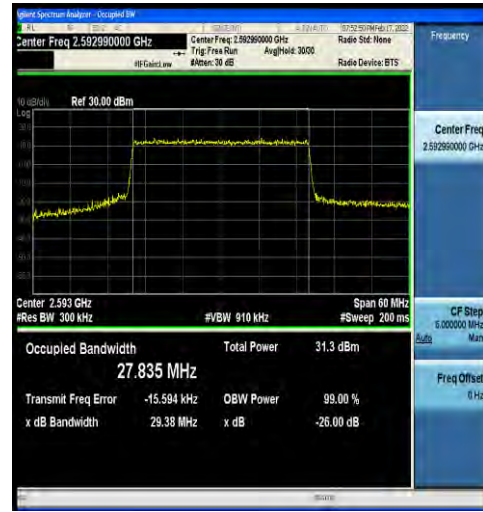
1-N41-30-30-M-6-CP-QPSK-Outer_Full-78@0-Ant2- 27.835-29.38-≤30-PASS
