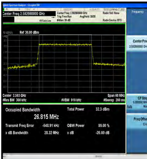
1-N41-30-30-M-3-DFT-16QAM-Outer_Full-75@0-Ant 2-26.815-28.32-≤30-PASS
