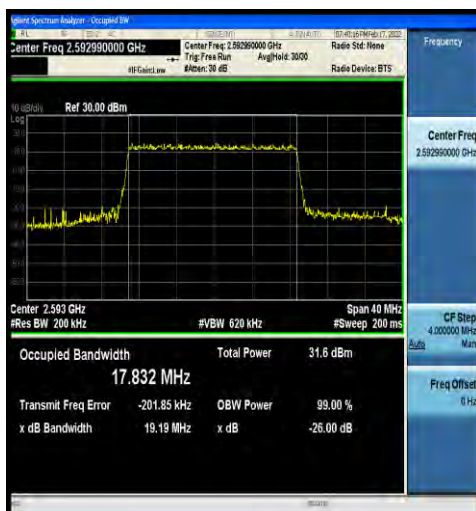
1-N41-30-20-M-4-DFT-64QAM-Outer_Full-50@0-Ant 2-17.832-19.19-≤20-PASS
