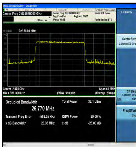
1-N41-30-30-H-4-DFT-64QAM-Outer_Full-75@0-Ant 2-26.770-28.35-≤30-PASS
