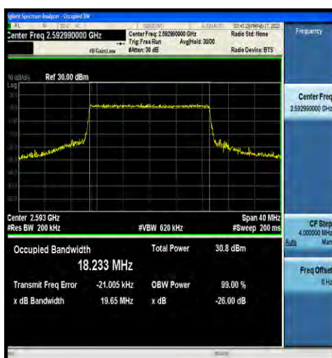
1-N41-30-20-M-6-CP-QPSK-Outer_Full-51@0-Ant2- 18.233-19.65-≤20-PASS
