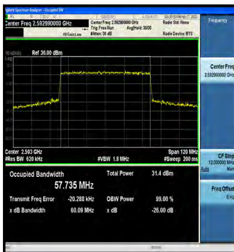
1-N41-30-60-M-8-CP-64QAM-Outer_Full-162@0-An t2-57.735-60.09-≤60-PASS
