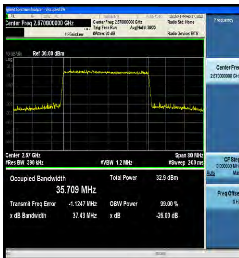
1-N41-30-40-H-3-DFT-16QAM-Outer_Full-100@0-A nt2-35.709-37.43-≤40-PASS
