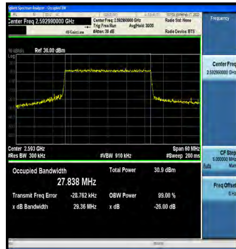
1-N41-30-30-M-8-CP-64QAM-Outer_Full-78@0-Ant2 -27.838-29.36-≤30-PASS
