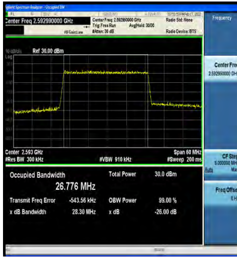
1-N41-30-30-M-5-DFT-256QAM-Outer_Full-75@0-A nt2-26.776-28.30-≤30-PASS
