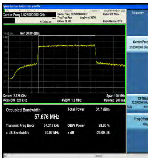
1-N41-30-60-L-7-CP-16QAM-Outer_Full-162@0-Ant 2-57.676-60.07-≤60-PASS
