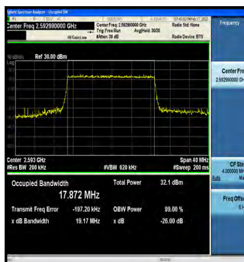
1-N41-30-20-M-3-DFT-16QAM-Outer_Full-50@0-Ant 2-17.872-19.17-≤20-PASS
