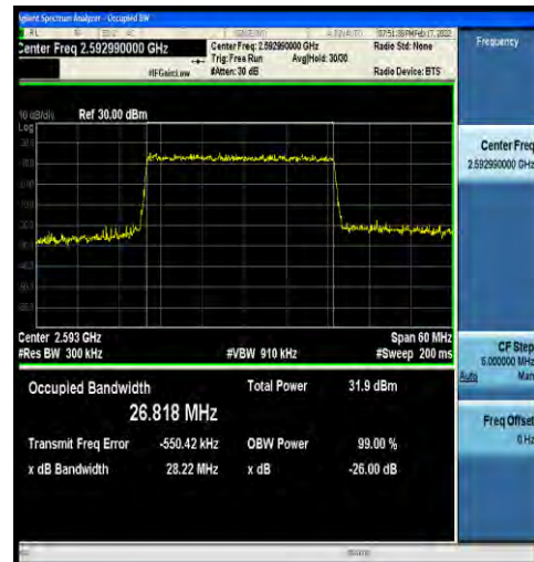
1-N41-30-30-M-4-DFT-64QAM-Outer_Full-75@0-Ant 2-26.818-28.22-≤30-PASS
