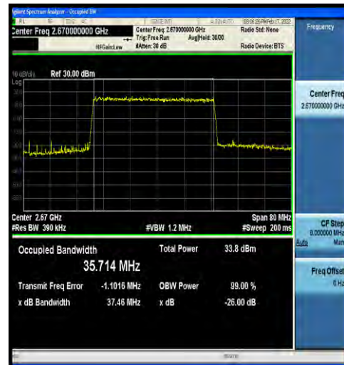
1-N41-30-40-H-2-DFT-PI2BPSK-Outer_Full-100@0-Ant2 35.714-37.46-≤40-PASS
