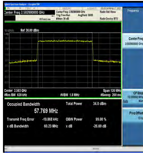
1-N41-30-60-M-1-DFT-QPSK-Outer_Full-162@0-Ant 2-57.769-60.23-≤60-PASS
