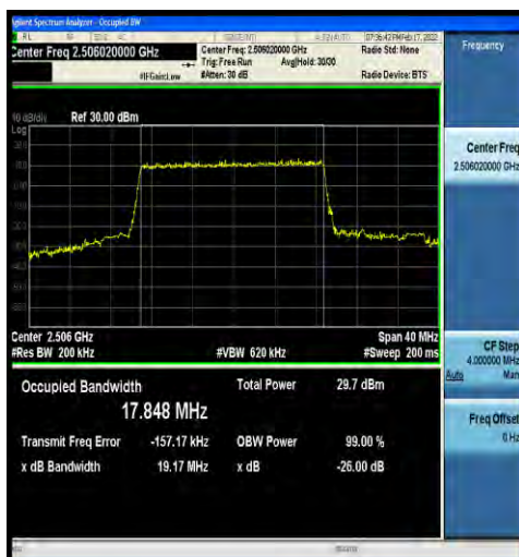
1-N41-30-20-L-5-DFT-256QAM-Outer_Full-50@0-Ant t2-17.848-19.17-≤20-PASS
