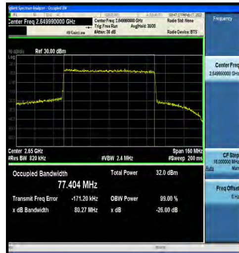
1-N41-30-80-H-7-CP-16QAM-Outer_Full-217@0-Ant 2-77.404-80.27-<80-PASS
