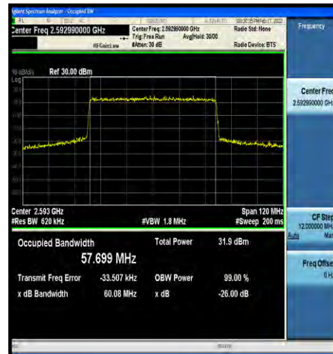
1-N41-30-60-M-7-CP-16QAM-Outer_Full-162@0-Ant 2-57.699-60.08-<60-PASS
