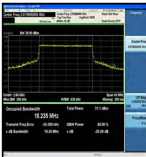
1-N41-30-20-H-7-CP-16QAM-Outer_Full-51@0-Ant2 -18.235-19.56-≤20-PASS
