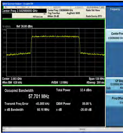
1-N41-30-60-M-4-DFT-64QAM-Outer_Full-162@0-A nt2-57.701-60.16-<60-PASS
