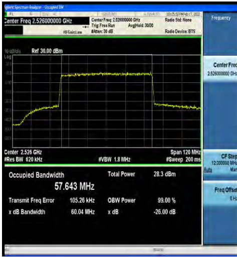
1-N41-30-60-L-9-CP-256QAM-Outer_Full-162@0-A nt2-57.643-60.04-≤60-PASS
