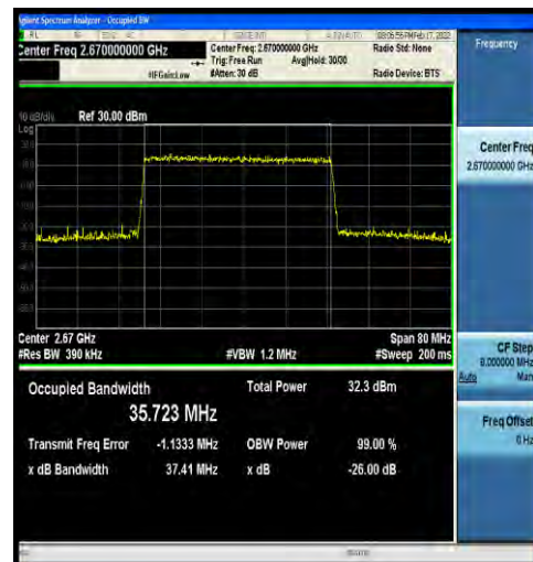
1-N41-30-40-H-4-DFT-64QAM-Outer_Full-100@0-A nt2-35.723-37.41-≤40-PASS
