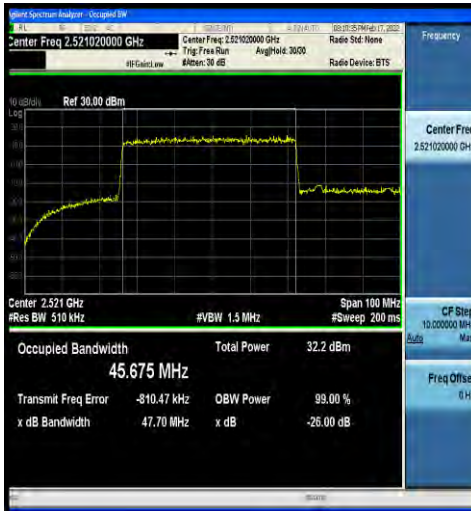
1-N41-30-50-L-4-DFT-64QAM-Outer_Full-128@0-An t2-45.675-47.70-≤50-PASS
