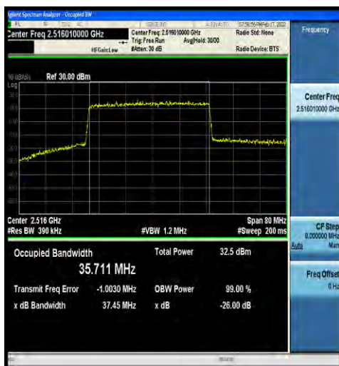
1-N41-30-40-L-3-DFT-16QAM-Outer_Full-100@0-An t2-35.711-37.45-≤40-PASS
