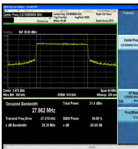
1-N41-30-30-H-6-CP-QPSK-Outer_Full-78@0-Ant2- 27.862-29.30-≤30-PASS
