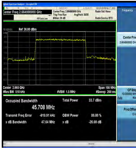
1-N41-30-50-H-2-DFT-PI2BPSK-Outer_Full-128@0-Ant2-45.708-47.64-≤50-PASS
