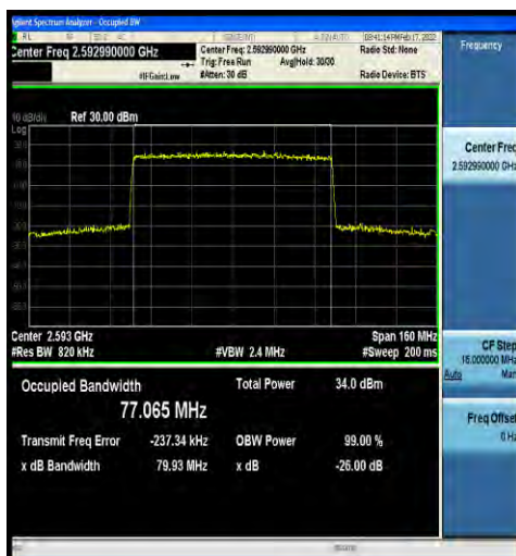
1-N41-30-80-M-1-DFT-QPSK-Outer_Full-216@0-Ant 2-77.065-79.93-≤80-PASS
