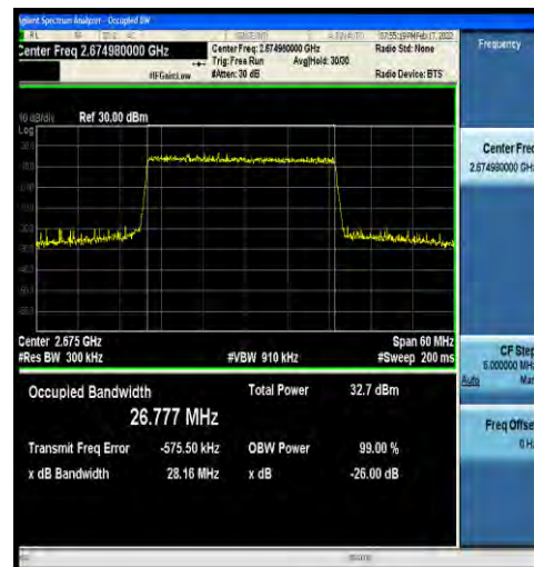
1-N41-30-30-H-3-DFT-16QAM-Outer_Full-75@0-Ant 2-26.777-28.16-≤30-PASS
