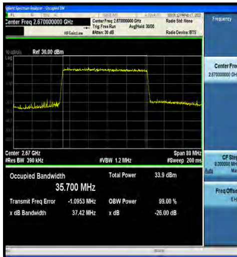
1-N41-30-40-H-1-DFT-QPSK-Outer_Full-100@0-Ant 2-35.700-37.42-≤40-PASS
