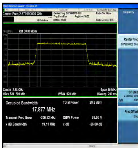
1-N41-30-20-H-5-DFT-256QAM-Outer_Full-50@0-Ant nt2-17.877-19.11-≤20-PASS
