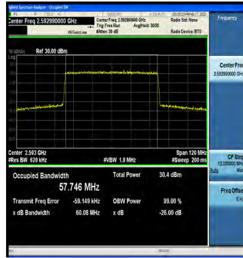
1-N41-30-60-M-5-DFT-256QAM-Outer_Full-162@0-A Ant2-57.746-60.08-<60-PASS
