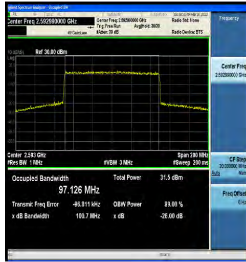
1-N41-30-100-M-8-CP-64QAM-Outer_Full-273@0-A nt2-97.126-100.7-≤100-PASS
