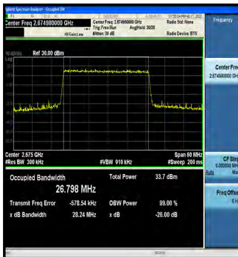
1-N41-30-30-H-2-DFT-PI2BPSK-Outer_Full-75@0-A nt2-26.798-28.24-≤30-PASS
