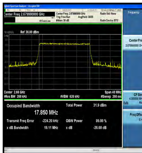
1-N41-30-20-H-4-DFT-64QAM-Outer_Full-50@0-Ant 2-17.850-19.11-≤20-PASS
