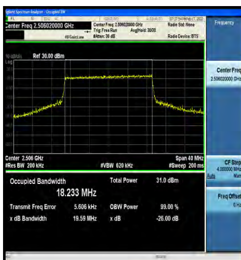
1-N41-30-20-L-7-CP-16QAM-Outer_Full-51@0-Ant2 -18.233-19.59-≤20-PASS
