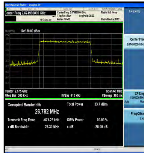
1-N41-30-30-H-1-DFT-QPSK-Outer_Full-75@0-Ant2 -26.782-28.30-≤30-PASS
