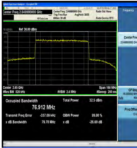
1-N41-30-80-H-4-DFT-64QAM-Outer_Full-216@0-A nt2-76.912-79.78-<80-PASS
