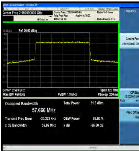
1-N41-30-60-M-6-CP-QPSK-Outer_Full-162@0-Ant2 -57.666-59.99-<60-PASS
