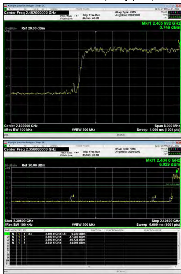
BT 3DH5 CH0, Carrier frequency (MHz): 2402
