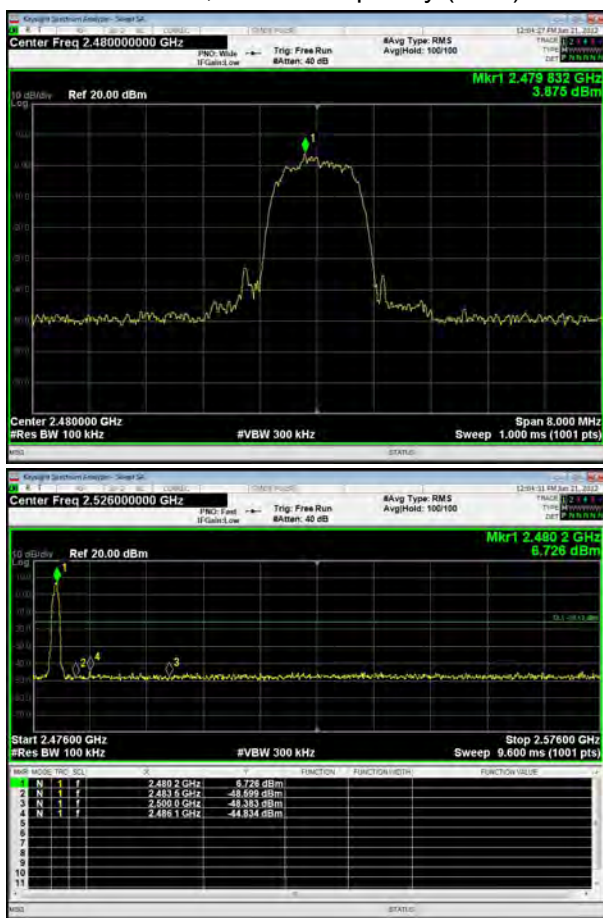
BT 3DH5 CH78, Carrier frequency (MHz): 2480
