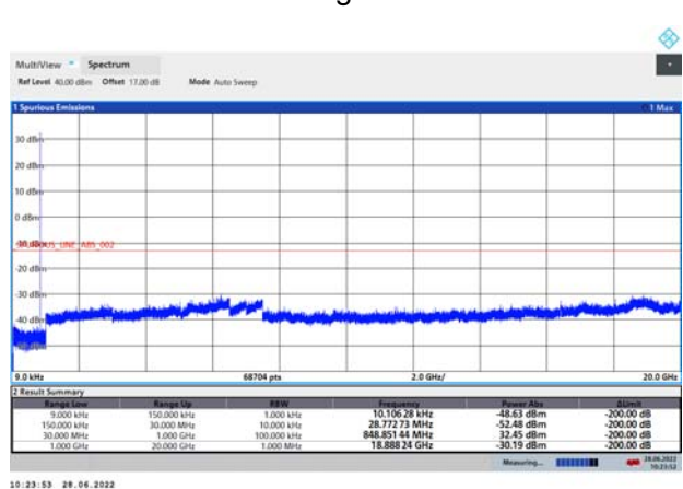
GSM 850 CH-High 9kHz ~ 20GHz
