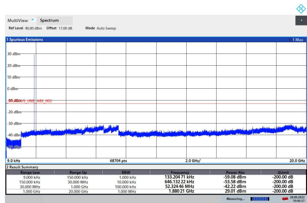
GPRS 1900 CH- Middle 9kHz ~ 20GHz
