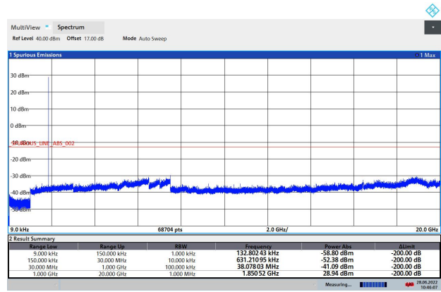
GPRS 1900 CH-Low 9kHz ~ 20GHz
