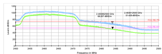
802.11n HT20 -Channel 11 Peak+ Average
