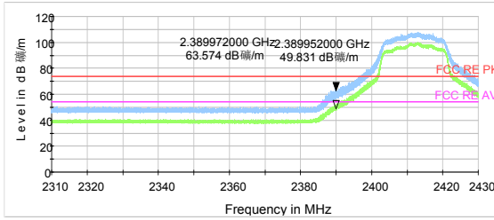
802.11b-Channel 1 Peak+ Average
