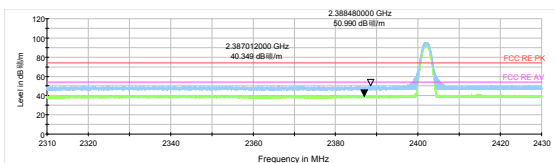
Bluetooth LE Channel 0 Peak+ Average
