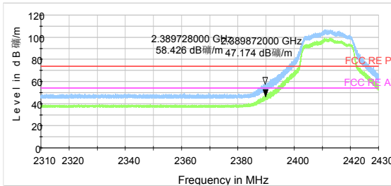
802.11n HT20 -Channel 1 Peak+ Average
