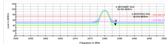
Bluetooth LE Channel 39 Peak+Average
