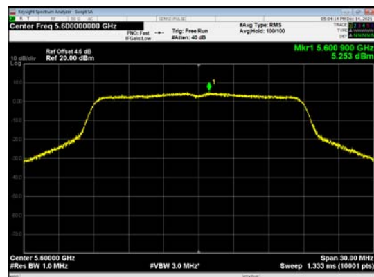
U-NII-2C, 802.11ac VHT20, Channel No.: 120
