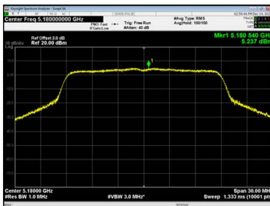
U-NII-1, 802.11ac VHT20, Channel No.: 36
