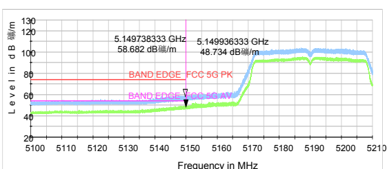
802.11n HT40-Channel 38: Peak + Average
