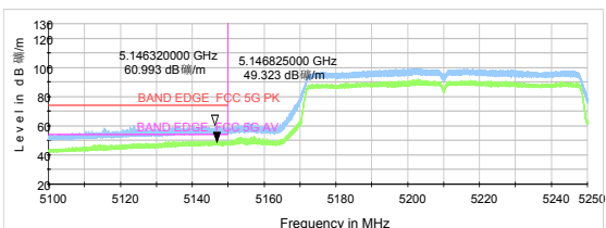
802.11ac VHT80 -Channel 42: Peak + Average
