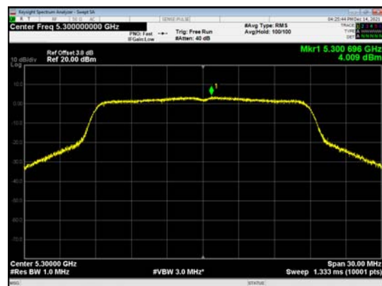
U-NII-2A, 802.11ac VHT20, Channel No.: 60
