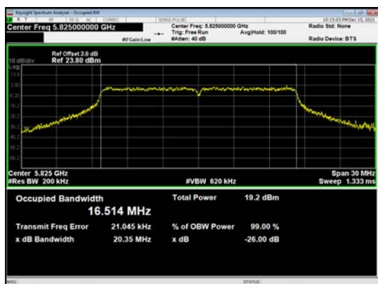
U-NII-3, 802.11a Carrier frequency (MHz): 5825
