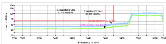
802.11n HT40-Channel 102: Peak + Average
