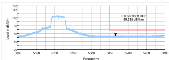
802.11n HT40-Channel 142: Peak
