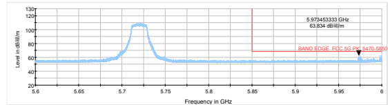
802.11n HT20-Channel 144: Peak
