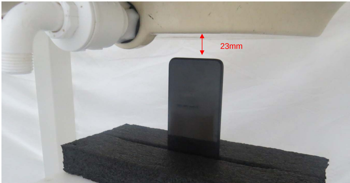
Picture 19: Bottom Edge, the distance from handset to the bottom of the Phantom is 23mm
