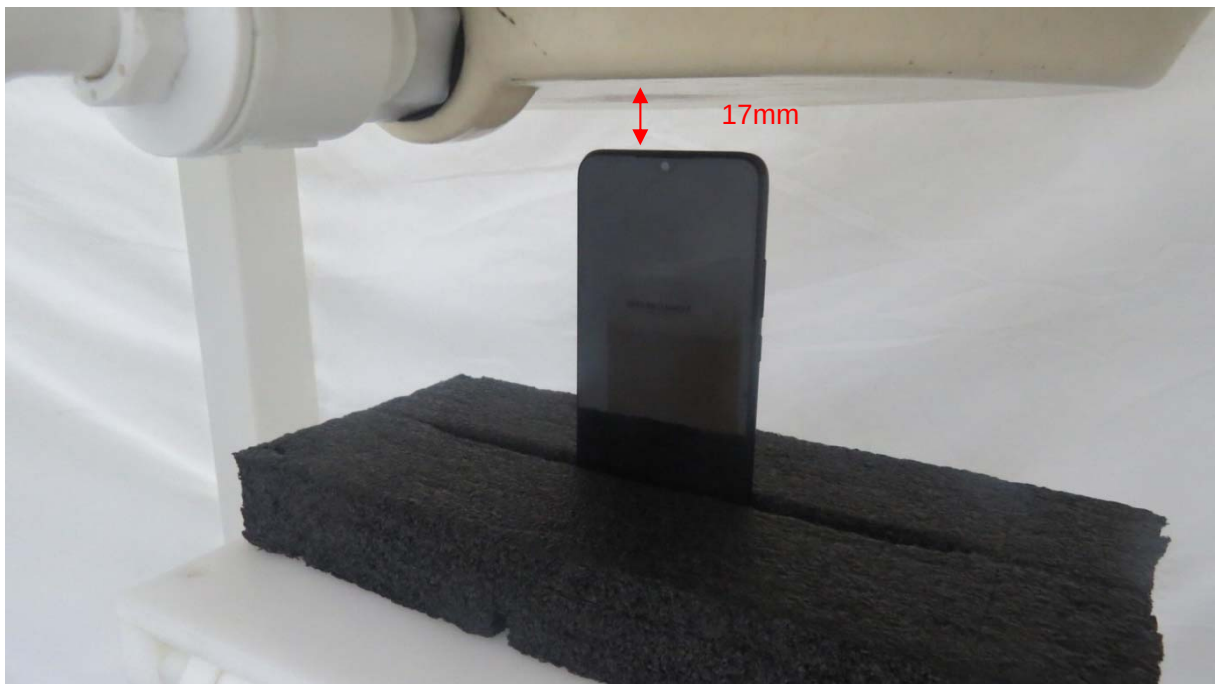
Picture 18: Top Edge, the distance from handset to the bottom of the Phantom is 17mm
