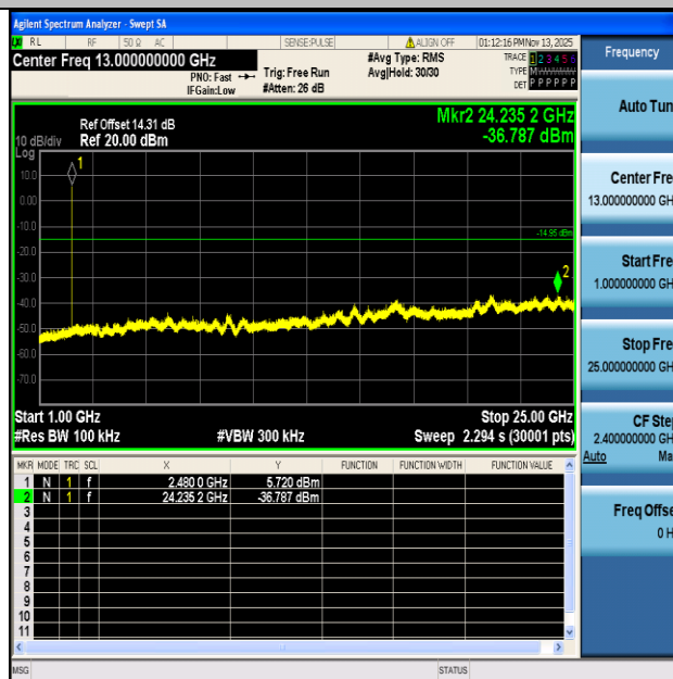
BLE_2M-Ant1-2480-1000~25000-PASS
