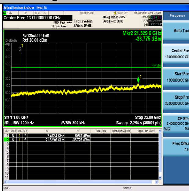
BLE_1M-Ant1-2402-1000~25000-PASS
