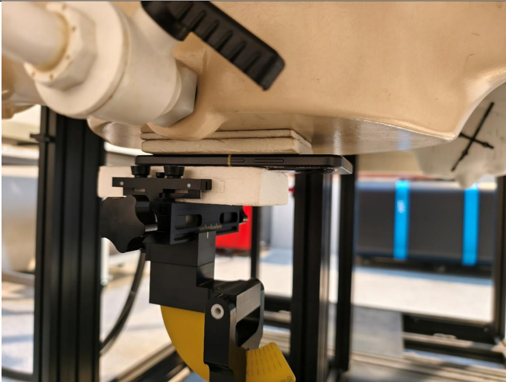
Body SAR Back side 15mm
