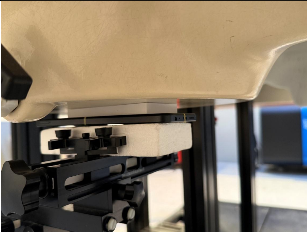
Body SAR Front side 11mm
