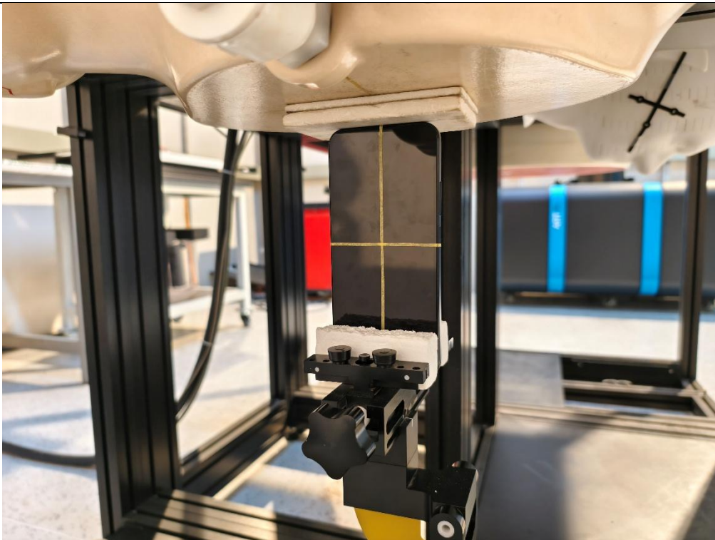
Body SAR Top side 15mm
