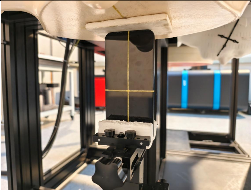
Body SAR Top side 10mm
