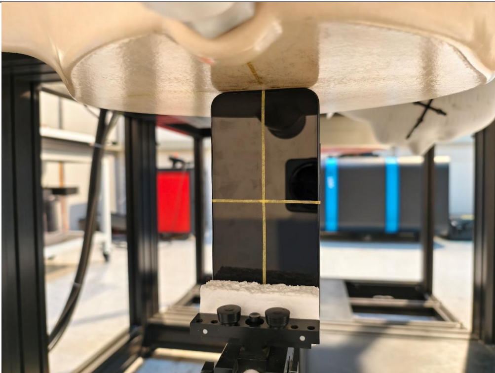
Body SAR Top side 0mm
