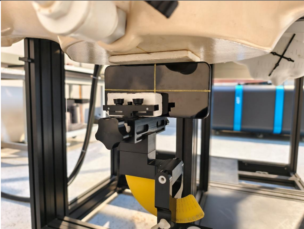
Body SAR Right side 10mm
