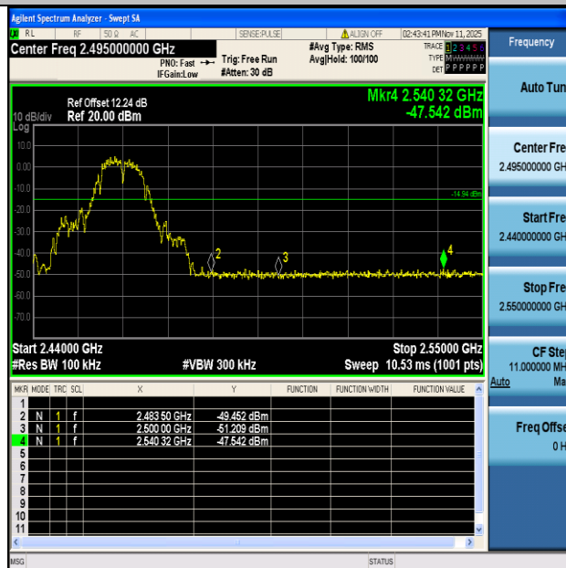
11B-Ant1-2462-PASS
