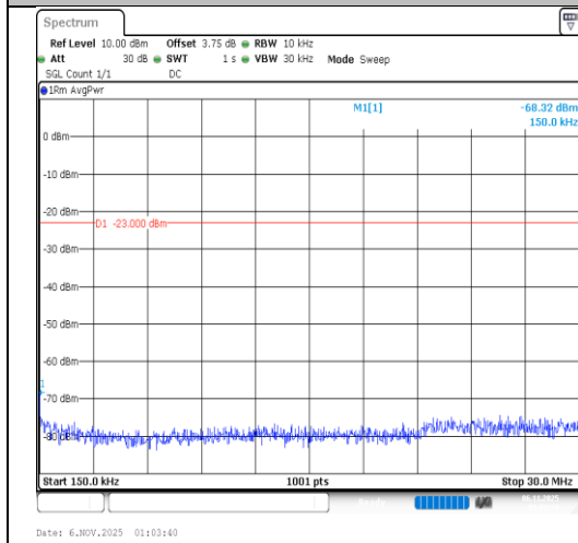
Band13-5MHz-QPSK-23230-1RB#0-0.15~30-PASS
