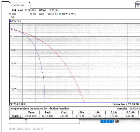
Band13-5MHz-QPSK-23255-1RB#0-PASS
