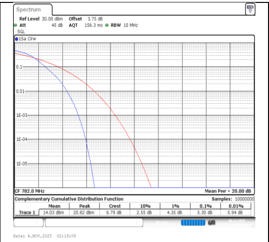
Band13-10MHz-QPSK-23230-50RB#0-PASS
