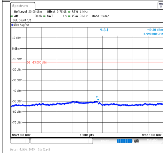
Band13-5MHz-16QAM-23205-25RB#0-3000~10000-PASS
