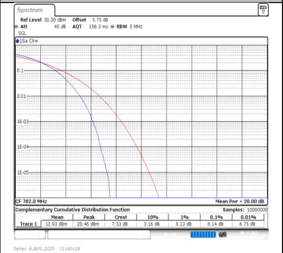
Band13-5MHz-16QAM-23230-25RB#0-PASS
