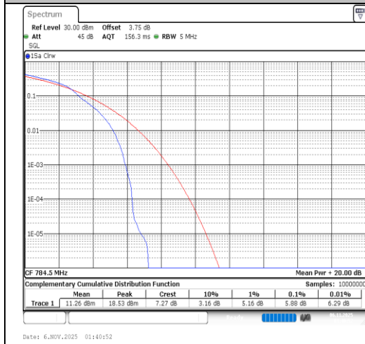
Band13-5MHz-64QAM-23255-1RB#0-PASS
