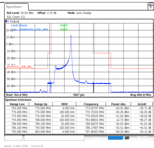
Band13-5MHz-QPSK-23205-1RB#24-PASS
