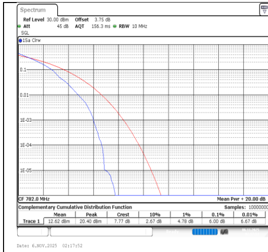
Band13-10MHz-QPSK-23230-1RB#0-PASS
