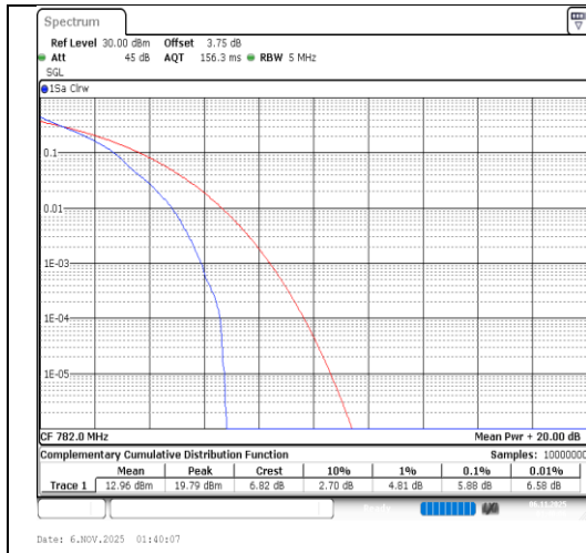
Band13-5MHz-QPSK-23230-1RB#0-PASS
