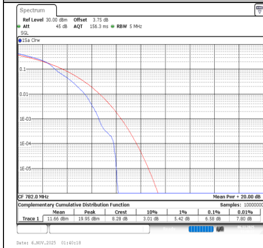
Band13-5MHz-64QAM-23230-1RB#0-PASS
