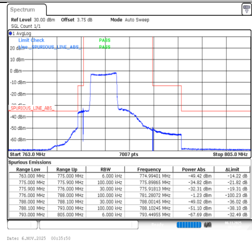
Band13-5MHz-64QAM-23205-25RB#0-PASS
