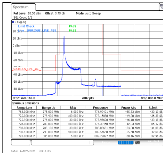
Band13-5MHz-QPSK-23205-1RB#0-PASS
