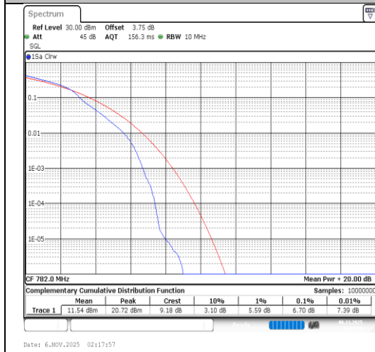
Band13-10MHz-16QAM-23230-1RB#0-PASS
