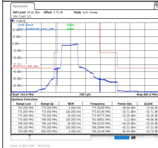
Band13-5MHz-QPSK-23205-25RB#0-PASS
