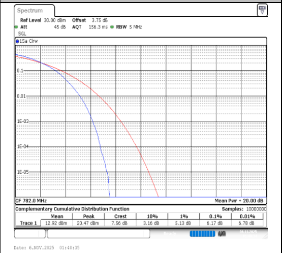
Band13-5MHz-64QAM-23230-25RB#0-PASS
