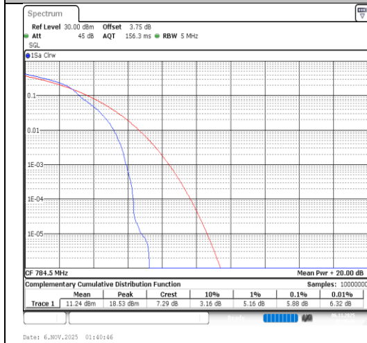
Band13-5MHz-16QAM-23255-1RB#0-PASS
