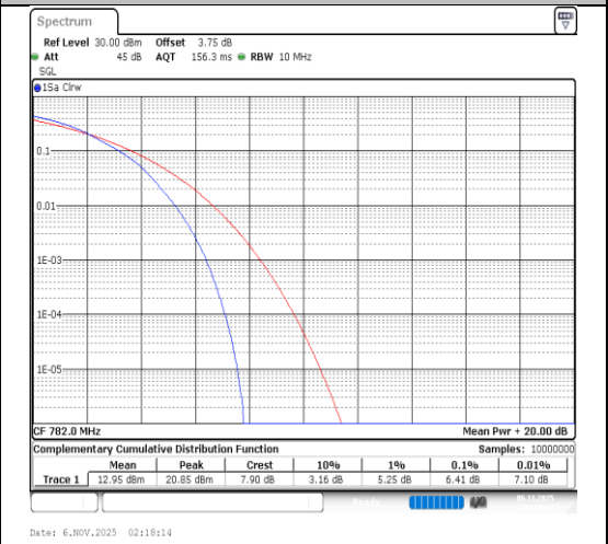
Band13-10MHz-16QAM-23230-50RB#0-PASS
