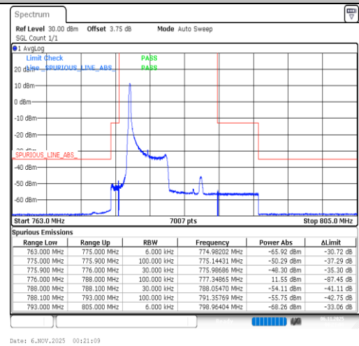
Band13-5MHz-64QAM-23205-1RB#0-PASS
