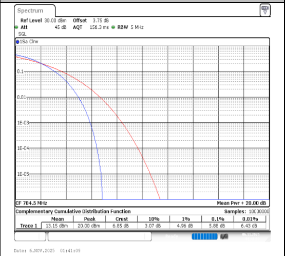
Band13-5MHz-64QAM-23255-25RB#0-PASS
