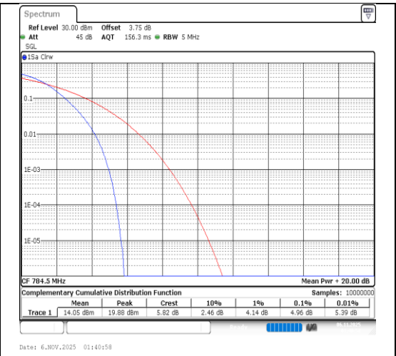
Band13-5MHz-QPSK-23255-25RB#0-PASS
