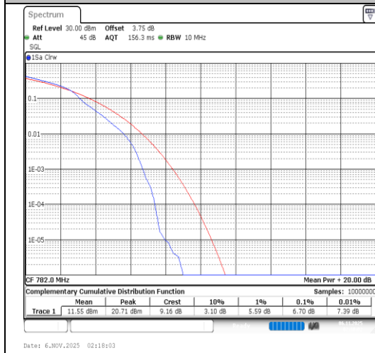
Band13-10MHz-64QAM-23230-1RB#0-PASS
