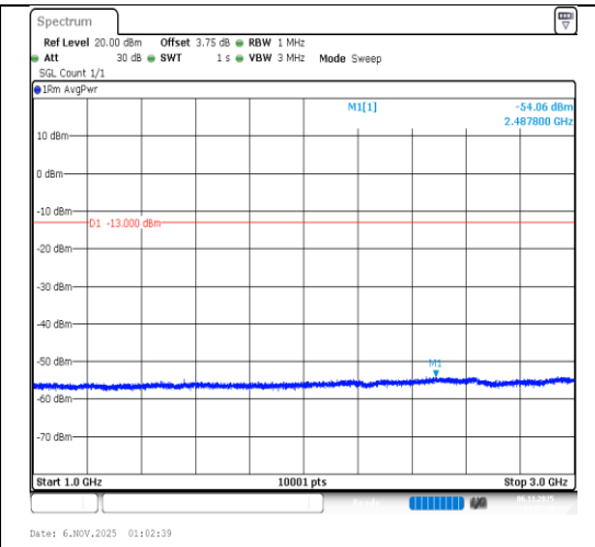
Band13-5MHz-16QAM-23205-25RB#0-1000~3000-PASS
