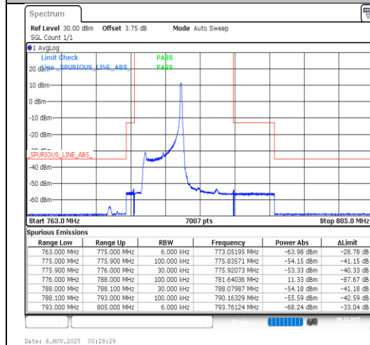
Band13-5MHz-64QAM-23205-1RB#24-PASS
