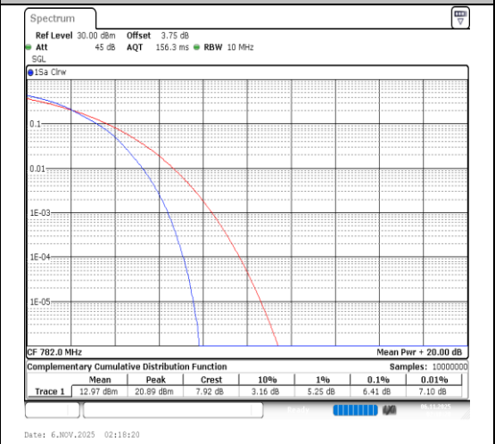
Band13-10MHz-64QAM-23230-50RB#0-PASS
