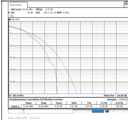
Band13-5MHz-16QAM-23230-1RB#0-PASS
