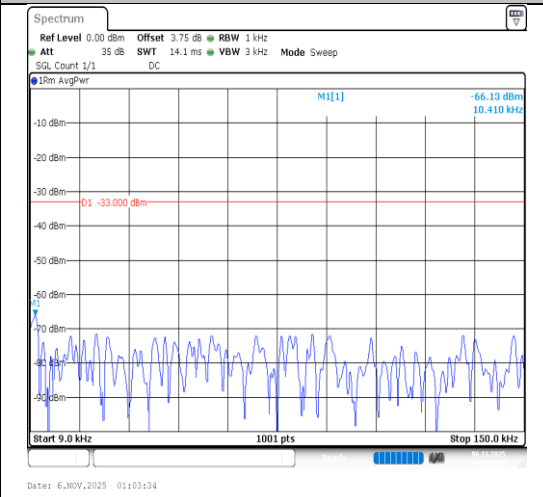
Band13-5MHz-QPSK-23230-1RB#0-0.009~0.15-PASS
