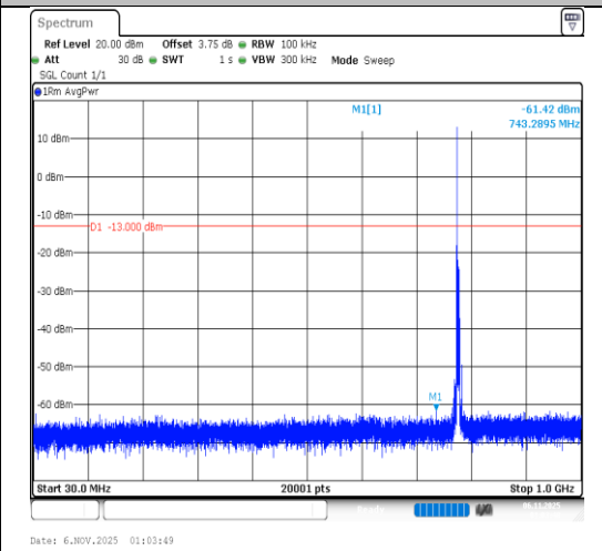
Band13-5MHz-QPSK-23230-1RB#0-30~1000-PASS
