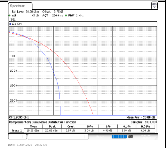
Band2-1.4MHz-16QAM-19193-6RB#0-PASS
