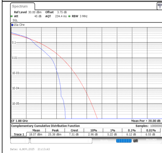
Band2-3MHz-64QAM-18900-1RB#0-PASS
