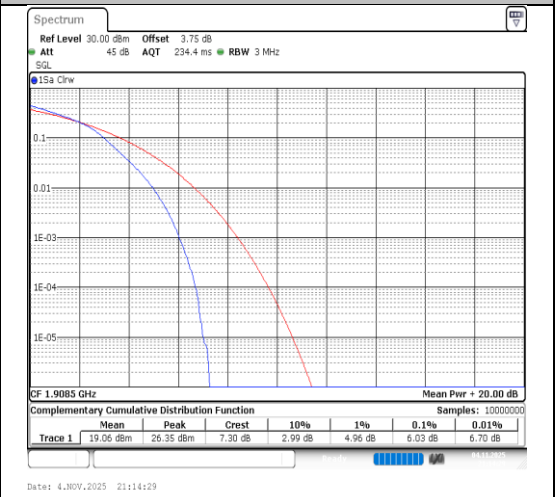
Band2-3MHz-16QAM-19185-15RB#0-PASS
