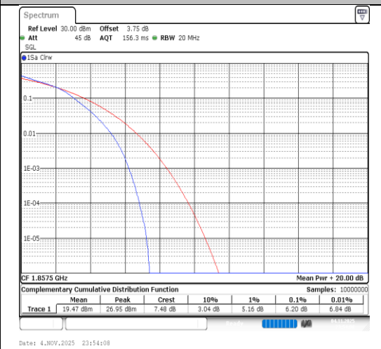
Band2-15MHz-16QAM-18675-75RB#0-PASS
