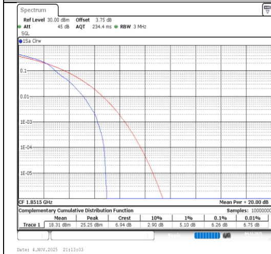
Band2-3MHz-16QAM-18615-1RB#0-PASS
