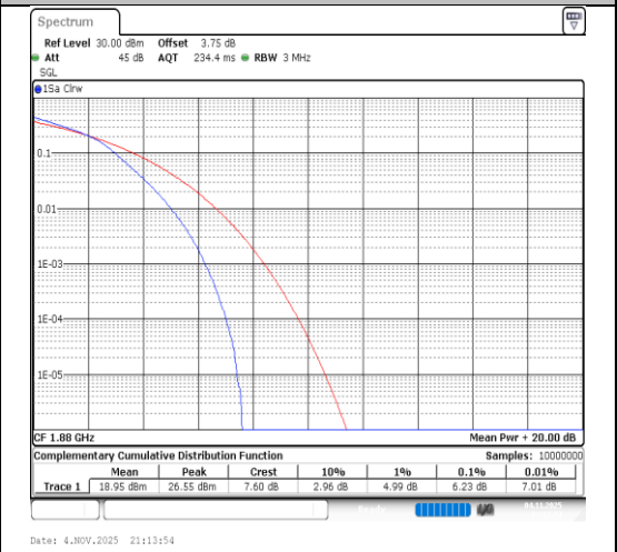
Band2-3MHz-16QAM-18900-15RB#0-PASS
