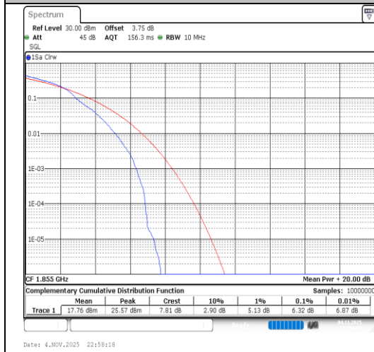
Band2-10MHz-64QAM-18650-1RB#0-PASS
