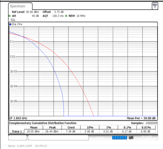
Band2-10MHz-64QAM-18650-50RB#0-PASS
