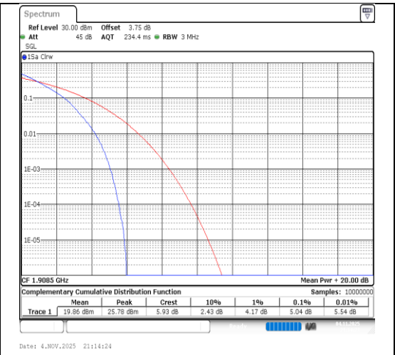
Band2-3MHz-QPSK-19185-15RB#0-PASS
