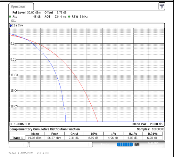
Band2-3MHz-64QAM-19185-15RB#0-PASS
