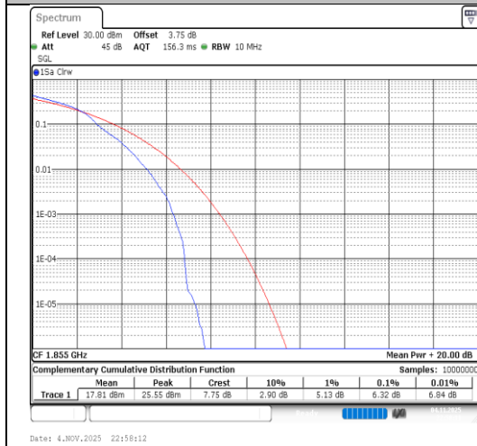
Band2-10MHz-16QAM-18650-1RB#0-PASS
