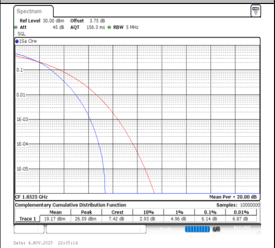
Band2-5MHz-64QAM-18625-25RB#0-PASS
