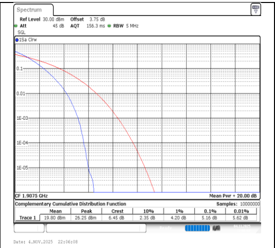
Band2-5MHz-QPSK-19175-25RB#0-PASS
