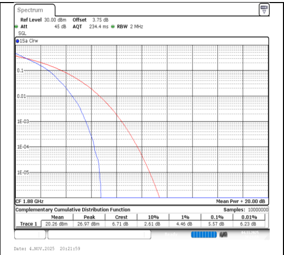
Band2-1.4MHz-QPSK-18900-6RB#0-PASS
