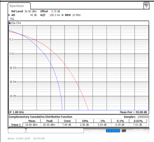
Band2-10MHz-64QAM-18900-50RB#0-PASS
