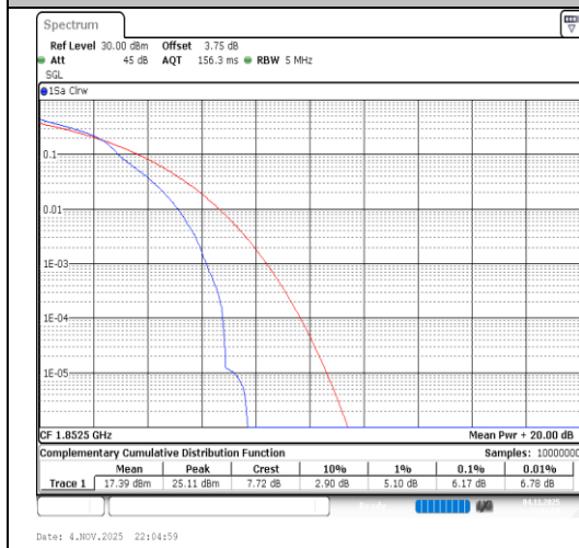
Band2-5MHz-64QAM-18625-1RB#0-PASS
