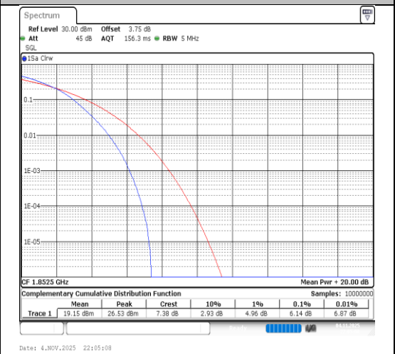
Band2-5MHz-16QAM-18625-25RB#0-PASS
