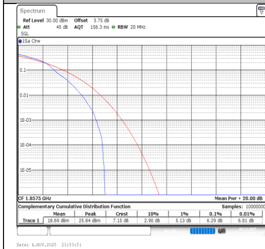
Band2-15MHz-16QAM-18675-1RB#0-PASS
