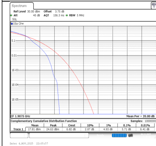
Band2-5MHz-16QAM-19175-1RB#0-PASS
