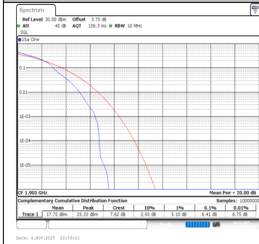
Band2-10MHz-64QAM-19150-1RB#0-PASS
