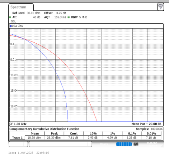
Band2-5MHz-64QAM-18900-25RB#0-PASS
