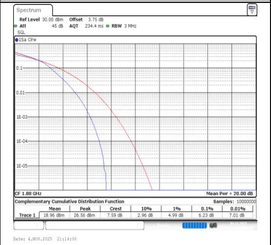
Band2-3MHz-64QAM-18900-15RB#0-PASS
