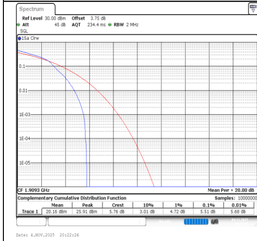
Band2-1.4MHz-64QAM-19193-1RB#0-PASS
