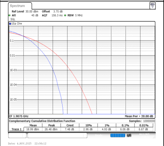
Band2-5MHz-16QAM-19175-25RB#0-PASS
