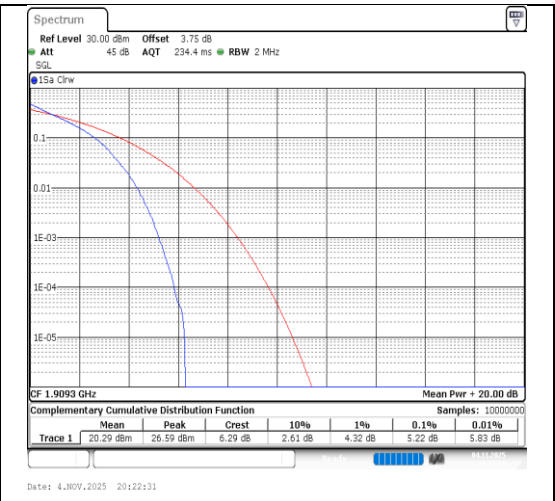
Band2-1.4MHz-QPSK-19193-6RB#0-PASS
