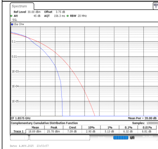
Band2-15MHz-64QAM-18675-1RB#0-PASS
