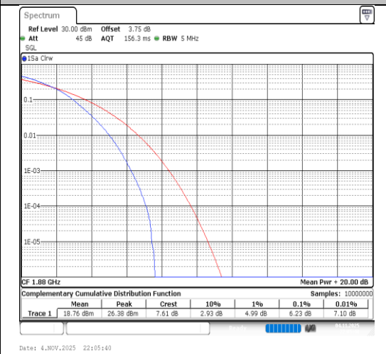
Band2-5MHz-16QAM-18900-25RB#0-PASS
