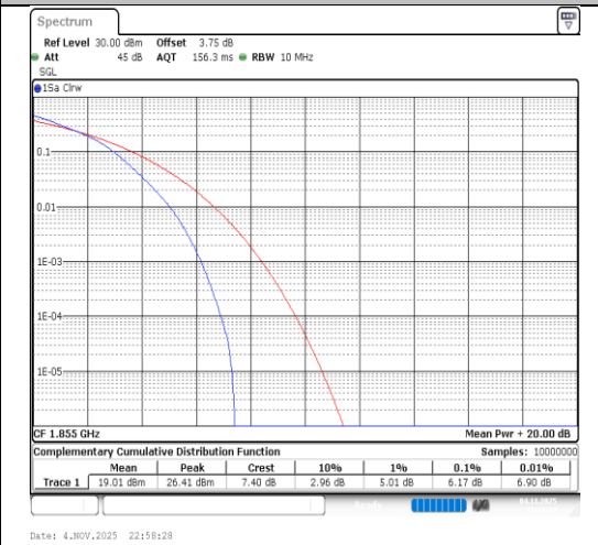
Band2-10MHz-16QAM-18650-50RB#0-PASS
