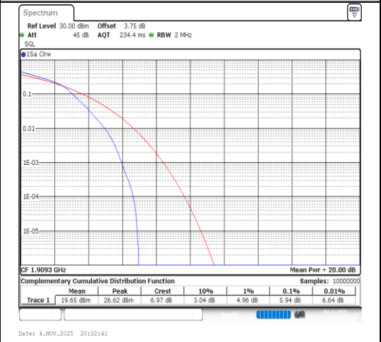
Band2-1.4MHz-64QAM-19193-6RB#0-PASS
