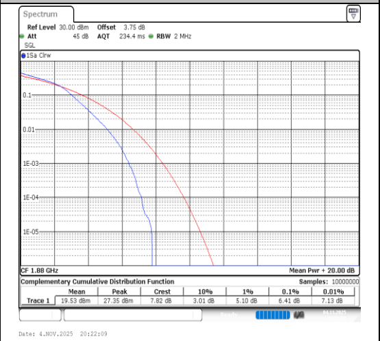
Band2-1.4MHz-64QAM-18900-6RB#0-PASS
