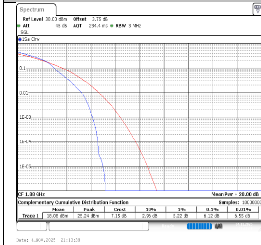
Band2-3MHz-16QAM-18900-1RB#0-PASS
