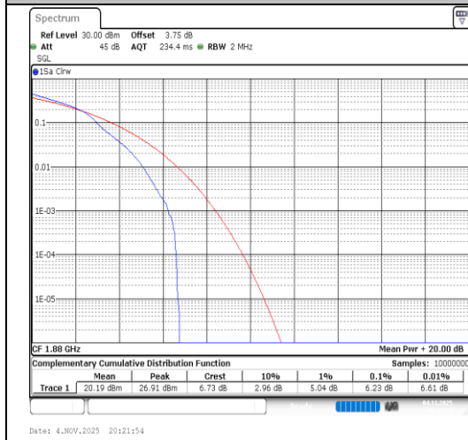
Band2-1.4MHz-64QAM-18900-1RB#0-PASS
