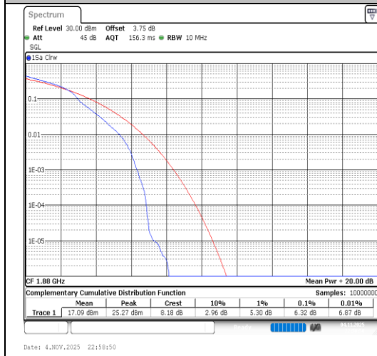
Band2-10MHz-64QAM-18900-1RB#0-PASS
