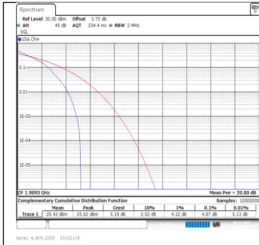
Band2-1.4MHz-QPSK-19193-1RB#0-PASS
