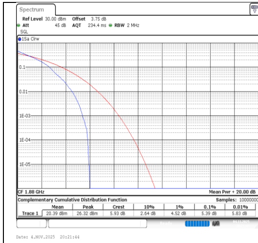
Band2-1.4MHz-QPSK-18900-1RB#0-PASS
