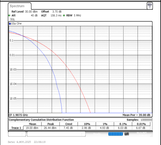
Band2-5MHz-64QAM-19175-25RB#0-PASS
