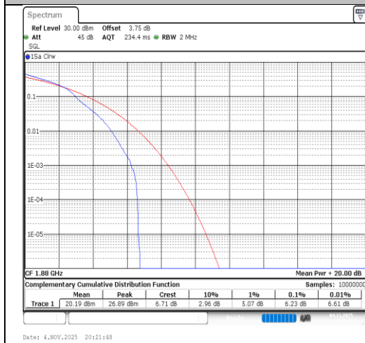
Band2-1.4MHz-16QAM-18900-1RB#0-PASS
