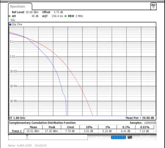
Band2-1.4MHz-16QAM-18900-6RB#0-PASS
