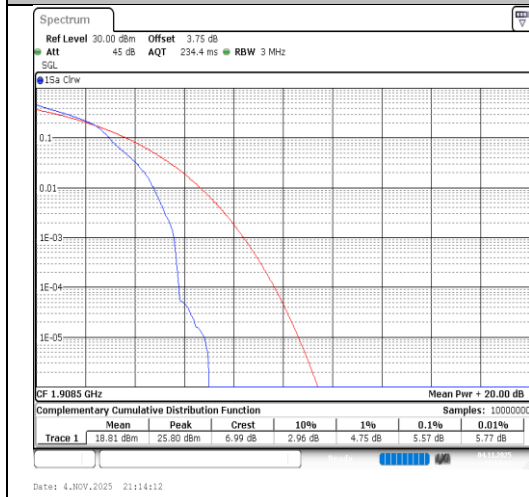
Band2-3MHz-16QAM-19185-1RB#0-PASS
