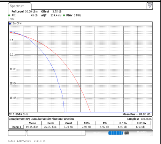
Band2-3MHz-64QAM-18615-15RB#0-PASS
