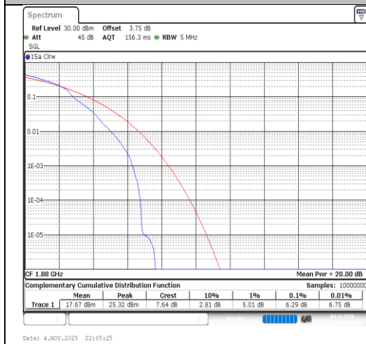
Band2-5MHz-16QAM-18900-1RB#0-PASS
