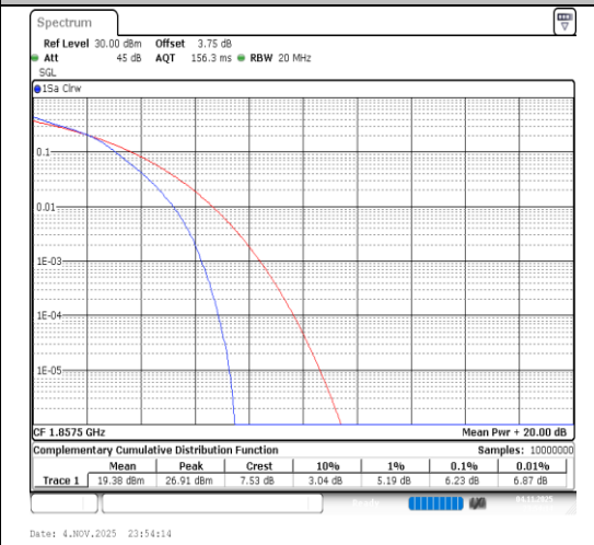
Band2-15MHz-64QAM-18675-75RB#0-PASS
