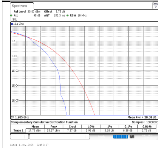
Band2-10MHz-16QAM-19150-1RB#0-PASS
