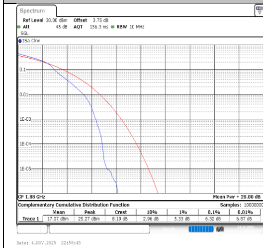
Band2-10MHz-16QAM-18900-1RB#0-PASS
