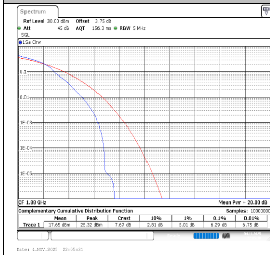
Band2-5MHz-64QAM-18900-1RB#0-PASS
