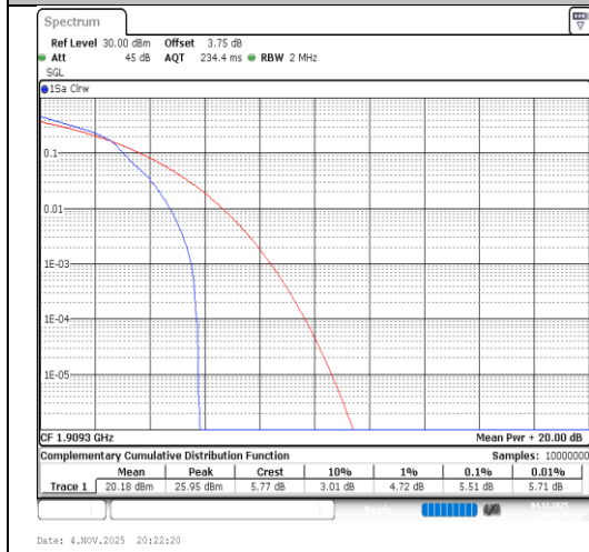
Band2-1.4MHz-16QAM-19193-1RB#0-PASS
