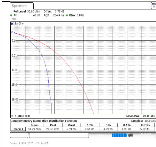
Band2-3MHz-QPSK-19185-1RB#0-PASS
