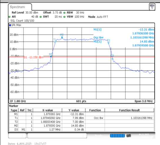
Band2-1.4MHz-16QAM-18900-6RB#0-PASS
