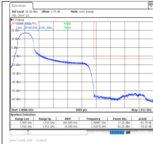
Band2-1.4MHz-64QAM-19193-1RB#0-PASS
