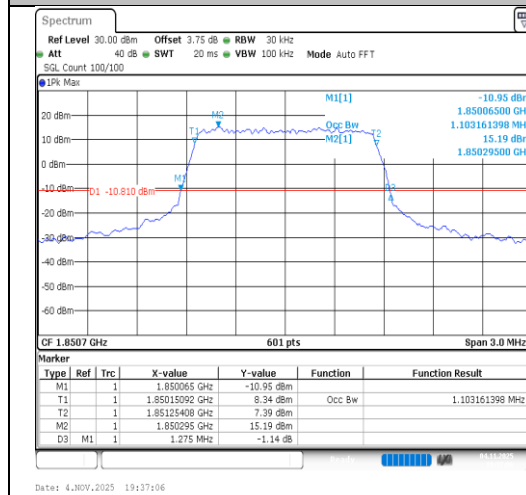
Band2-1.4MHz-16QAM-18607-6RB#0-PASS
