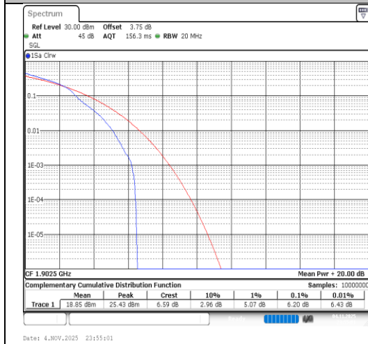
Band2-15MHz-16QAM-19125-1RB#0-PASS
