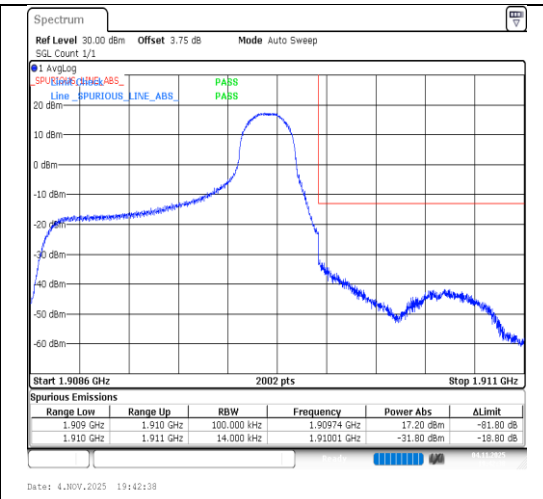
Band2-1.4MHz-64QAM-19193-1RB#5-PASS
