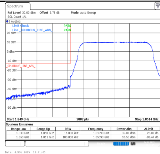
Band2-1.4MHz-64QAM-18607-6RB#0-PASS
