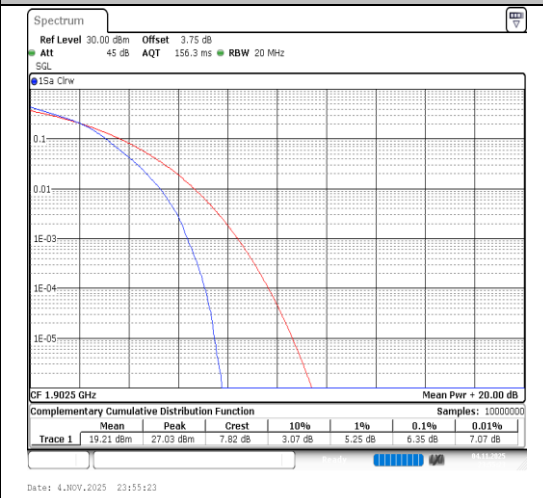
Band2-15MHz-64QAM-19125-75RB#0-PASS
