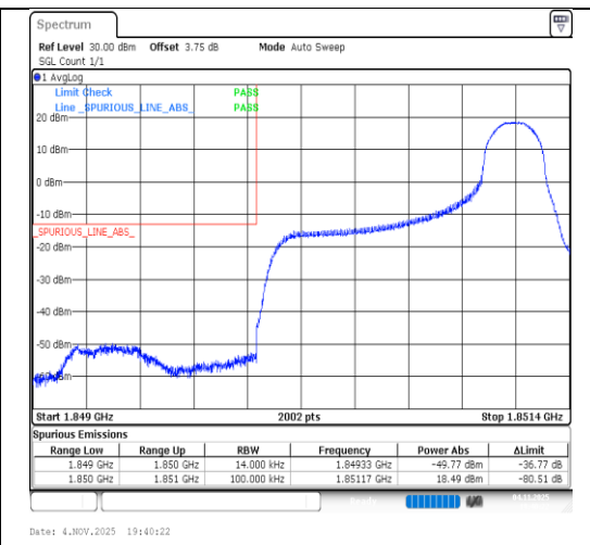
Band2-1.4MHz-16QAM-18607-1RB#5-PASS
