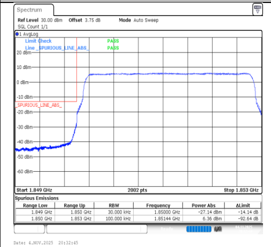
Band2-3MHz-64QAM-18615-15RB#0-PASS
