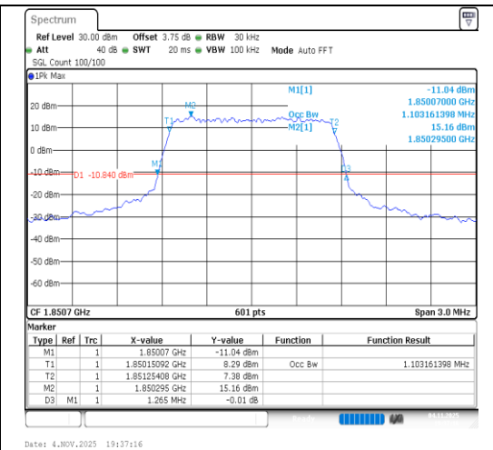
Band2-1.4MHz-64QAM-18607-6RB#0-PASS
