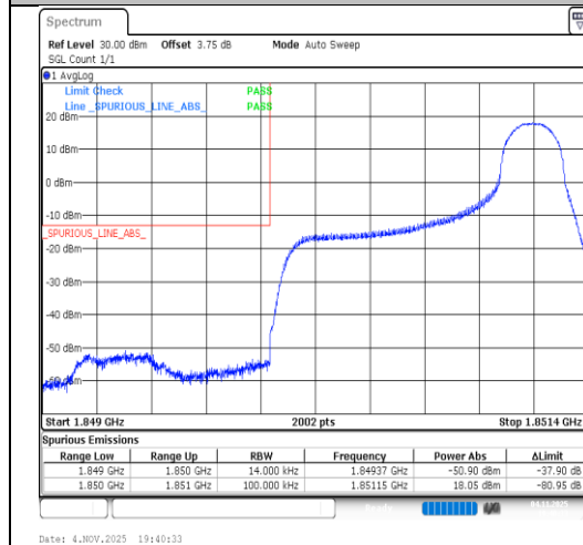
Band2-1.4MHz-64QAM-18607-1RB#5-PASS
