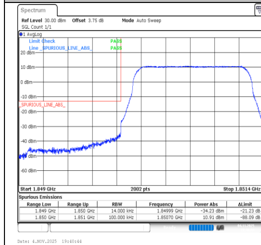
Band2-1.4MHz-QPSK-18607-6RB#0-PASS
