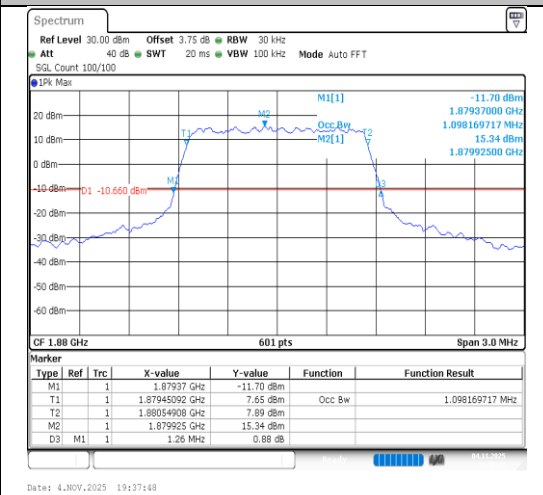
Band2-1.4MHz-QPSK-18900-6RB#0-PASS
