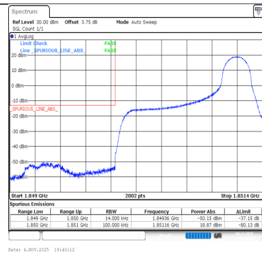
Band2-1.4MHz-QPSK-18607-1RB#5-PASS
