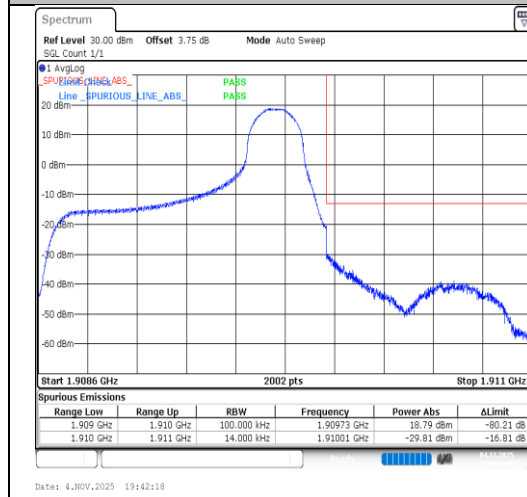
Band2-1.4MHz-QPSK-19193-1RB#5-PASS
