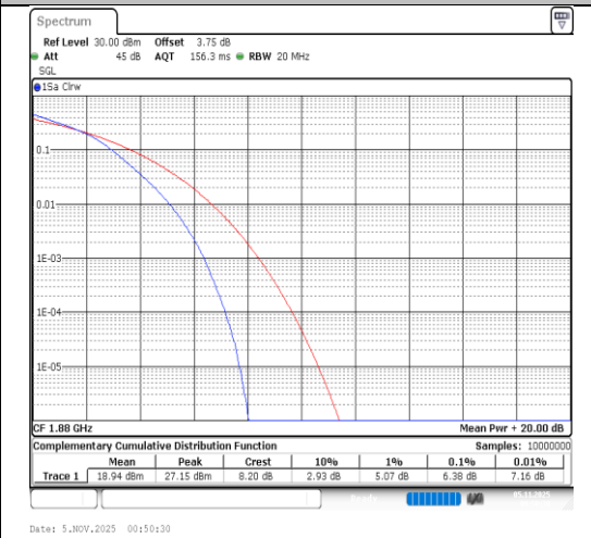
Band2-20MHz-16QAM-18900-100RB#0-PASS
