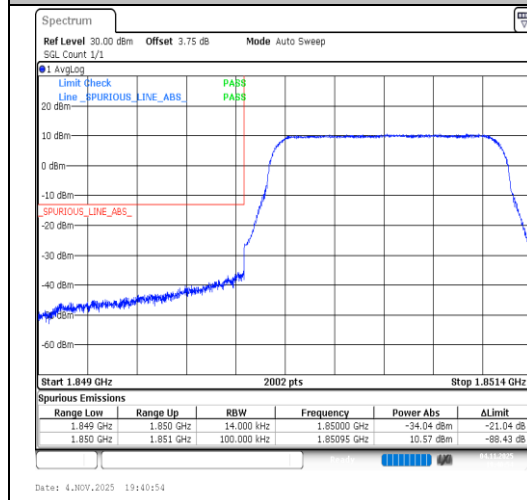
Band2-1.4MHz-16QAM-18607-6RB#0-PASS
