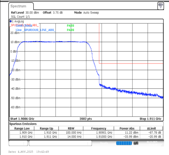
Band2-1.4MHz-QPSK-19193-6RB#0-PASS
