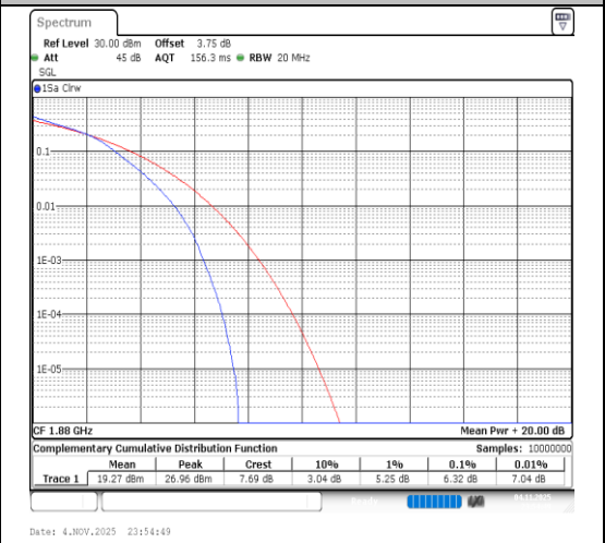
Band2-15MHz-64QAM-18900-75RB#0-PASS
