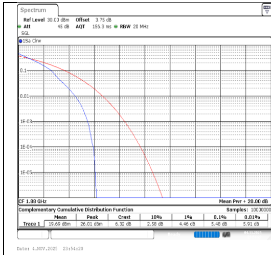
Band2-15MHz-QPSK-18900-1RB#0-PASS
