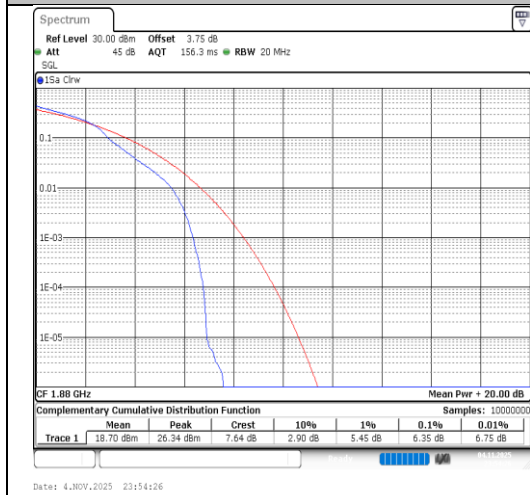
Band2-15MHz-16QAM-18900-1RB#0-PASS
