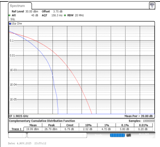
Band2-15MHz-QPSK-19125-75RB#0-PASS
