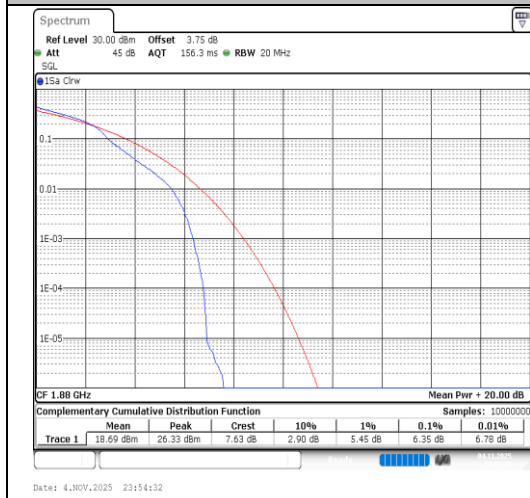
Band2-15MHz-64QAM-18900-1RB#0-PASS
