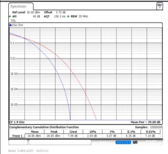
Band2-20MHz-64QAM-19100-100RB#0-PASS
