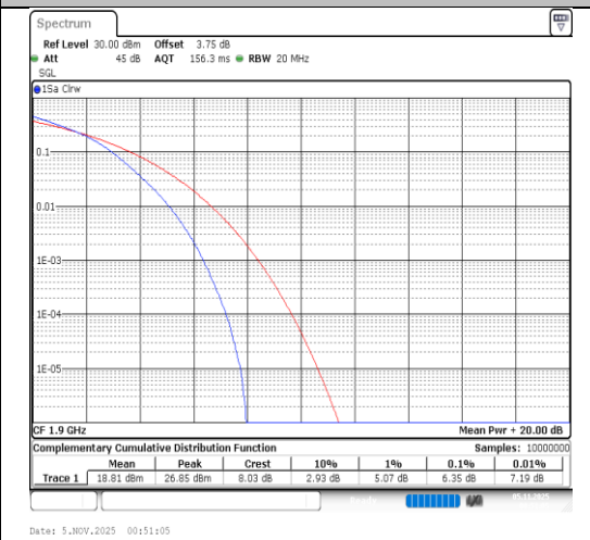
Band2-20MHz-16QAM-19100-100RB#0-PASS
