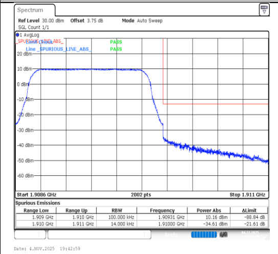
Band2-1.4MHz-16QAM-19193-6RB#0-PASS
