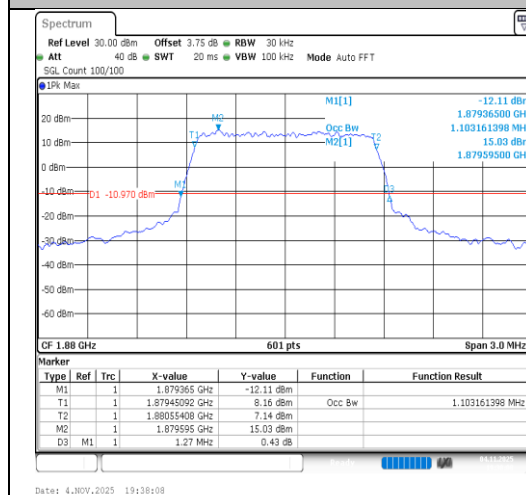
Band2-1.4MHz-64QAM-18900-6RB#0-PASS
