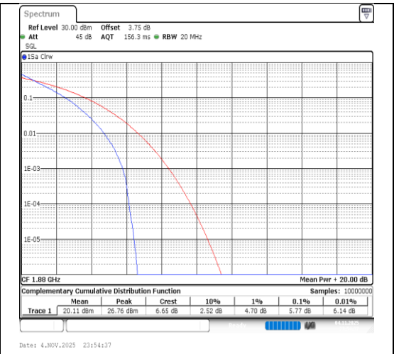
Band2-15MHz-QPSK-18900-75RB#0-PASS
