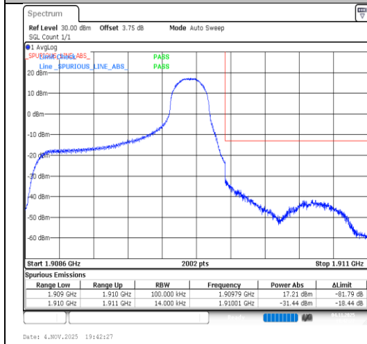
Band2-1.4MHz-16QAM-19193-1RB#5-PASS
