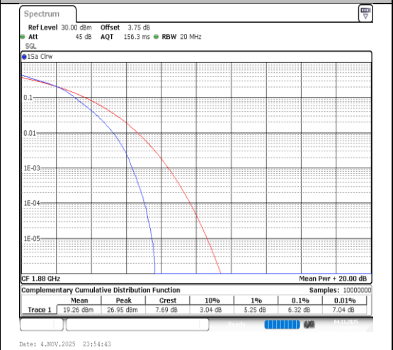
Band2-15MHz-16QAM-18900-75RB#0-PASS
