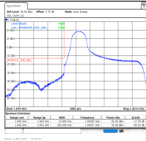
Band2-1.4MHz-64QAM-18607-1RB#0-PASS
