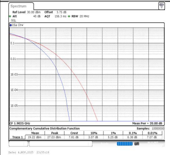
Band2-15MHz-16QAM-19125-75RB#0-PASS
