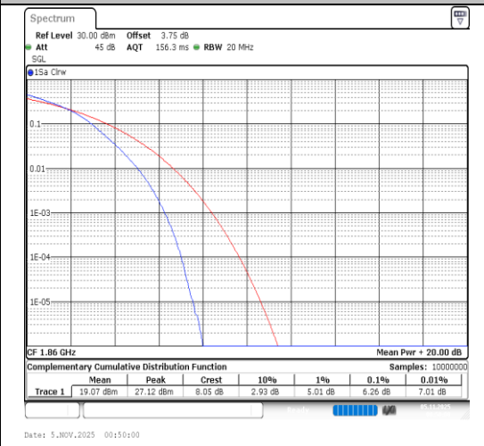
Band2-20MHz-64QAM-18700-100RB#0-PASS
