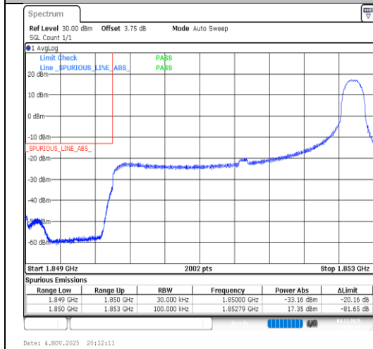
Band2-3MHz-64QAM-18615-1RB#14-PASS
