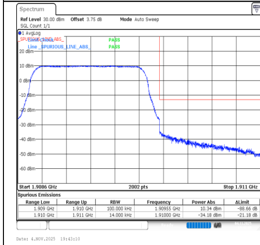
Band2-1.4MHz-64QAM-19193-6RB#0-PASS
