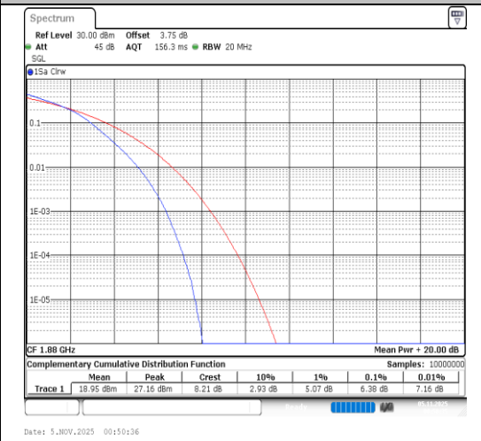
Band2-20MHz-64QAM-18900-100RB#0-PASS
