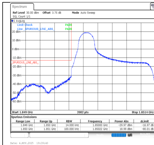
Band2-1.4MHz-QPSK-18607-1RB#0-PASS
