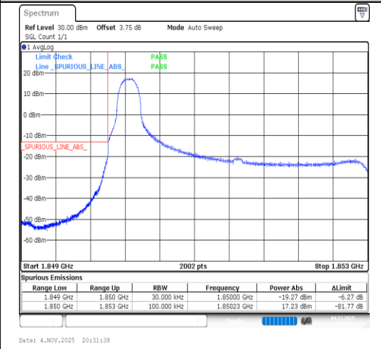
Band2-3MHz-64QAM-18615-1RB#0-PASS
