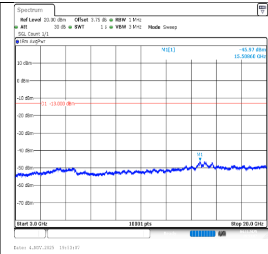
Band2-1.4MHz-QPSK-18900-6RB#0- 3000~20000-PASS
