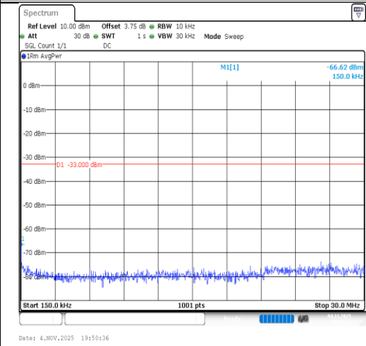
Band2-1.4MHz-64QAM-18900-1RB#0-0.15~30- PASS
