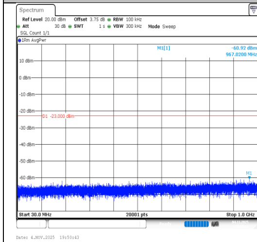
Band2-1.4MHz-64QAM-18900-1RB#0-30~1000- PASS
