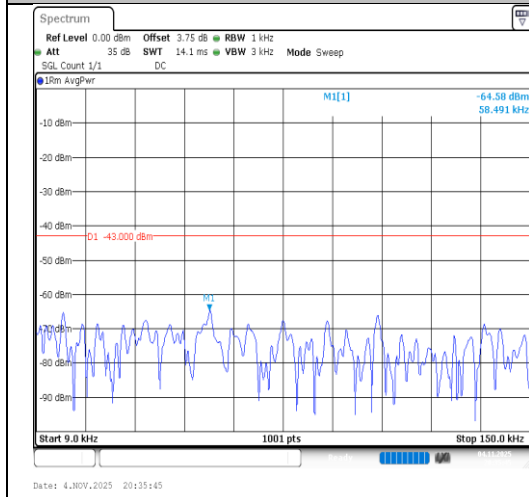
Band2-3MHz-64QAM-18615-1RB#0-0.009~0.15- PASS
