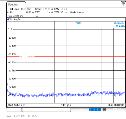
Band2-3MHz-64QAM-18615-1RB#0-0.15~30- PASS
