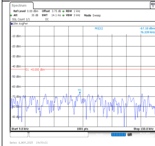
Band2-1.4MHz-64QAM-18900-1RB#0- 0.009~0.15-PASS
