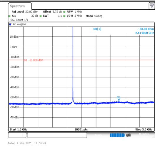
Band2-1.4MHz-64QAM-18900-1RB#0- 1000~3000-PASS
