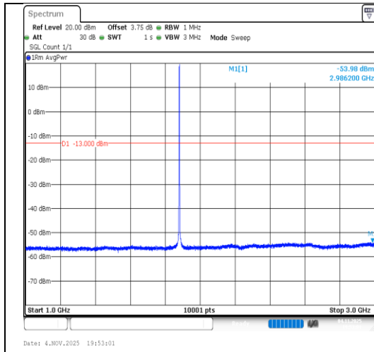
Band2-1.4MHz-QPSK-18900-6RB#0- 1000~3000-PASS
