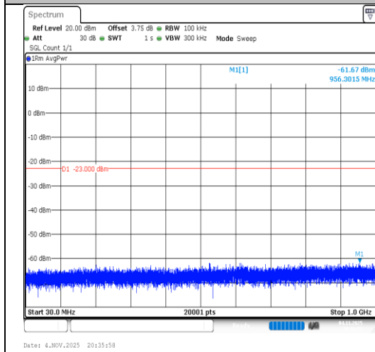
Band2-3MHz-64QAM-18615-1RB#0-30~1000- PASS
