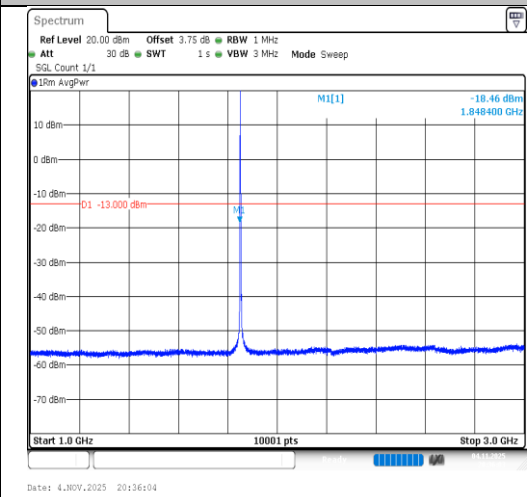
Band2-3MHz-64QAM-18615-1RB#0-1000~3000- PASS
