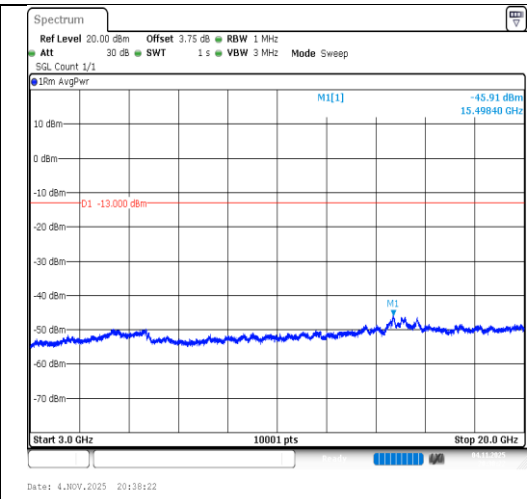
Band2-3MHz-QPSK-18615-15RB#0- 3000~20000-PASS
