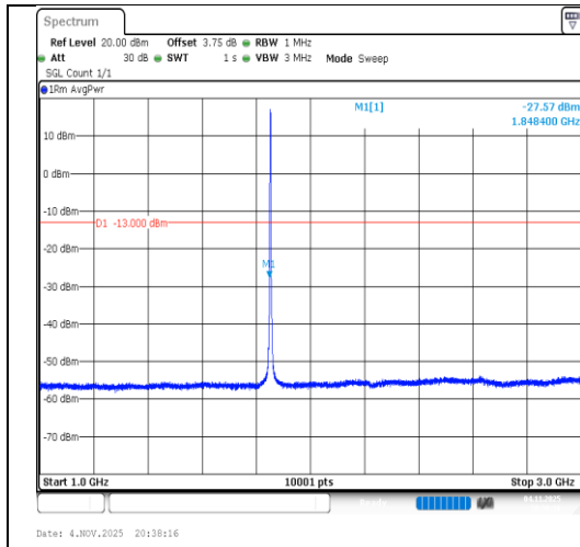
Band2-3MHz-QPSK-18615-15RB#0-1000~3000- PASS
