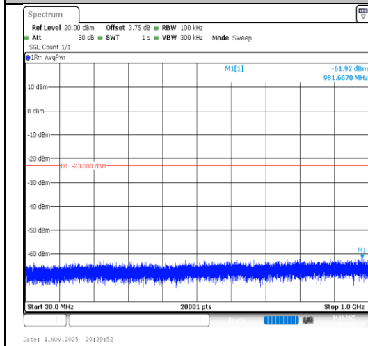
Band2-3MHz-QPSK-18900-1RB#0-30~1000- PASS
