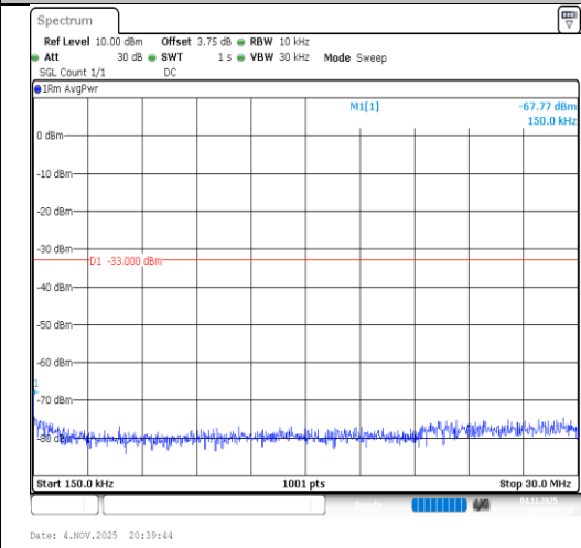
Band2-3MHz-QPSK-18900-1RB#0-0.15~30- PASS
