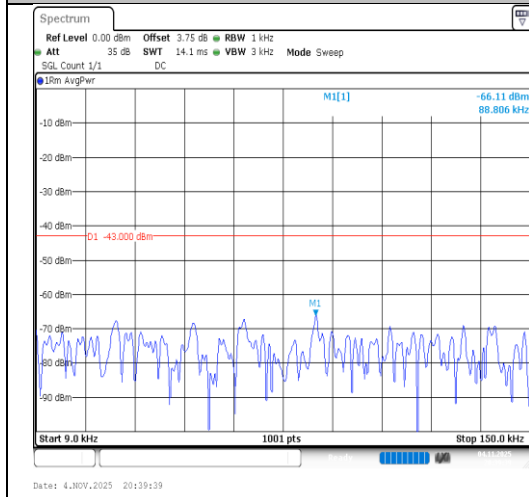
Band2-3MHz-QPSK-18900-1RB#0-0.009~0.15- PASS
