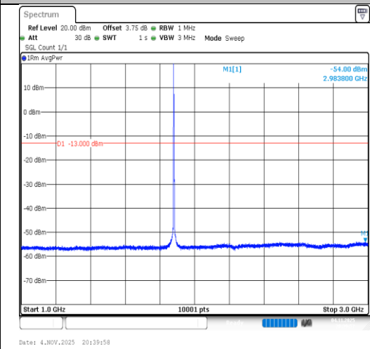
Band2-3MHz-QPSK-18900-1RB#0-1000~3000- PASS
