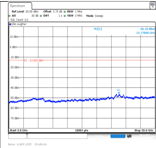
Band2-3MHz-QPSK-19185-15RB#0-3000~20000-PASS
