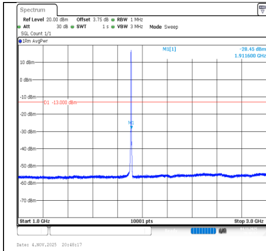
Band2-3MHz-QPSK-19185-15RB#0-1000~3000-PASS
