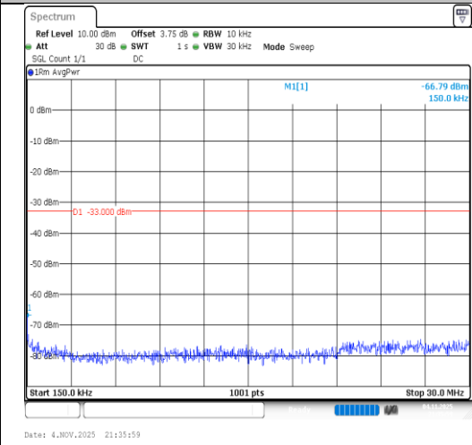
Band2-5MHz-QPSK-19175-1RB#0-0.15~30- PASS
