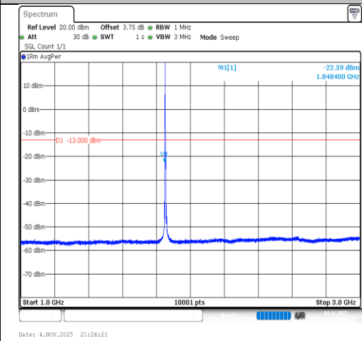
Band2-5MHz-QPSK-18625-1RB#0-1000~3000- PASS
