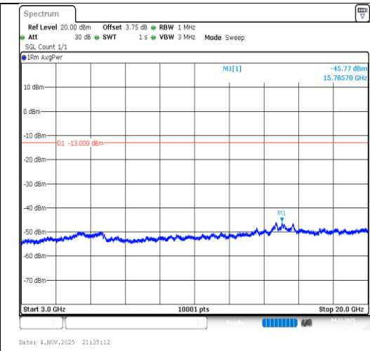
Band2-5MHz-16QAM-18900-25RB#0- 3000~20000-PASS
