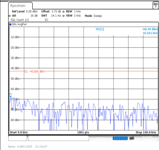
Band2-5MHz-16QAM-18900-25RB#0-0.009~0.15-PASS
