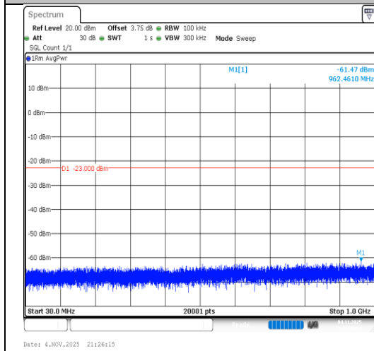
Band2-5MHz-QPSK-18625-1RB#0-30~1000- PASS
