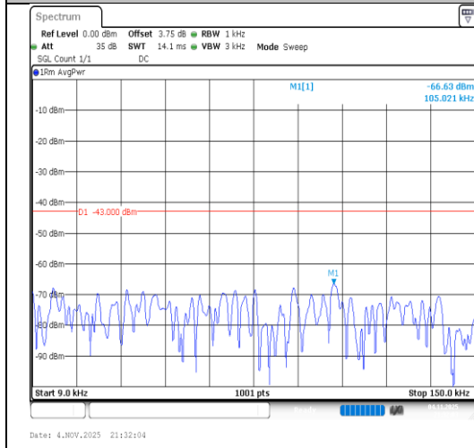
Band2-5MHz-64QAM-18900-1RB#0-0.009~0.15-PASS
