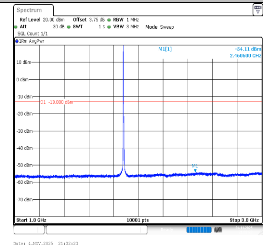
Band2-5MHz-64QAM-18900-1RB#0-1000~3000-PASS
