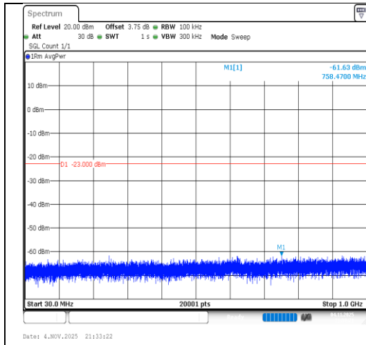
Band2-5MHz-16QAM-18900-1RB#24-30~1000-PASS
