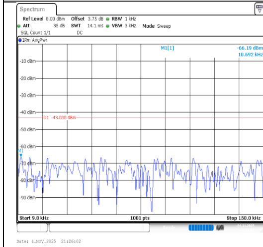
Band2-5MHz-QPSK-18625-1RB#0-0.009~0.15- PASS
