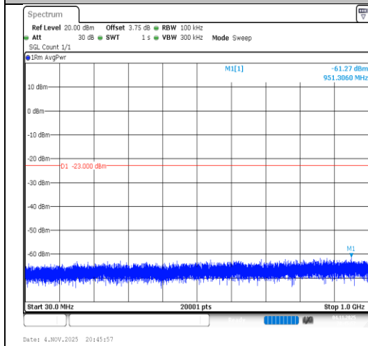
Band2-3MHz-64QAM-19185-1RB#0-30~1000-PASS
