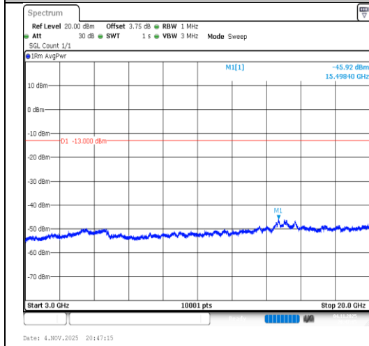
Band2-3MHz-16QAM-19185-1RB#14-3000~20000-PASS
