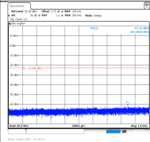
Band2-5MHz-16QAM-18900-25RB#0-30~1000-PASS
