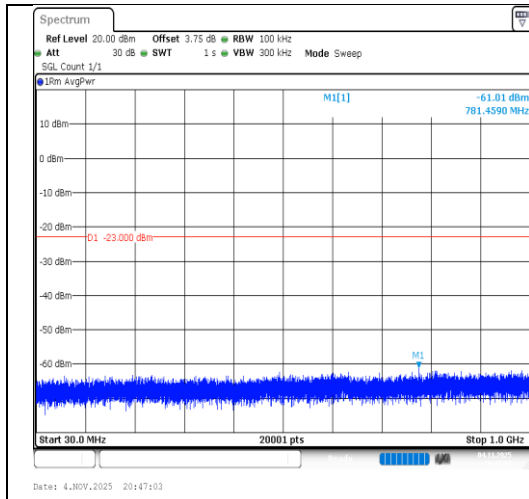
Band2-3MHz-16QAM-19185-1RB#14-30~1000-PASS
