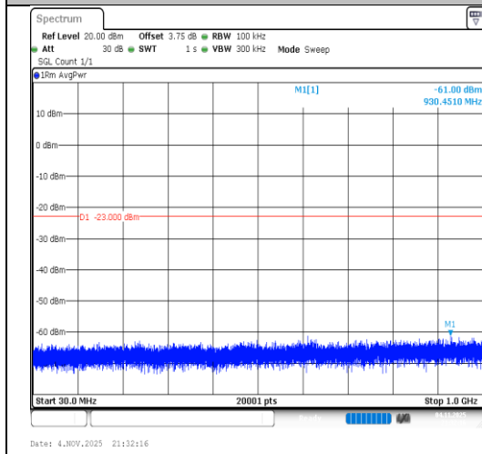
Band2-5MHz-64QAM-18900-1RB#0-30~1000-PASS
