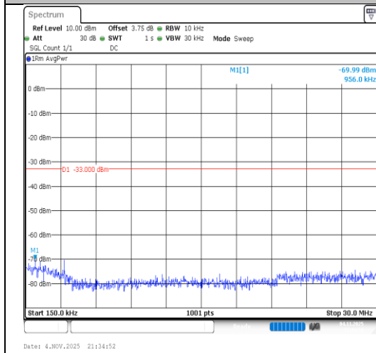
Band2-5MHz-16QAM-18900-25RB#0-0.15~30-PASS
