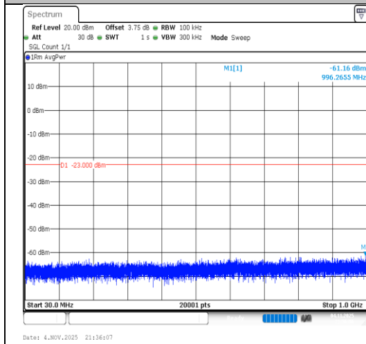
Band2-5MHz-QPSK-19175-1RB#0-30~1000- PASS
