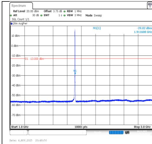
Band2-3MHz-16QAM-19185-15RB#0- 1000~3000-PASS
