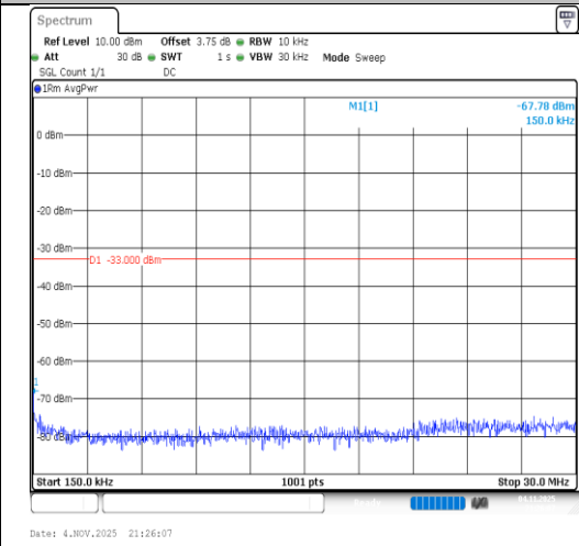
Band2-5MHz-QPSK-18625-1RB#0-0.15~30- PASS
