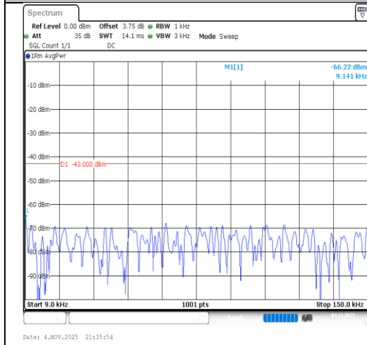
Band2-5MHz-QPSK-19175-1RB#0-0.009~0.15- PASS
