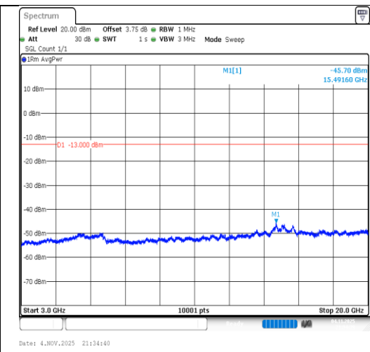
Band2-5MHz-QPSK-18900-25RB#0-3000~20000-PASS
