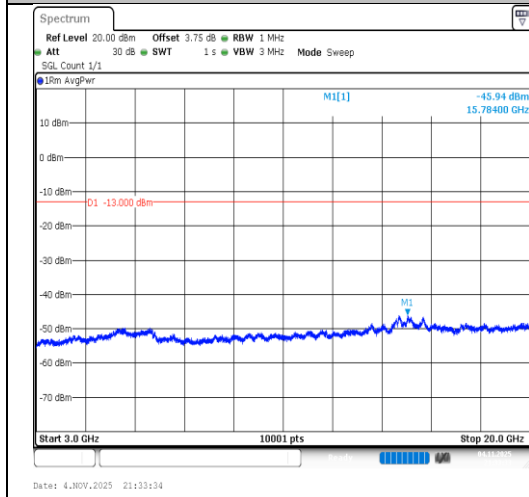
Band2-5MHz-16QAM-18900-1RB#24-3000~20000-PASS
