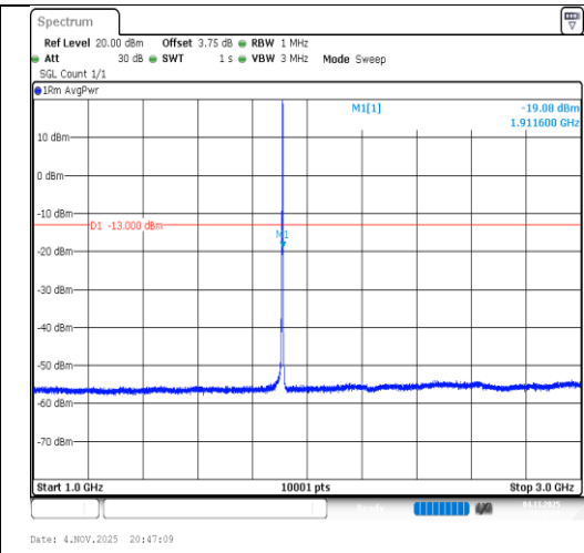
Band2-3MHz-16QAM-19185-1RB#14-1000~3000-PASS
