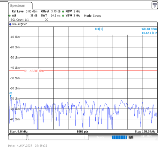
Band2-3MHz-16QAM-19185-15RB#0-0.009~0.15-PASS
