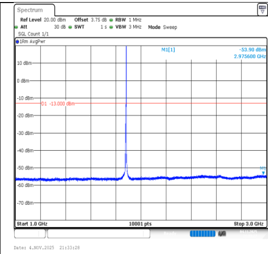
Band2-5MHz-16QAM-18900-1RB#24-1000~3000-PASS
