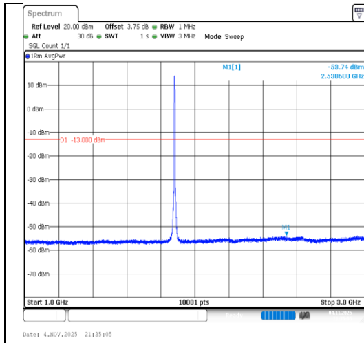
Band2-5MHz-16QAM-18900-25RB#0- 1000~3000-PASS
