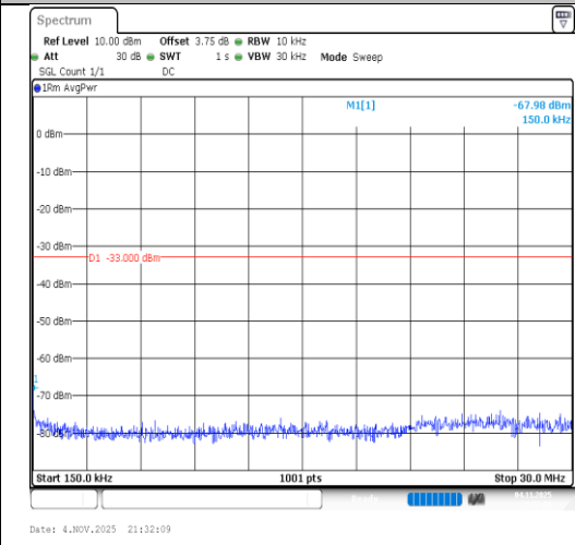
Band2-5MHz-64QAM-18900-1RB#0-0.15~30-PASS
