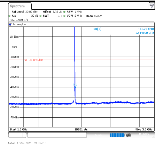
Band2-5MHz-QPSK-19175-1RB#0-1000~3000- PASS
