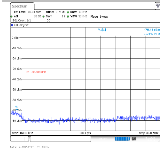
Band2-3MHz-16QAM-19185-15RB#0-0.15~30-PASS
