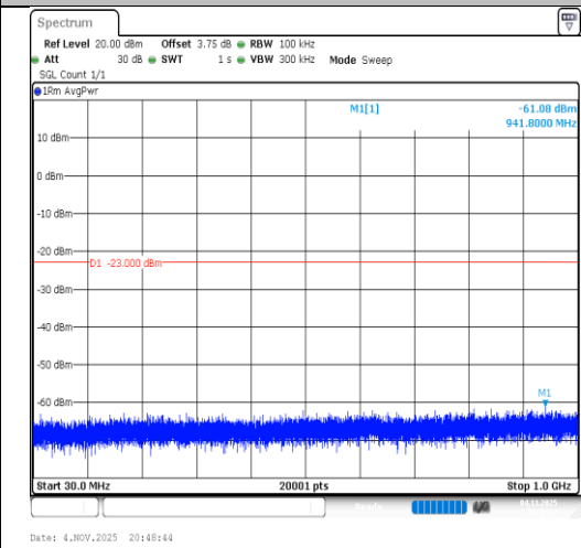
Band2-3MHz-16QAM-19185-15RB#0-30~1000-PASS
