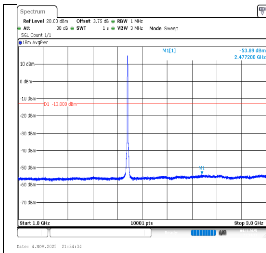
Band2-5MHz-QPSK-18900-25RB#0-1000~3000-PASS
