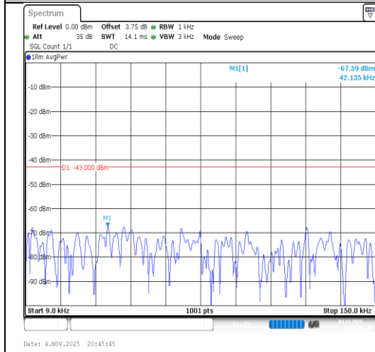
Band2-3MHz-64QAM-19185-1RB#0-0.009~0.15-PASS
