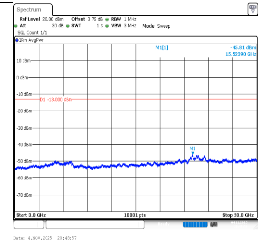
Band2-3MHz-16QAM-19185-15RB#0- 3000~20000-PASS
