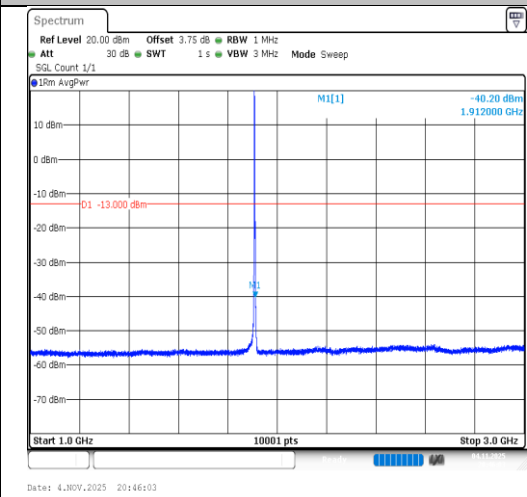
Band2-3MHz-64QAM-19185-1RB#0-1000~3000-PASS
