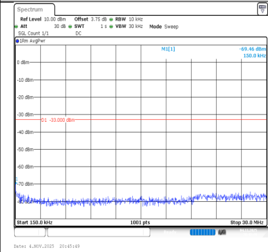
Band2-3MHz-64QAM-19185-1RB#0-0.15~30-PASS
