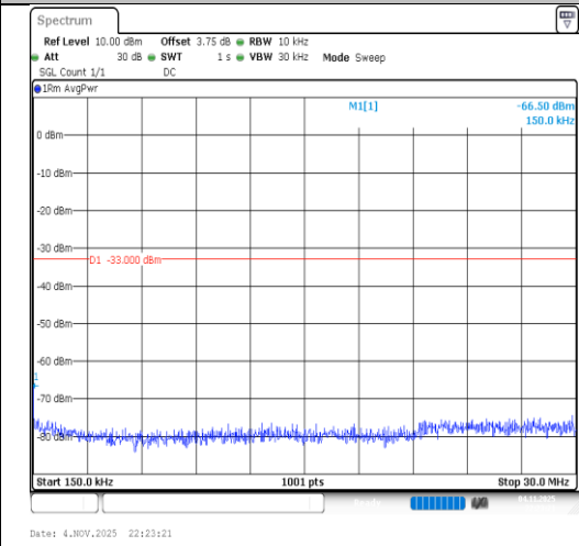
Band2-10MHz-QPSK-18900-1RB#0-0.15~30- PASS
