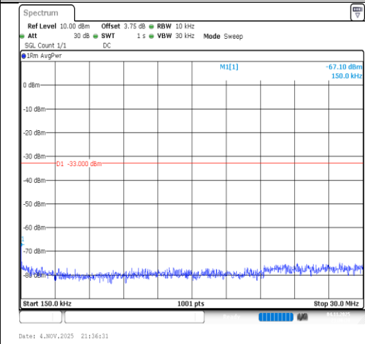
Band2-5MHz-16QAM-19175-1RB#0-0.15~30- PASS
