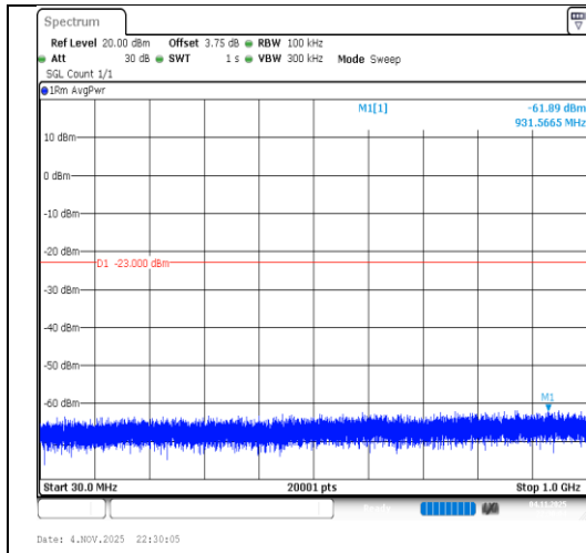
Band2-10MHz-QPSK-19150-1RB#49-30~1000-PASS
