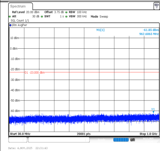
Band2-10MHz-QPSK-19150-50RB#0-30~1000-PASS
