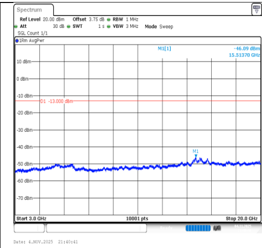
Band2-5MHz-64QAM-19175-25RB#0- 3000~20000-PASS
