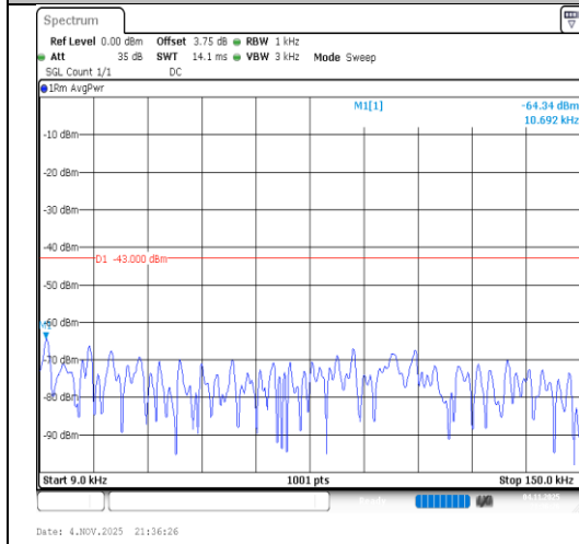
Band2-5MHz-16QAM-19175-1RB#0-0.009~0.15- PASS
