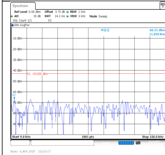
Band2-10MHz-QPSK-18900-1RB#0-0.009~0.15- PASS
