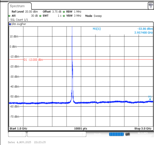
Band2-10MHz-QPSK-18900-1RB#0-1000~3000- PASS
