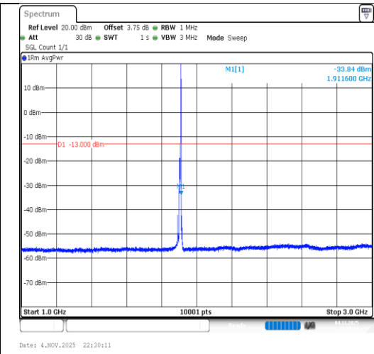
Band2-10MHz-QPSK-19150-1RB#49-1000~3000-PASS
