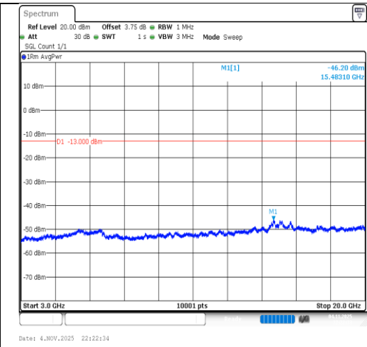
Band2-10MHz-16QAM-18650-50RB#0- 3000~20000-PASS
