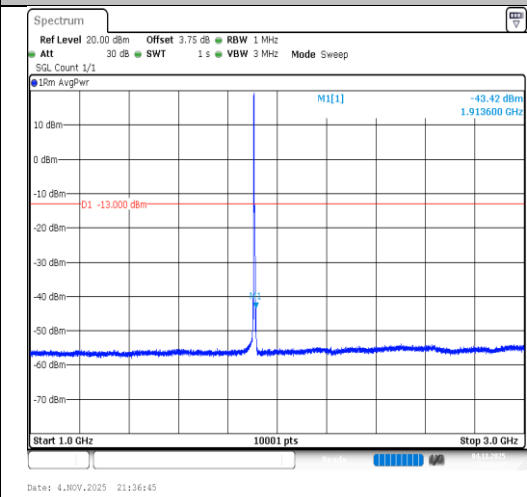
Band2-5MHz-16QAM-19175-1RB#0-1000~3000- PASS
