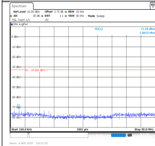
Band2-10MHz-QPSK-19150-50RB#0-0.15~30-PASS
