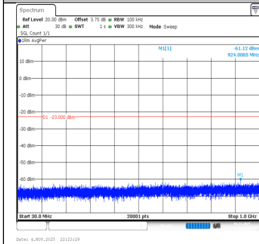
Band2-10MHz-QPSK-18900-1RB#0-30~1000- PASS
