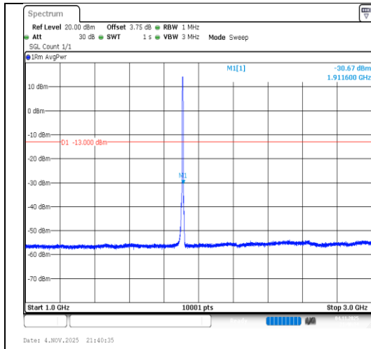
Band2-5MHz-64QAM-19175-25RB#0- 1000~3000-PASS
