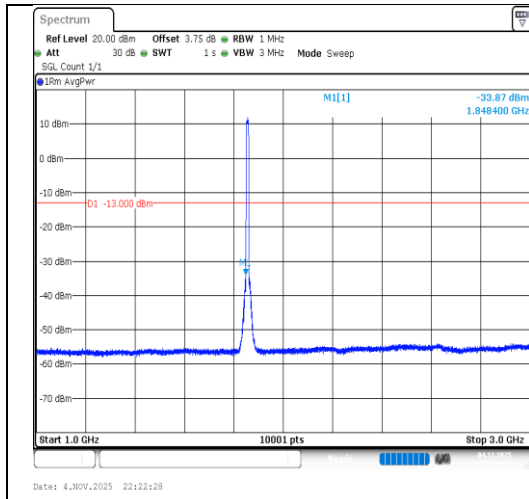
Band2-10MHz-16QAM-18650-50RB#0- 1000~3000-PASS
