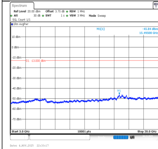
Band2-10MHz-QPSK-19150-1RB#49-3000~20000-PASS
