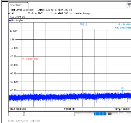
Band2-5MHz-16QAM-19175-1RB#0-30~1000- PASS
