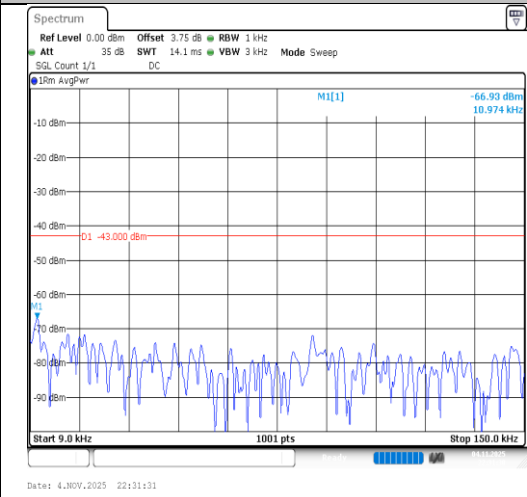
Band2-10MHz-QPSK-19150-50RB#0-0.009~0.15-PASS
