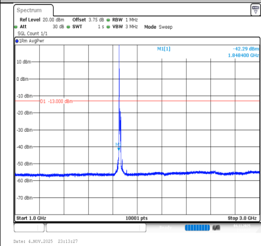
Band2-15MHz-16QAM-18675-1RB#0- 1000~3000-PASS
