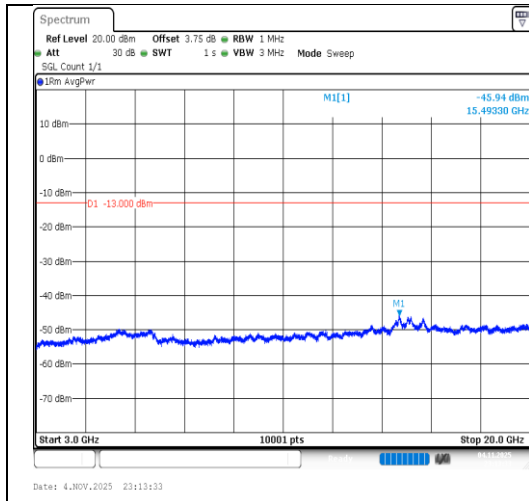
Band2-15MHz-16QAM-18675-1RB#0- 3000~20000-PASS
