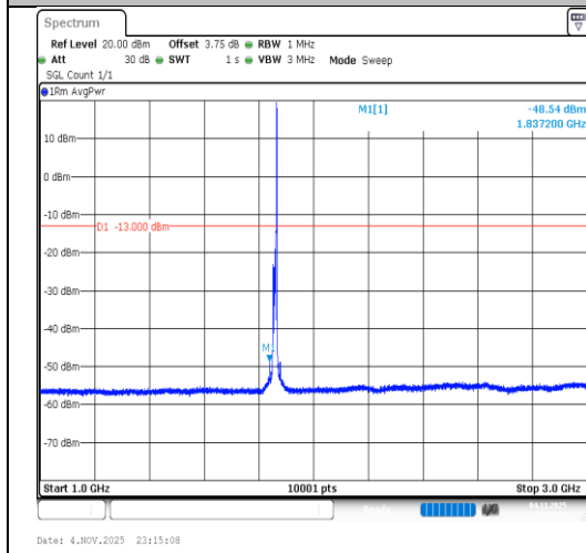
Band2-15MHz-16QAM-18675-1RB#74- 1000~3000-PASS
