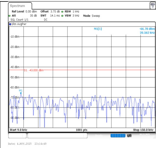
Band2-15MHz-16QAM-18675-1RB#74- 0.009~0.15-PASS
