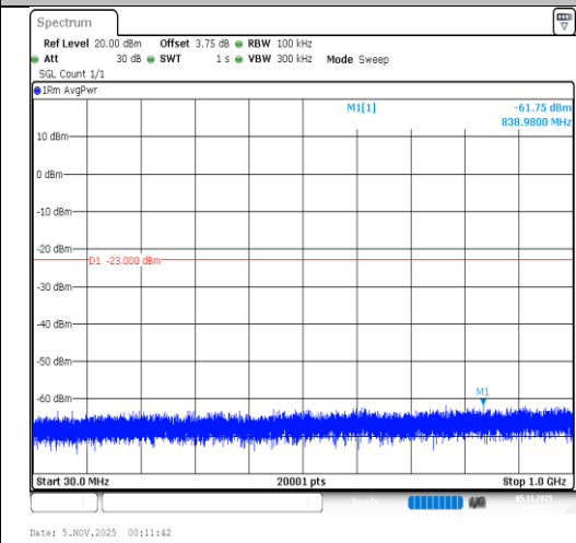
Band2-20MHz-QPSK-18700-100RB#0-30~1000-PASS
