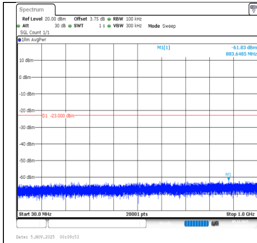
Band2-20MHz-QPSK-18700-1RB#99-30~1000-PASS
