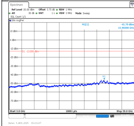
Band2-20MHz-QPSK-18700-1RB#99-3000~20000-PASS
