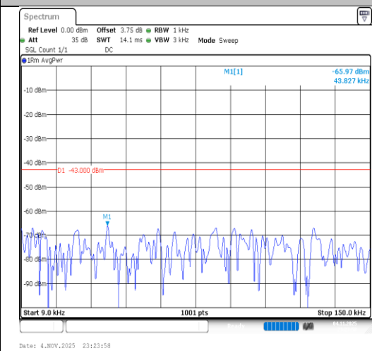
Band2-15MHz-64QAM-19125-1RB#0- 0.009~0.15-PASS
