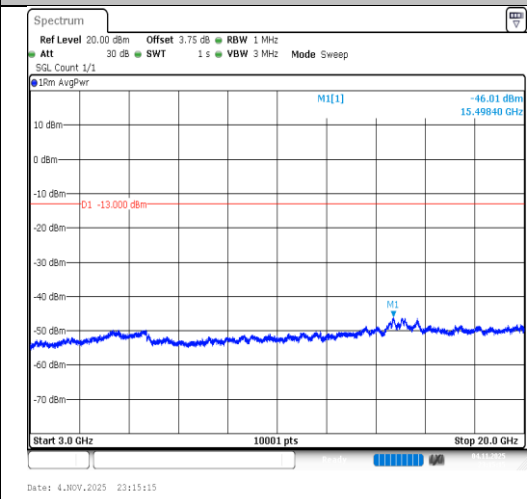
Band2-15MHz-16QAM-18675-1RB#74- 3000~20000-PASS
