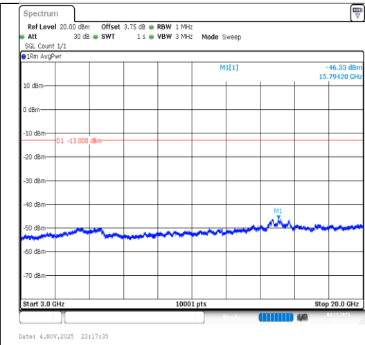
Band2-15MHz-64QAM-18675-75RB#0- 3000~20000-PASS
