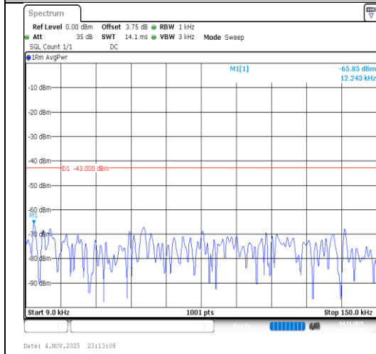
Band2-15MHz-16QAM-18675-1RB#0- 0.009~0.15-PASS
