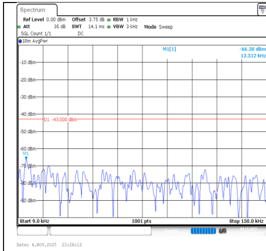
Band2-15MHz-QPSK-19125-75RB#0- 0.009~0.15-PASS
