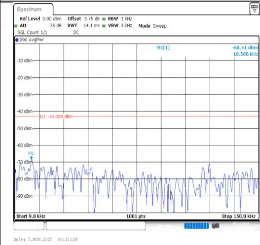
Band2-20MHz-QPSK-18700-100RB#0-0.009~0.15-PASS
