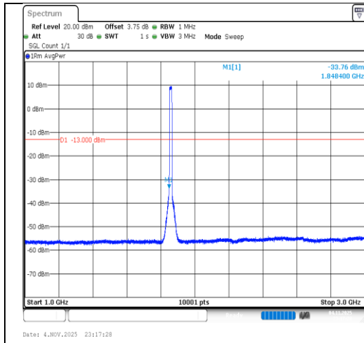
Band2-15MHz-64QAM-18675-75RB#0- 1000~3000-PASS
