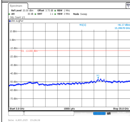
Band2-15MHz-QPSK-19125-75RB#0- 3000~20000-PASS
