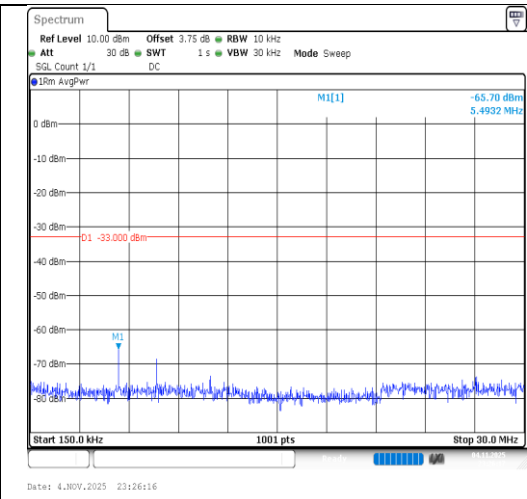
Band2-15MHz-QPSK-19125-75RB#0-0.15~30- PASS
