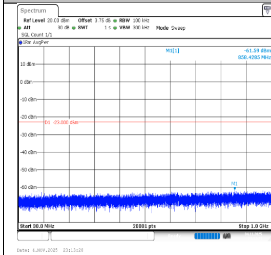
Band2-15MHz-16QAM-18675-1RB#0-30~1000- PASS
