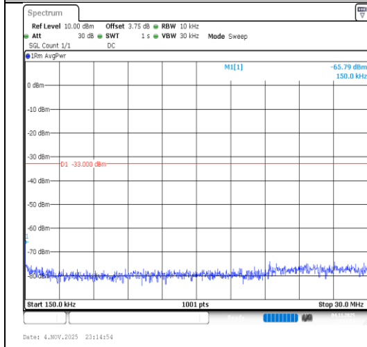
Band2-15MHz-16QAM-18675-1RB#74-0.15~30- PASS
