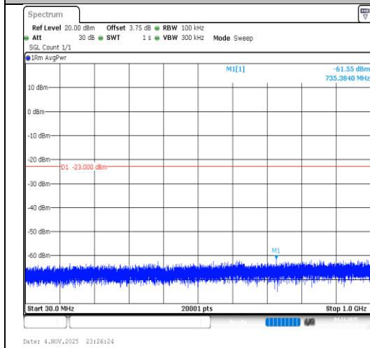
Band2-15MHz-QPSK-19125-75RB#0-30~1000- PASS
