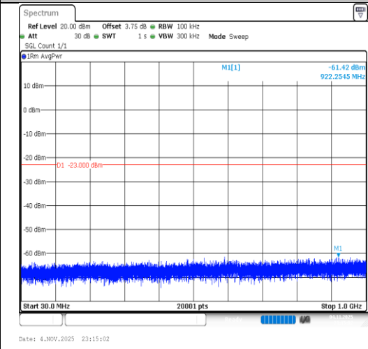
Band2-15MHz-16QAM-18675-1RB#74-30~1000- PASS
