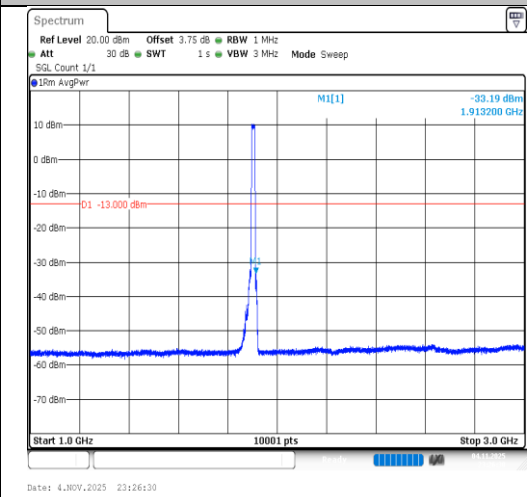
Band2-15MHz-QPSK-19125-75RB#0- 1000~3000-PASS
