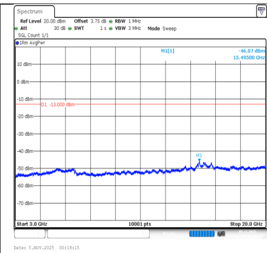
Band2-20MHz-64QAM-18900-100RB#0- 3000~20000-PASS
