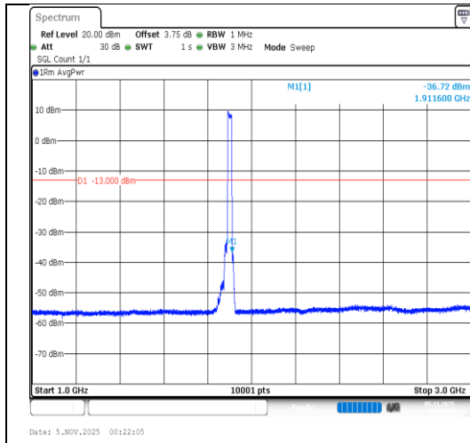
Band2-20MHz-QPSK-19100-100RB#0- 1000~3000-PASS
