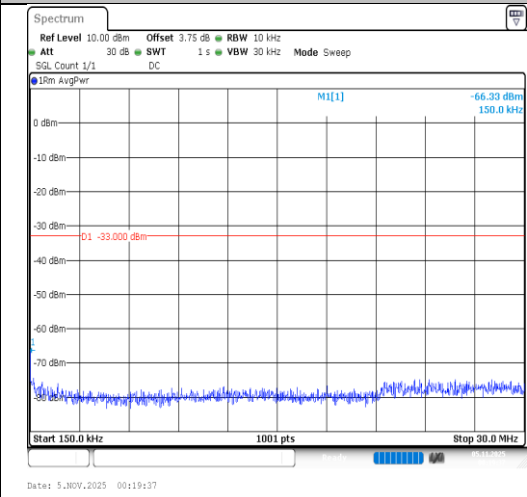
Band2-20MHz-64QAM-19100-1RB#0-0.15~30- PASS
