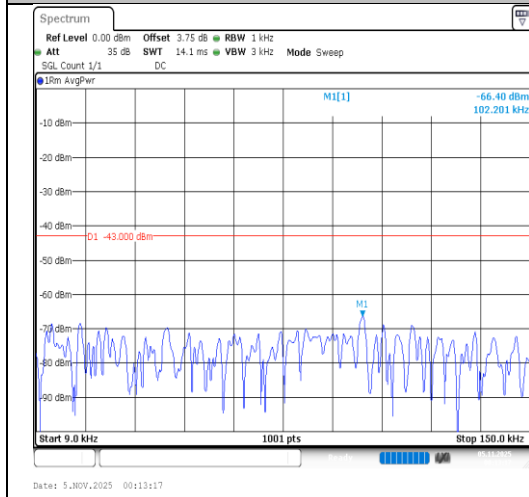
Band2-20MHz-QPSK-18900-1RB#0-0.009~0.15- PASS
