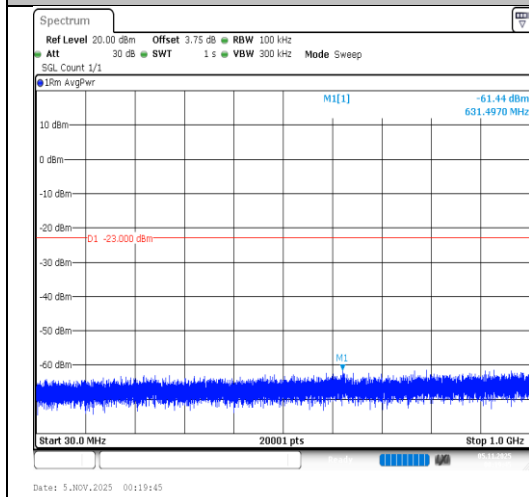
Band2-20MHz-64QAM-19100-1RB#0-30~1000- PASS
