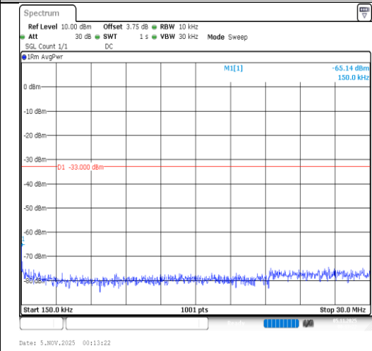
Band2-20MHz-QPSK-18900-1RB#0-0.15~30- PASS
