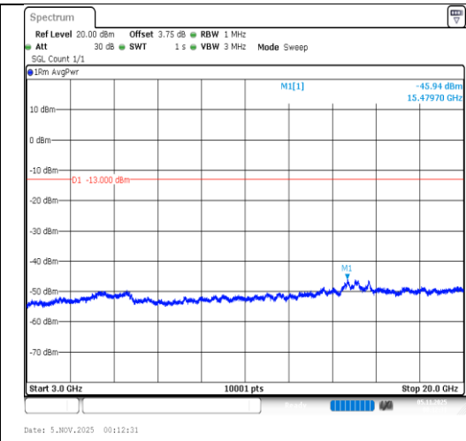
Band2-20MHz-16QAM-18700-100RB#0- 3000~20000-PASS
