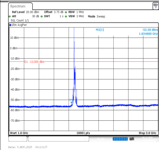
Band2-20MHz-QPSK-18900-1RB#0-1000~3000- PASS
