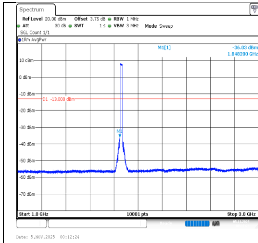
Band2-20MHz-16QAM-18700-100RB#0- 1000~3000-PASS
