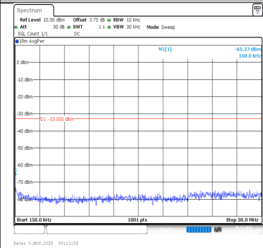
Band2-20MHz-16QAM-18900-1RB#0-0.15~30- PASS
