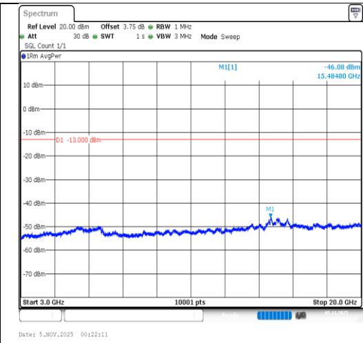
Band2-20MHz-QPSK-19100-100RB#0- 3000~20000-PASS
