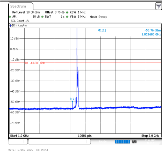
Band2-20MHz-64QAM-19100-1RB#0- 1000~3000-PASS
