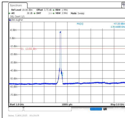
Band2-20MHz-64QAM-18900-100RB#0- 1000~3000-PASS
