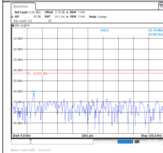
Band2-20MHz-16QAM-18900-1RB#0- 0.009~0.15-PASS
