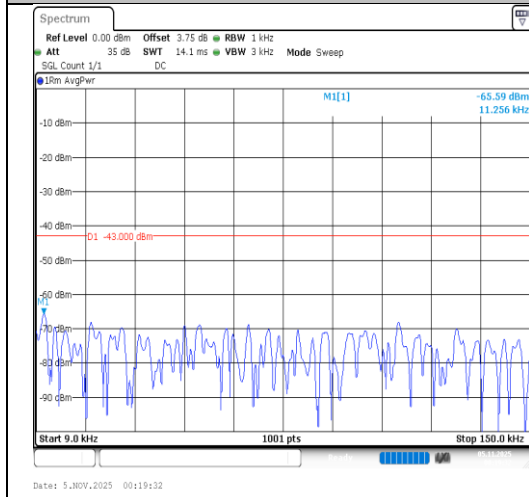
Band2-20MHz-64QAM-19100-1RB#0- 0.009~0.15-PASS
