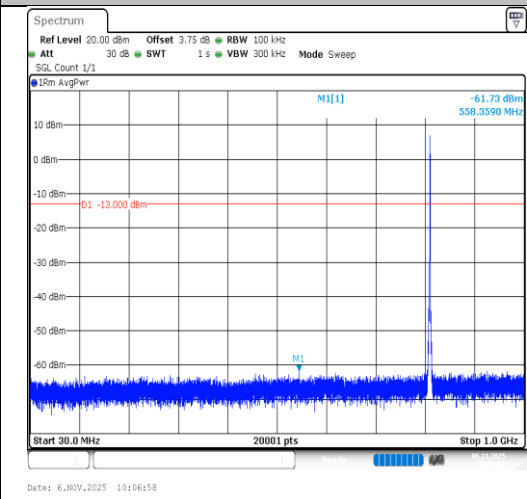
Band26(814-824)-1.4MHz-64QAM-26697- 6RB#0-30~1000-PASS
