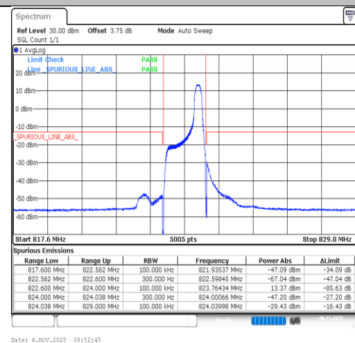
Band26(814-824)-1.4MHz-64QAM-26783-1RB#5-PASS
