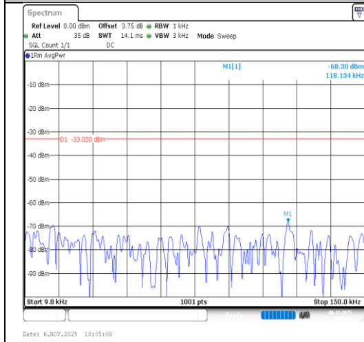
Band26(814-824)-1.4MHz-64QAM-26697- 1RB#5-0.009~0.15-PASS
