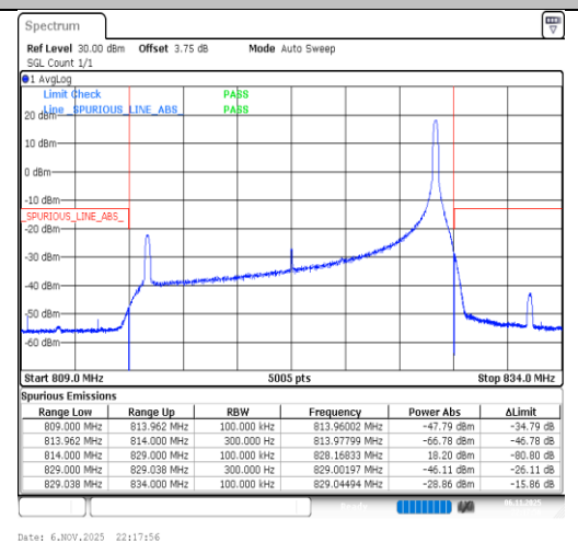
Band26(814-824)-15MHz-64QAM-26765-1RB#74-PASS
