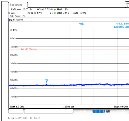
Band26(814-824)-1.4MHz-64QAM-26697- 1RB#0-1000~3000-PASS
