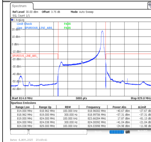
Band26(814-824)-5MHz-16QAM-26765-1RB#24-PASS
