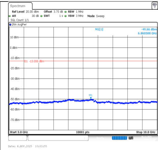
Band26(814-824)-1.4MHz-64QAM-26697- 1RB#0-3000~10000-PASS
