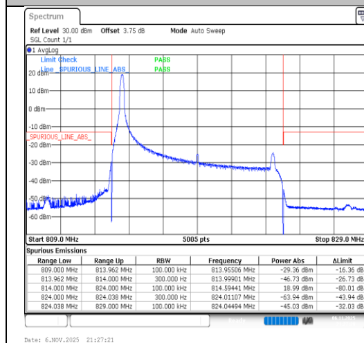
Band26(814-824)-10MHz-QPSK-26740-1RB#0-PASS
