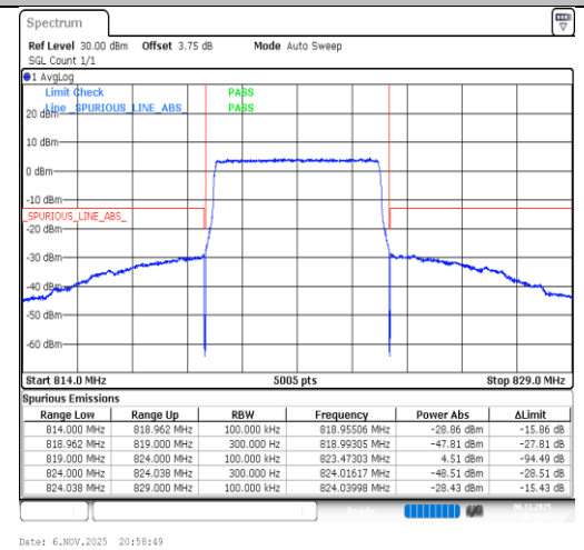
Band26(814-824)-5MHz-16QAM-26765-25RB#0-PASS
