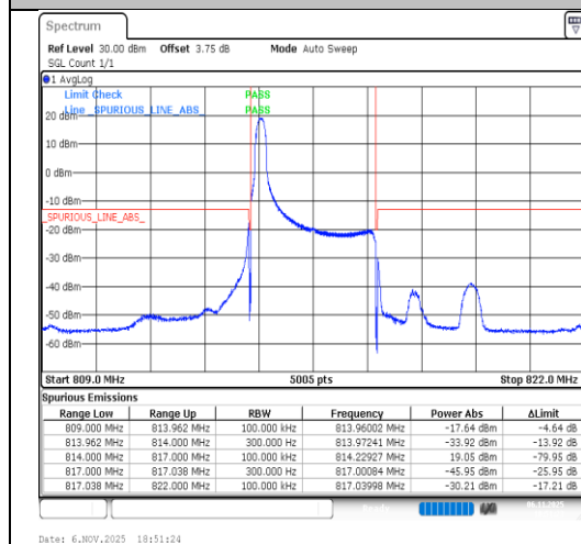
Band26(814-824)-3MHz-QPSK-26705-1RB#0-PASS
