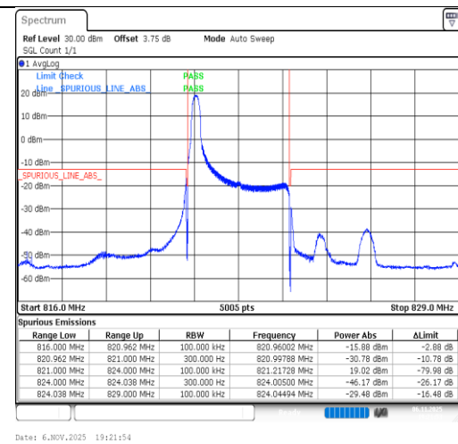
Band26(814-824)-3MHz-16QAM-26775-1RB#0-PASS
