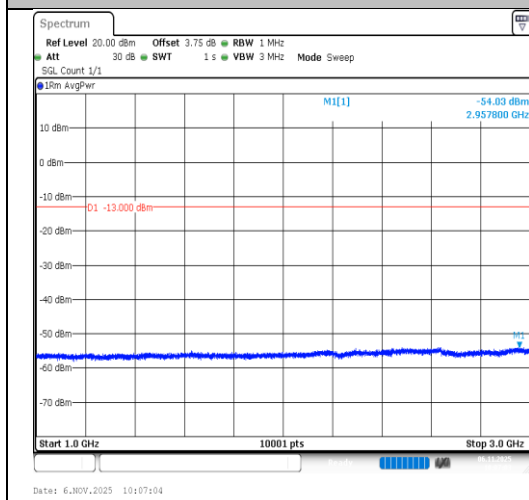
Band26(814-824)-1.4MHz-64QAM-26697- 6RB#0-1000~3000-PASS
