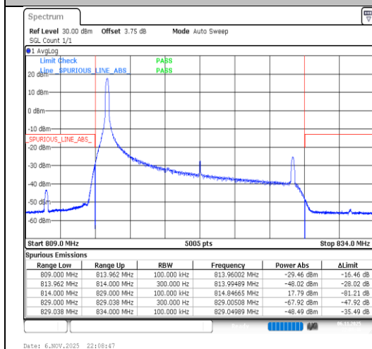
Band26(814-824)-15MHz-64QAM-26765-1RB#0-PASS
