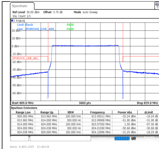
Band26(814-824)-10MHz-16QAM-26740-50RB#0-PASS
