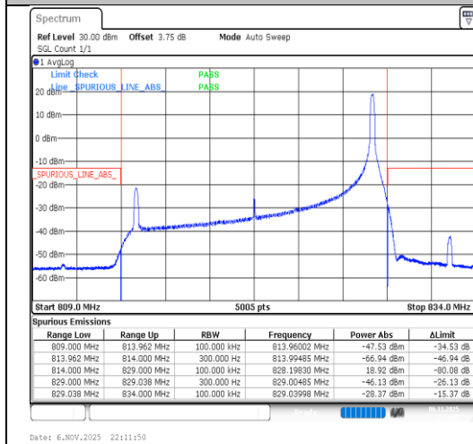
Band26(814-824)-15MHz-QPSK-26765-1RB#74-PASS
