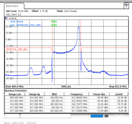
Band26(814-824)-3MHz-QPSK-26705-1RB#14-PASS
