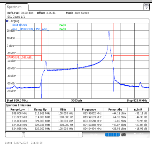
Band26(814-824)-10MHz-QPSK-26740-1RB#49-PASS
