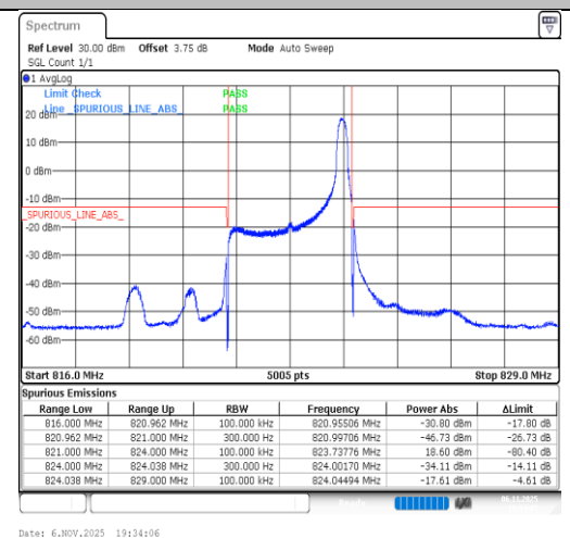
Band26(814-824)-3MHz-64QAM-26775-1RB#14-PASS
