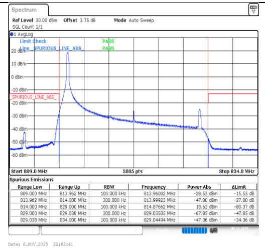
Band26(814-824)-15MHz-QPSK-26765-1RB#0-PASS
