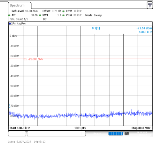
Band26(814-824)-1.4MHz-64QAM-26697- 1RB#5-0.15~30-PASS
