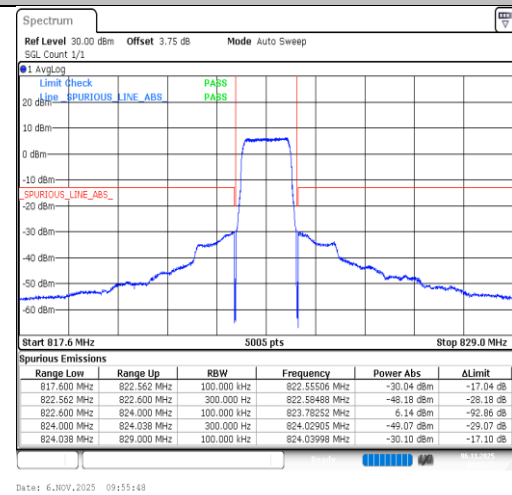
Band26(814-824)-1.4MHz-QPSK-26783-6RB#0-PASS
