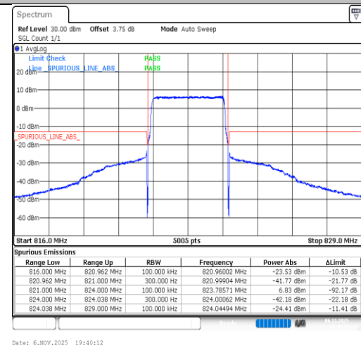
Band26(814-824)-3MHz-16QAM-26775-15RB#0-PASS
