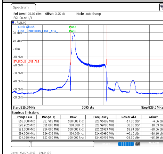
Band26(814-824)-3MHz-64QAM-26775-1RB#0-PASS
