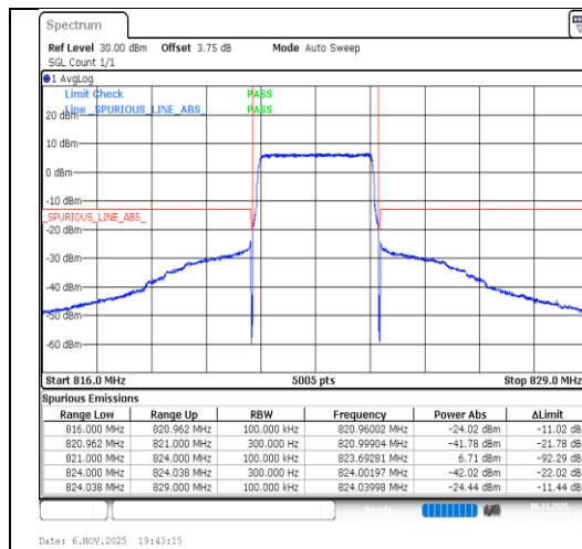
Band26(814-824)-3MHz-64QAM-26775-15RB#0-PASS
