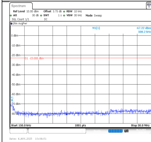
Band26(814-824)-1.4MHz-64QAM-26697- 6RB#0-0.15~30-PASS
