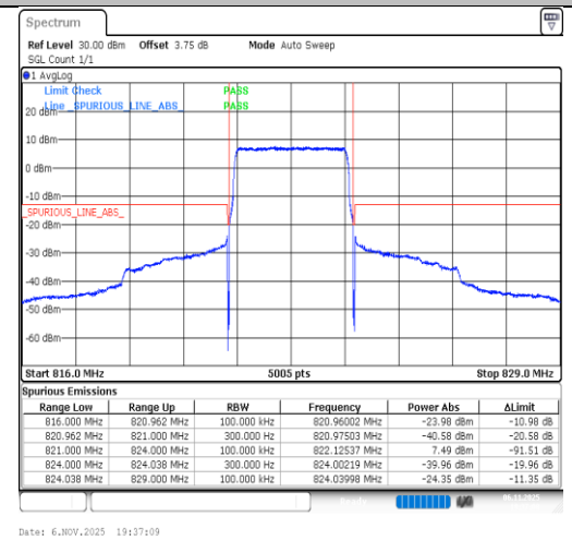
Band26(814-824)-3MHz-QPSK-26775-15RB#0-PASS
