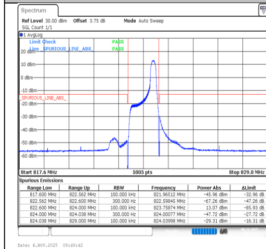
Band26(814-824)-1.4MHz-16QAM-26783-1RB#5-PASS
