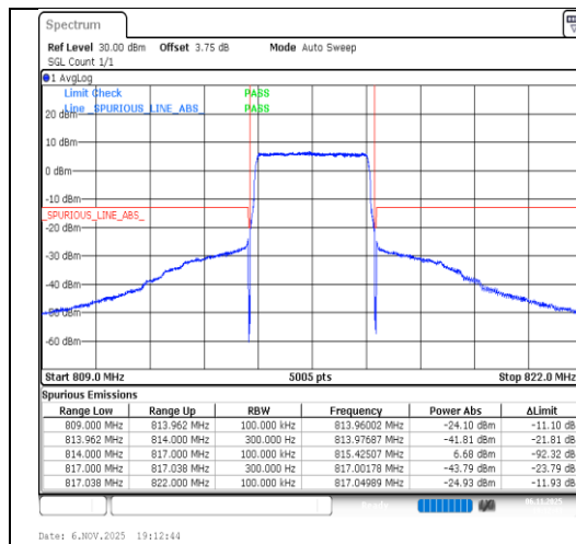
Band26(814-824)-3MHz-16QAM-26705-15RB#0-PASS
