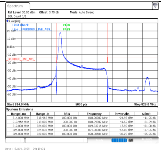
Band26(814-824)-5MHz-16QAM-26765-1RB#0-PASS
