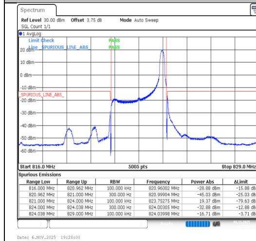
Band26(814-824)-3MHz-QPSK-26775-1RB#14-PASS
