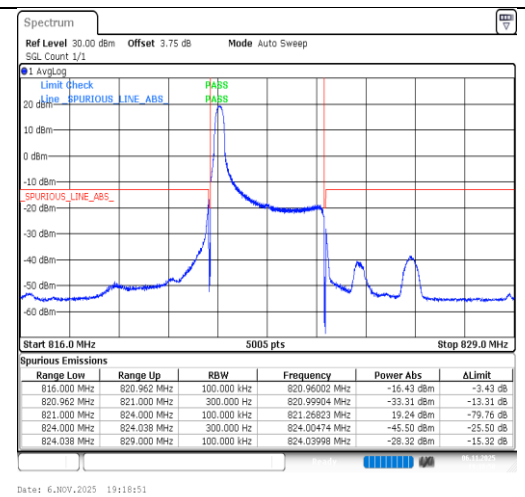
Band26(814-824)-3MHz-QPSK-26775-1RB#0-PASS
