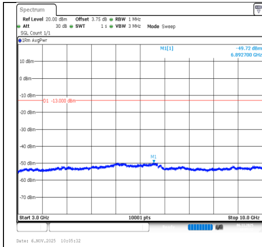
Band26(814-824)-1.4MHz-64QAM-26697- 1RB#5-3000~10000-PASS
