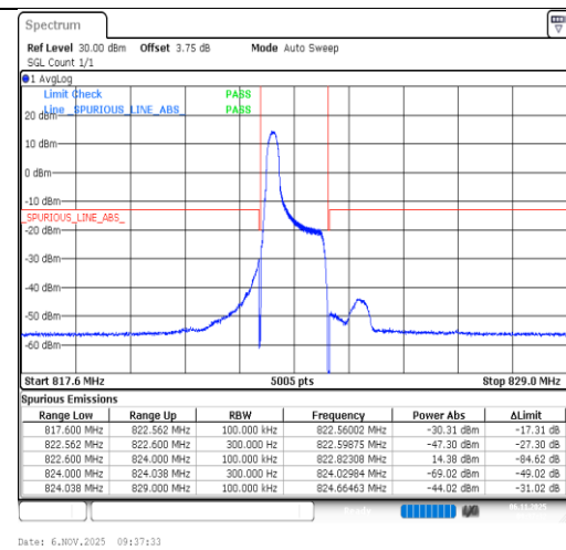
Band26(814-824)-1.4MHz-QPSK-26783-1RB#0-PASS
