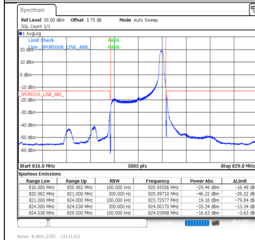
Band26(814-824)-3MHz-16QAM-26775-1RB#14-PASS
