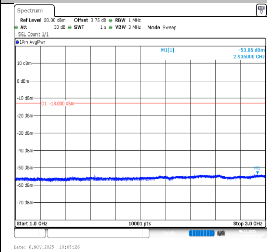
Band26(814-824)-1.4MHz-64QAM-26697- 1RB#5-1000~3000-PASS
