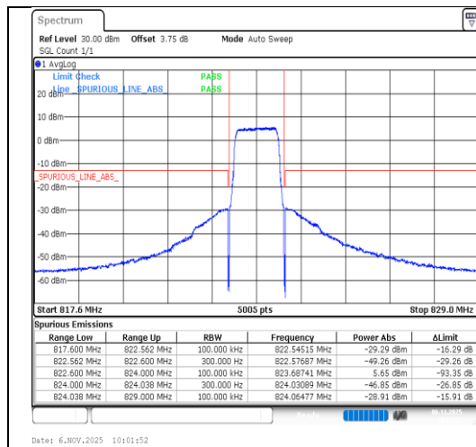
Band26(814-824)-1.4MHz-64QAM-26783-6RB#0-PASS
