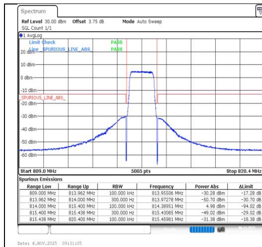
Band26(814-824)-1.4MHz-16QAM-26697-6RB#0-PASS
