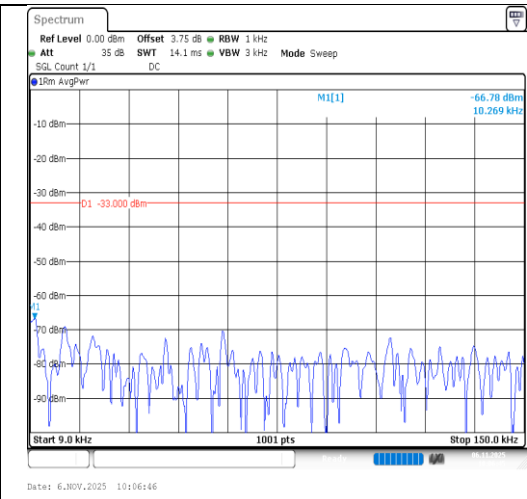
Band26(814-824)-1.4MHz-64QAM-26697- 6RB#0-0.009~0.15-PASS
