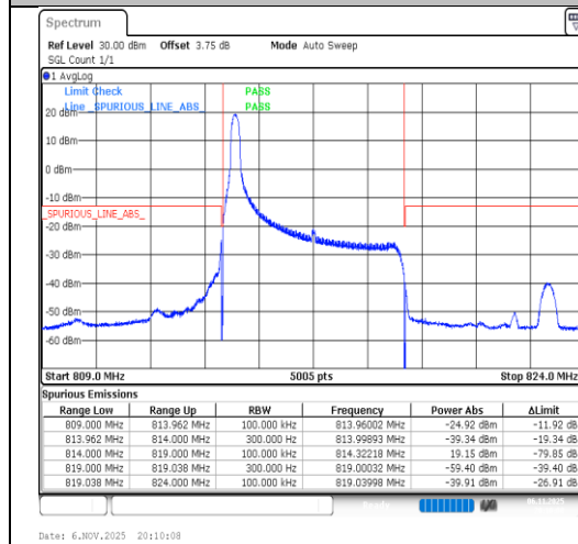
Band26(814-824)-5MHz-QPSK-26715-1RB#0-PASS
