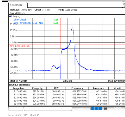
Band26(814-824)-1.4MHz-QPSK-26783-1RB#5-PASS
