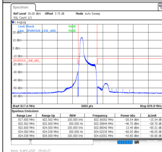
Band26(814-824)-1.4MHz-64QAM-26783-1RB#0-PASS
