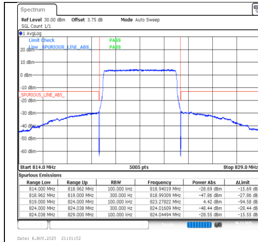
Band26(814-824)-5MHz-64QAM-26765-25RB#0-PASS
