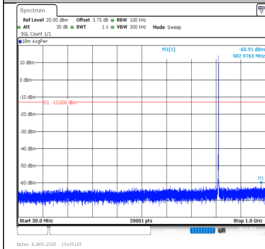
Band26(814-824)-1.4MHz-64QAM-26697- 1RB#5-30~1000-PASS
