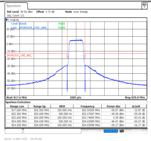
Band26(814-824)-1.4MHz-16QAM-26783-6RB#0-PASS
