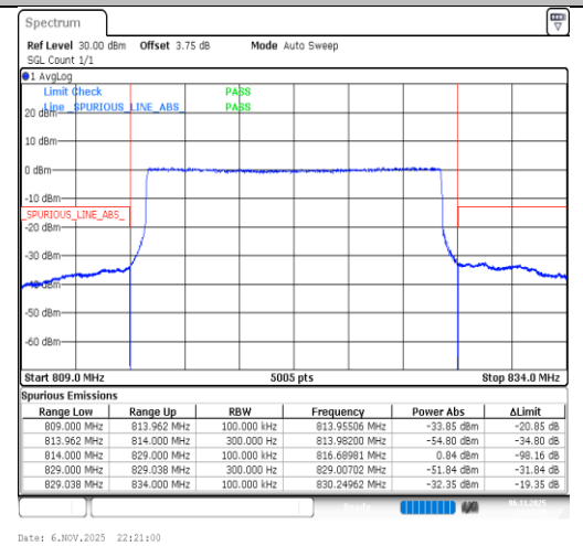
Band26(814-824)-15MHz-QPSK-26765-75RB#0-PASS
