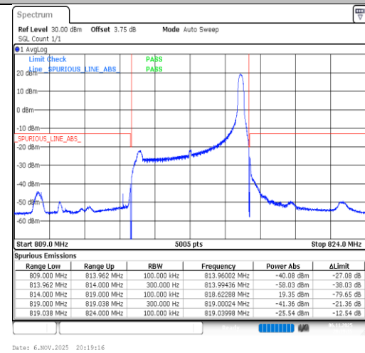
Band26(814-824)-5MHz-QPSK-26715-1RB#24-PASS
