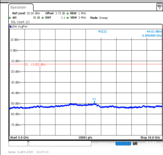
Band26(814-824)-1.4MHz-64QAM-26697- 6RB#0-3000~10000-PASS
