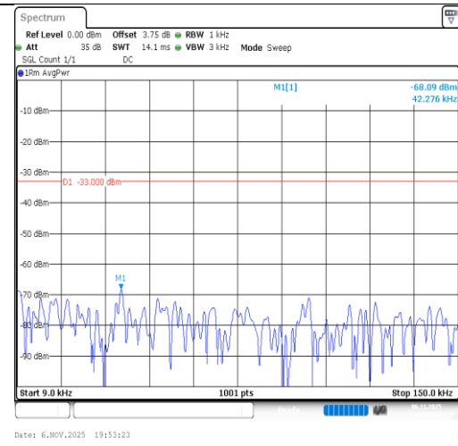
Band26(814-824)-3MHz-64QAM-26740- 15RB#0-0.009~0.15-PASS
