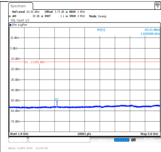
Band26(814-824)-5MHz-QPSK-26715-25RB#0- 1000~3000-PASS
