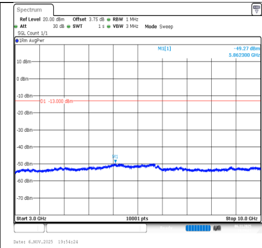
Band26(814-824)-3MHz-QPSK-26775-1RB#0- 3000~10000-PASS
