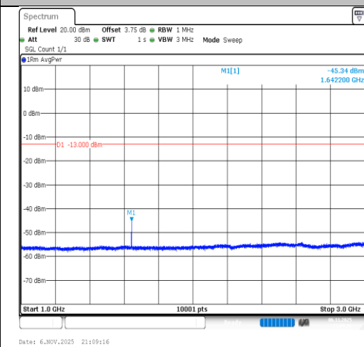
Band26(814-824)-5MHz-QPSK-26740-1RB#24- 1000~3000-PASS
