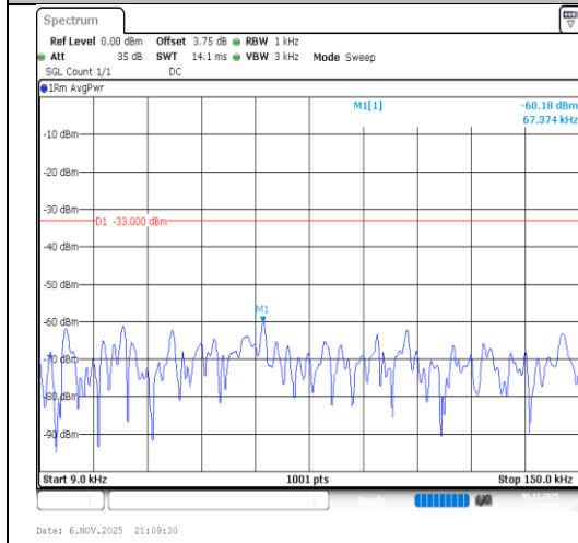
Band26(814-824)-5MHz-16QAM-26740- 1RB#24-0.009~0.15-PASS
