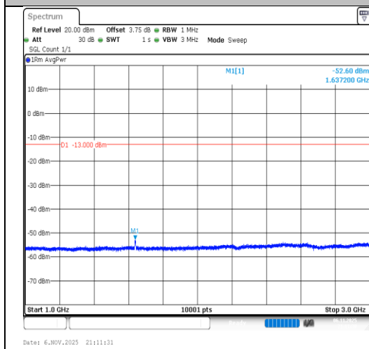
Band26(814-824)-5MHz-16QAM-26740- 25RB#0-1000~3000-PASS
