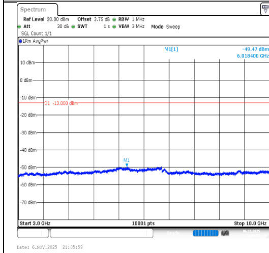
Band26(814-824)-5MHz-QPSK-26715-25RB#0- 3000~10000-PASS
