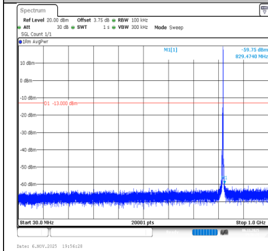
Band26(814-824)-3MHz-16QAM-26775- 1RB#14-30~1000-PASS
