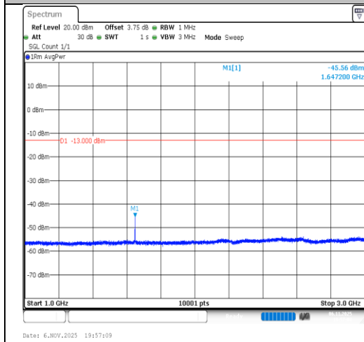
Band26(814-824)-3MHz-64QAM-26775- 1RB#14-1000~3000-PASS
