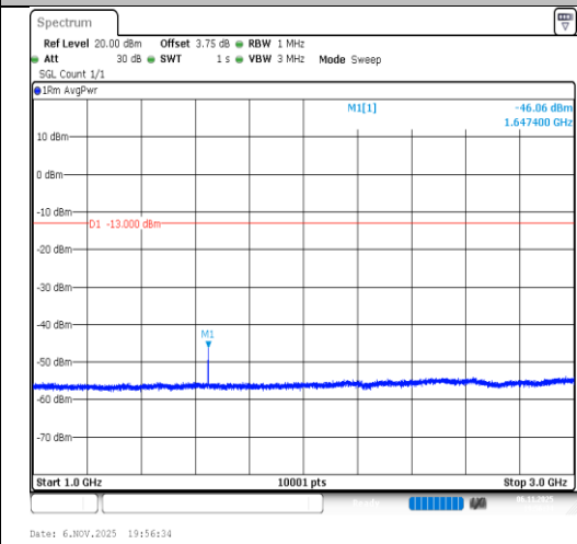
Band26(814-824)-3MHz-16QAM-26775- 1RB#14-1000~3000-PASS
