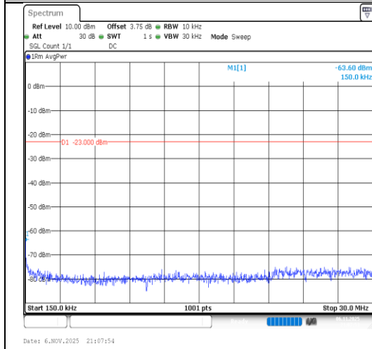
Band26(814-824)-5MHz-16QAM-26740-1RB#0- 0.15~30-PASS
