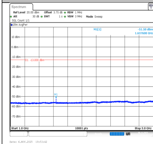
Band26(814-824)-3MHz-64QAM-26740- 15RB#0-1000~3000-PASS
