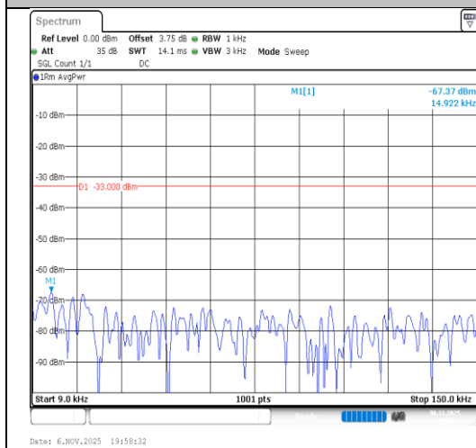
Band26(814-824)-3MHz-64QAM-26775- 15RB#0-0.009~0.15-PASS
