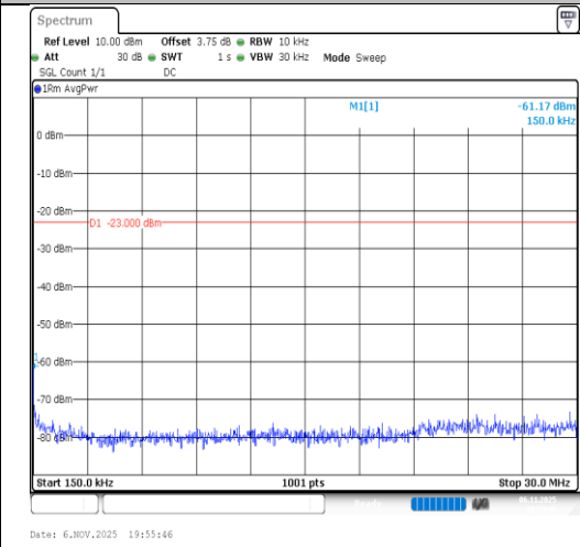
Band26(814-824)-3MHz-QPSK-26775-1RB#14- 0.15~30-PASS
