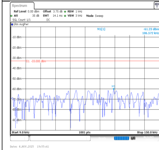
Band26(814-824)-3MHz-QPSK-26775-1RB#14- 0.009~0.15-PASS
