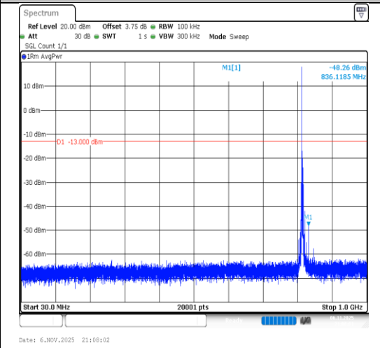
Band26(814-824)-5MHz-16QAM-26740-1RB#0- 30~1000-PASS
