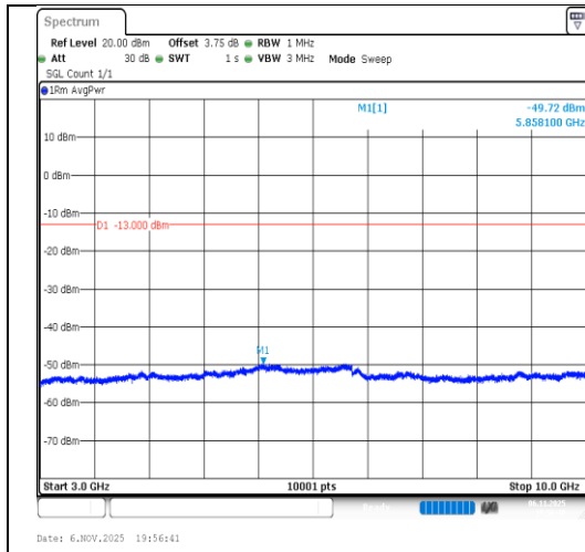
Band26(814-824)-3MHz-16QAM-26775- 1RB#14-3000~10000-PASS
