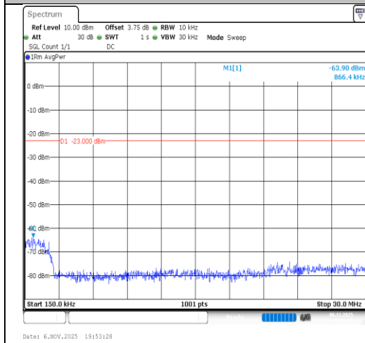
Band26(814-824)-3MHz-64QAM-26740- 15RB#0-0.15~30-PASS
