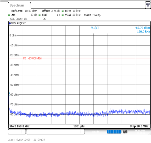
Band26(814-824)-5MHz-16QAM-26740- 1RB#24-0.15~30-PASS
