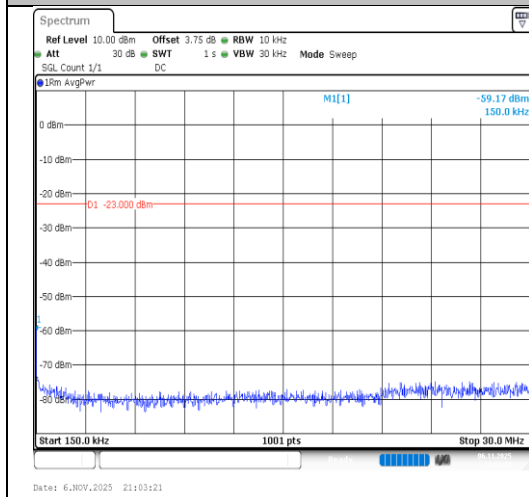
Band26(814-824)-5MHz-64QAM-26715-1RB#0- 0.15~30-PASS
