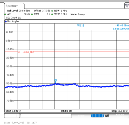
Band26(814-824)-5MHz-16QAM-26740- 25RB#0-3000~10000-PASS
