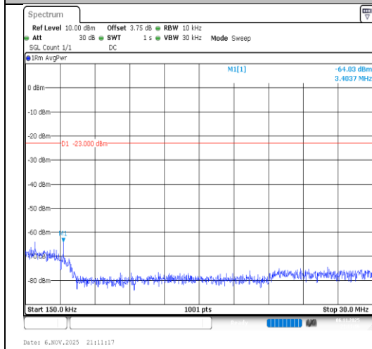
Band26(814-824)-5MHz-16QAM-26740- 25RB#0-0.15~30-PASS
