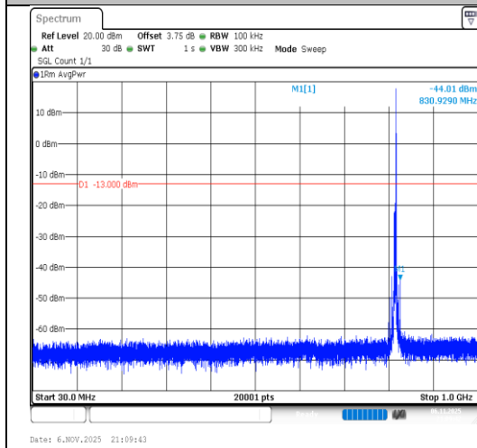
Band26(814-824)-5MHz-16QAM-26740- 1RB#24-30~1000-PASS
