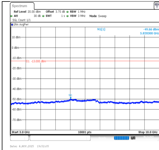
Band26(814-824)-3MHz-64QAM-26740- 1RB#14-3000~10000-PASS
