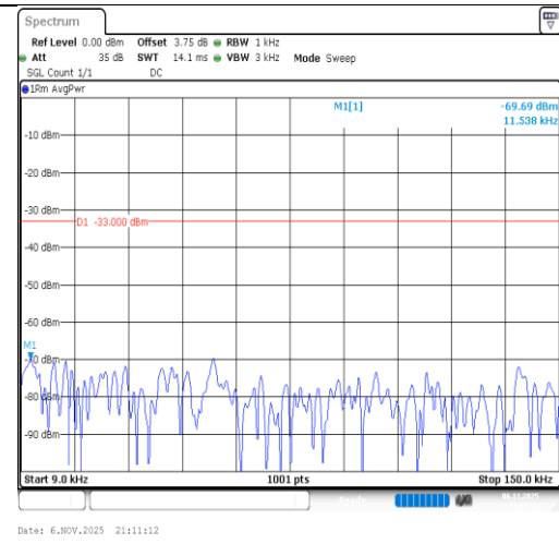
Band26(814-824)-5MHz-16QAM-26740- 25RB#0-0.009~0.15-PASS
