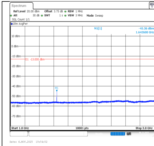
Band26(814-824)-3MHz-16QAM-26775-1RB#0- 1000~3000-PASS
