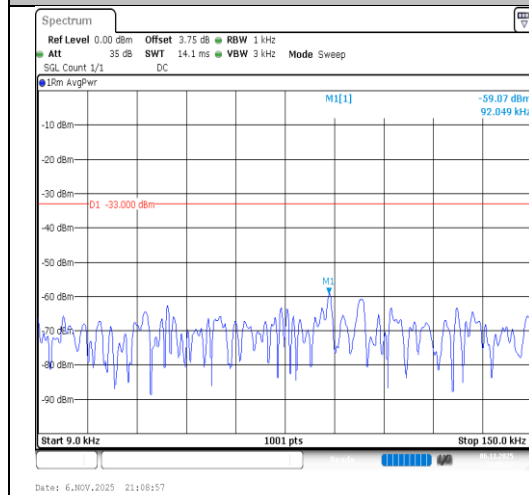
Band26(814-824)-5MHz-QPSK-26740-1RB#24- 0.009~0.15-PASS
