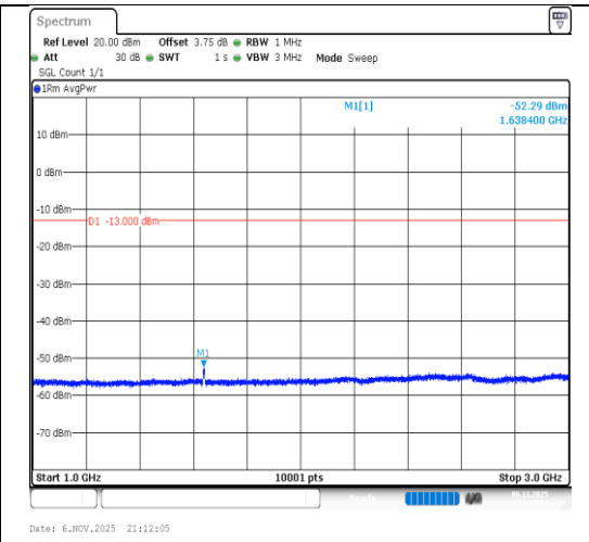
Band26(814-824)-5MHz-64QAM-26740- 25RB#0-1000~3000-PASS
