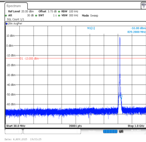
Band26(814-824)-3MHz-64QAM-26740- 15RB#0-30~1000-PASS
