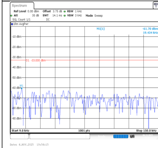
Band26(814-824)-3MHz-16QAM-26775- 1RB#14-0.009~0.15-PASS
