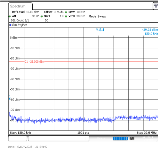
Band26(814-824)-5MHz-QPSK-26740-1RB#24- 0.15~30-PASS
