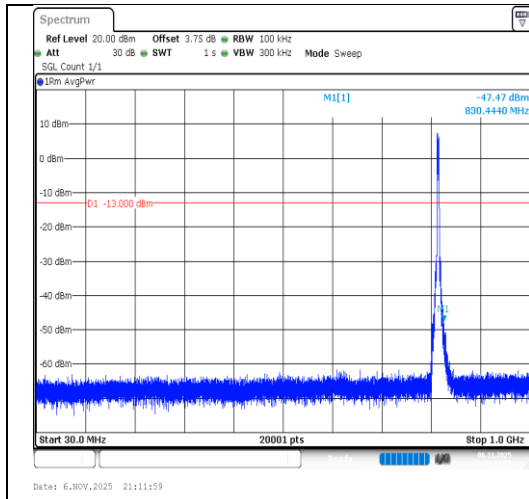
Band26(814-824)-5MHz-64QAM-26740- 25RB#0-30~1000-PASS
