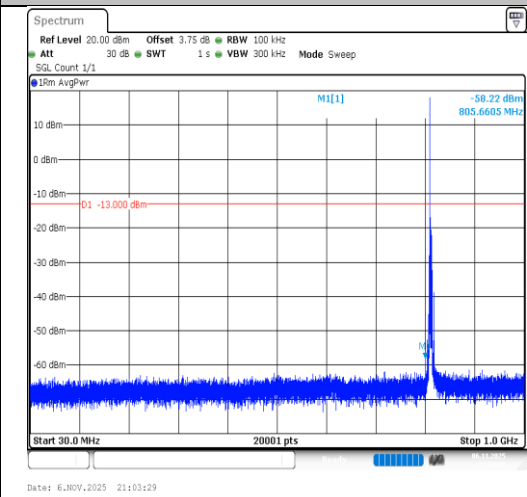
Band26(814-824)-5MHz-64QAM-26715-1RB#0- 30~1000-PASS
