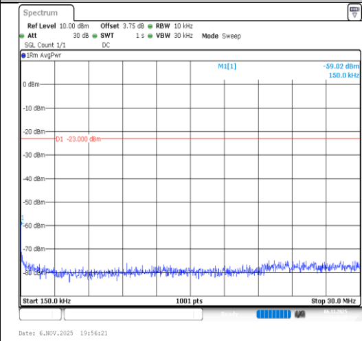
Band26(814-824)-3MHz-16QAM-26775- 1RB#14-0.15~30-PASS
