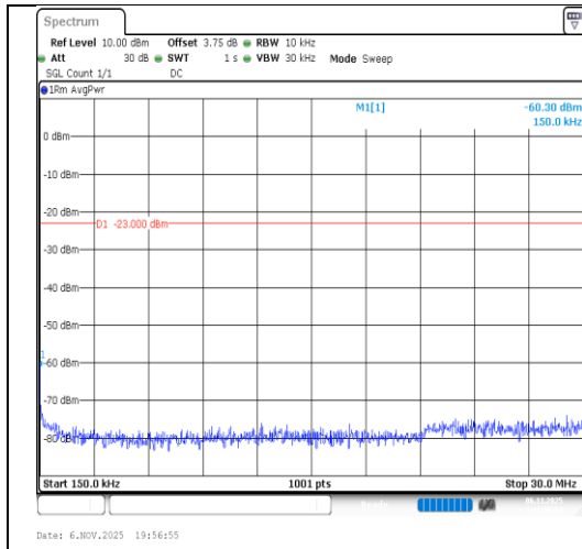
Band26(814-824)-3MHz-64QAM-26775- 1RB#14-0.15~30-PASS
