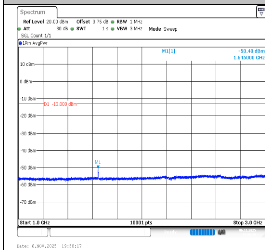
Band26(814-824)-3MHz-16QAM-26775- 15RB#0-1000~3000-PASS
