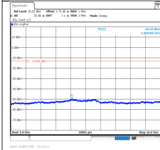
Band26(814-824)-5MHz-64QAM-26740- 25RB#0-3000~10000-PASS
