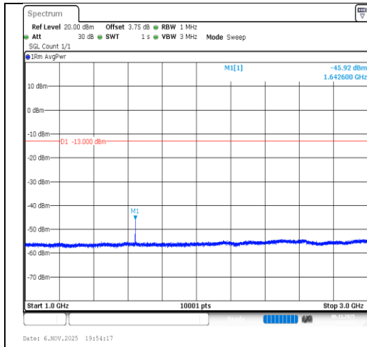
Band26(814-824)-3MHz-QPSK-26775-1RB#0- 1000~3000-PASS
