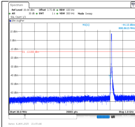
Band26(814-824)-5MHz-QPSK-26715-25RB#0- 30~1000-PASS
