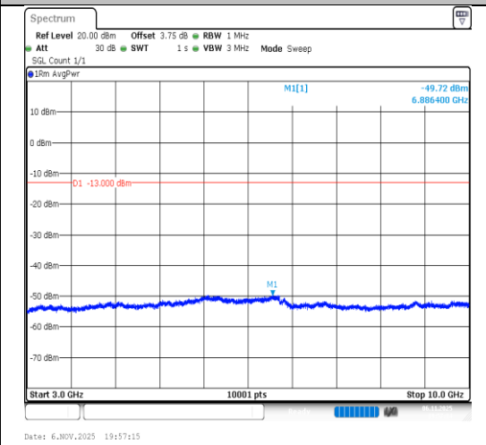
Band26(814-824)-3MHz-64QAM-26775- 1RB#14-3000~10000-PASS
