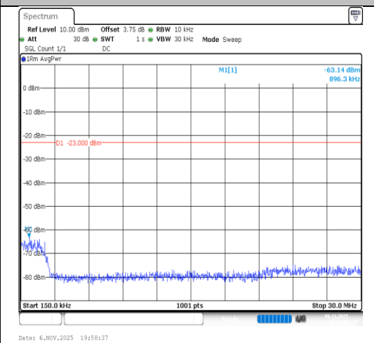
Band26(814-824)-3MHz-64QAM-26775- 15RB#0-0.15~30-PASS
