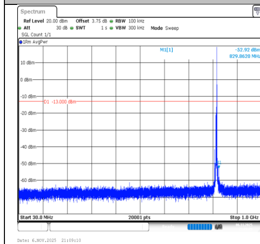
Band26(814-824)-5MHz-QPSK-26740-1RB#24- 30~1000-PASS
