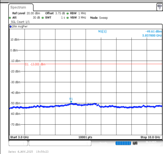
Band26(814-824)-3MHz-16QAM-26775- 15RB#0-3000~10000-PASS
