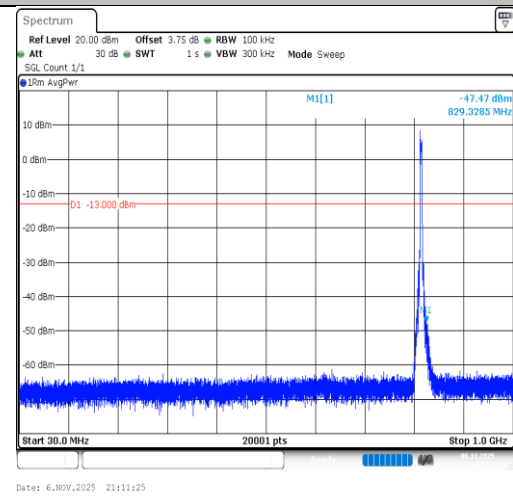
Band26(814-824)-5MHz-16QAM-26740- 25RB#0-30~1000-PASS
