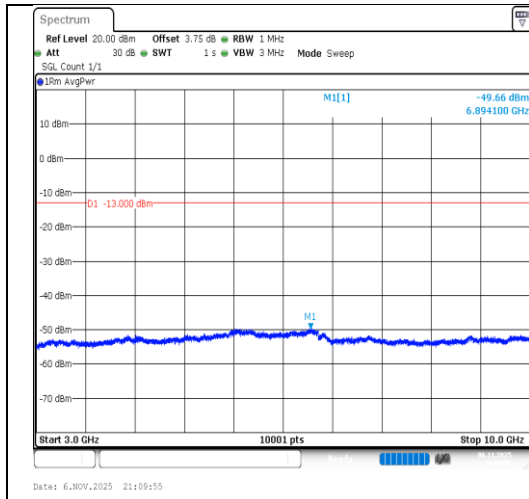
Band26(814-824)-5MHz-16QAM-26740- 1RB#24-3000~10000-PASS
