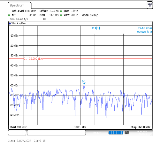
Band26(814-824)-5MHz-64QAM-26715-1RB#0- 0.009~0.15-PASS
