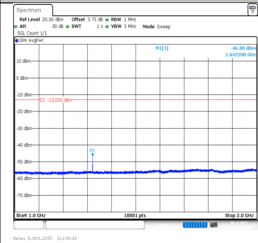
Band26(814-824)-5MHz-16QAM-26740- 1RB#24-1000~3000-PASS
