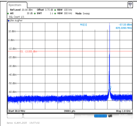
Band26(814-824)-3MHz-64QAM-26775- 1RB#14-30~1000-PASS
