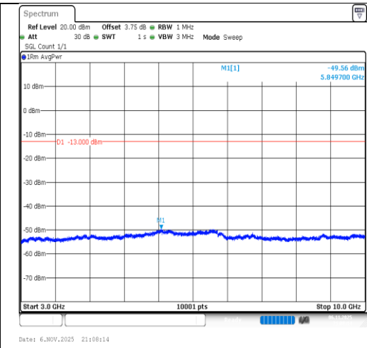
Band26(814-824)-5MHz-16QAM-26740-1RB#0- 3000~10000-PASS
