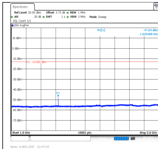
Band26(814-824)-5MHz-QPSK-26740-1RB#0- 1000~3000-PASS
