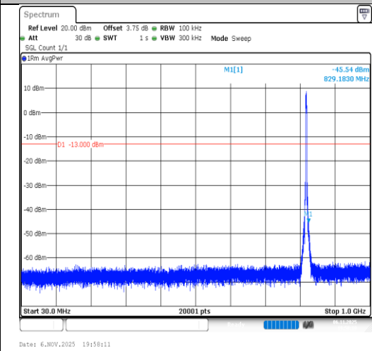
Band26(814-824)-3MHz-16QAM-26775- 15RB#0-30~1000-PASS
