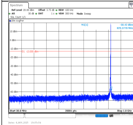
Band26(814-824)-3MHz-QPSK-26775-1RB#14- 30~1000-PASS
