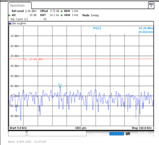
Band26(814-824)-5MHz-16QAM-26740-1RB#0- 0.009~0.15-PASS
