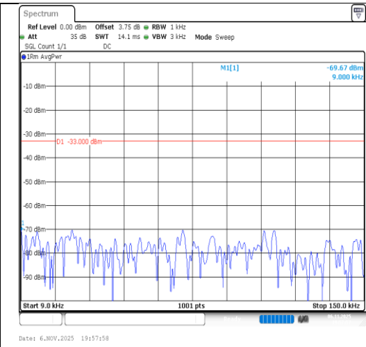
Band26(814-824)-3MHz-16QAM-26775- 15RB#0-0.009~0.15-PASS
