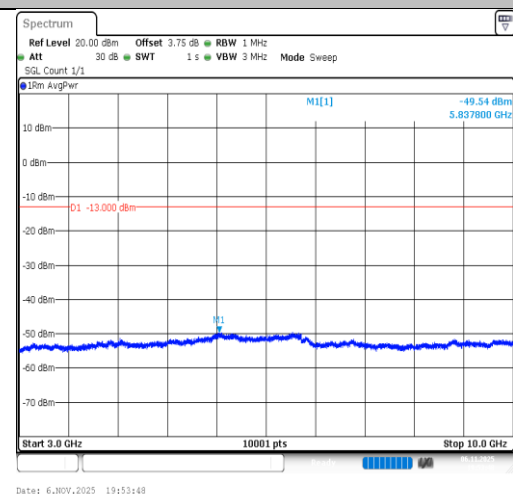
Band26(814-824)-3MHz-64QAM-26740- 15RB#0-3000~10000-PASS
