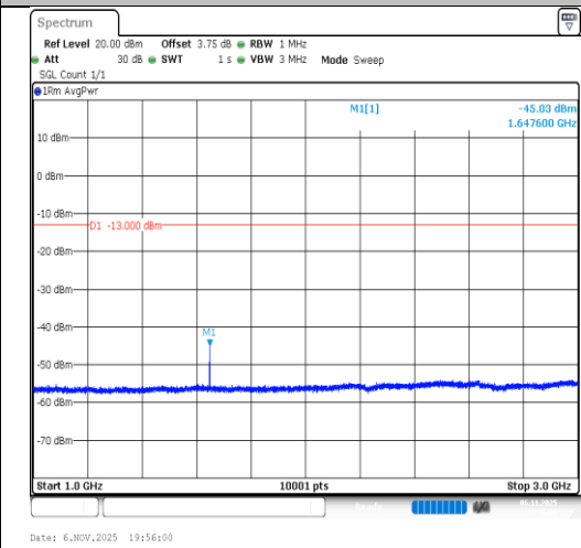
Band26(814-824)-3MHz-QPSK-26775-1RB#14- 1000~3000-PASS
