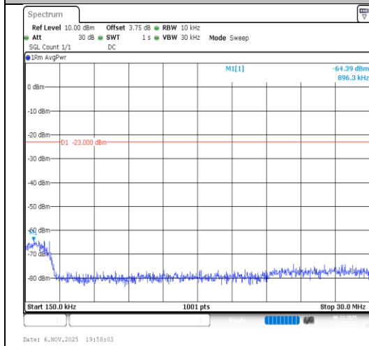
Band26(814-824)-3MHz-16QAM-26775- 15RB#0-0.15~30-PASS
