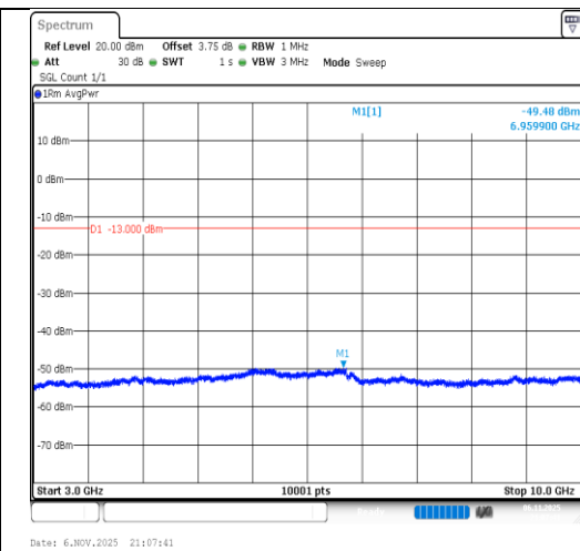
Band26(814-824)-5MHz-QPSK-26740-1RB#0- 3000~10000-PASS
