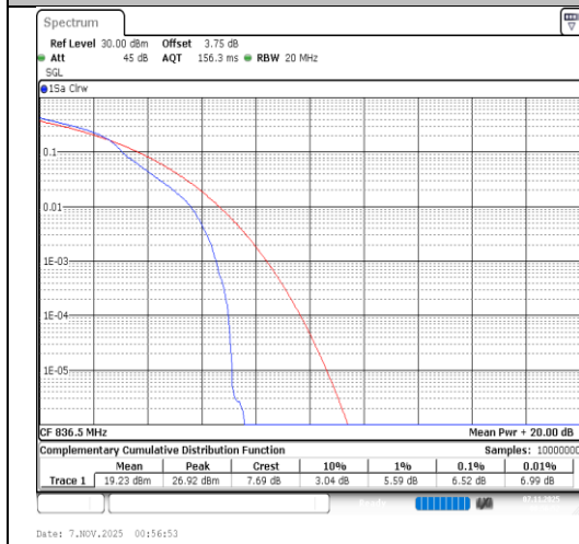
Band26(824-849)-15MHz-16QAM-26915- 1RB#0-PASS
