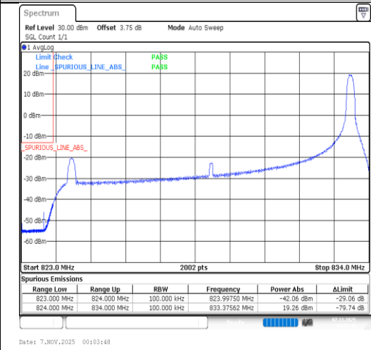
Band26(824-849)-10MHz-QPSK-26840-1RB#49-PASS
