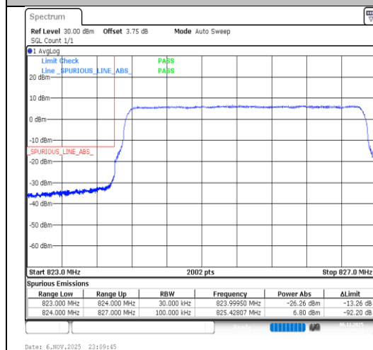
Band26(824-849)-3MHz-16QAM-26805-15RB#0-PASS
