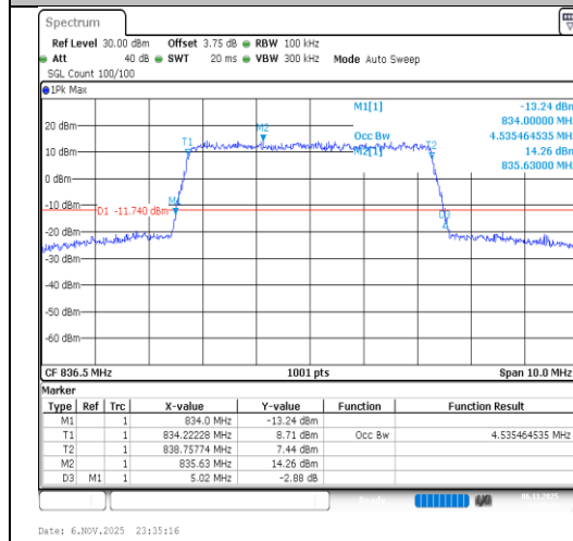
Band26(824-849)-5MHz-64QAM-26915- 25RB#0-PASS
