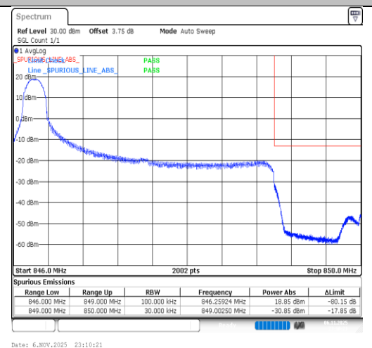
Band26(824-849)-3MHz-16QAM-27025-1RB#0-PASS
