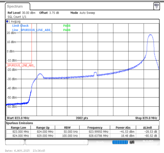
Band26(824-849)-5MHz-16QAM-26815-1RB#24-PASS
