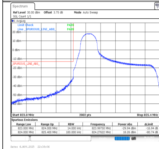
Band26(824-849)-1.4MHz-16QAM-26797- 1RB#0-PASS
