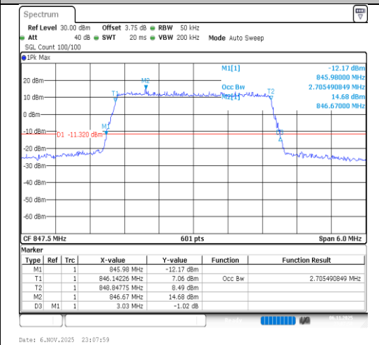
Band26(824-849)-3MHz-16QAM-27025-15RB#0-PASS
