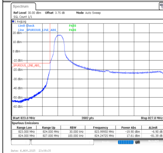
Band26(824-849)-3MHz-16QAM-26805-1RB#0-PASS
