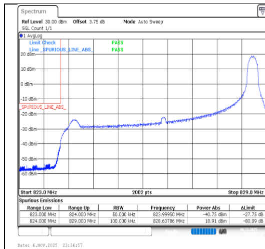
Band26(824-849)-5MHz-64QAM-26815-1RB#24-PASS
