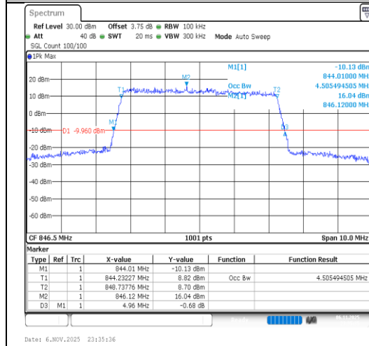
Band26(824-849)-5MHz-16QAM-27015- 25RB#0-PASS
