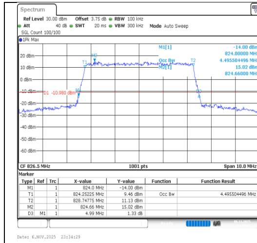
Band26(824-849)-5MHz-QPSK-26815-25RB#0- PASS
