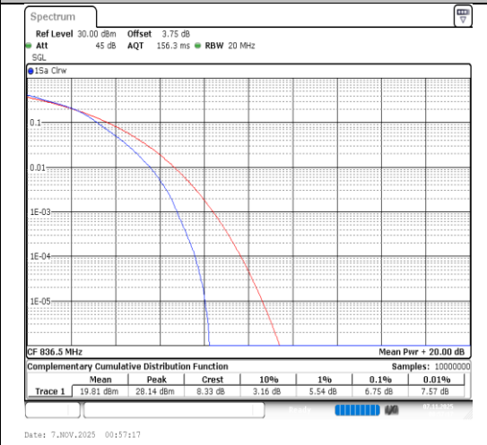
Band26(824-849)-15MHz-64QAM-26915- 75RB#0-PASS
