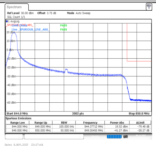
Band26(824-849)-5MHz-QPSK-27015-1RB#0-PASS
