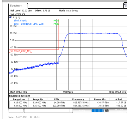
Band26(824-849)-1.4MHz-16QAM-26797- 6RB#0-PASS
