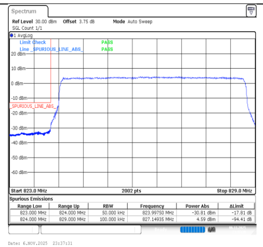
Band26(824-849)-5MHz-64QAM-26815-25RB#0-PASS
