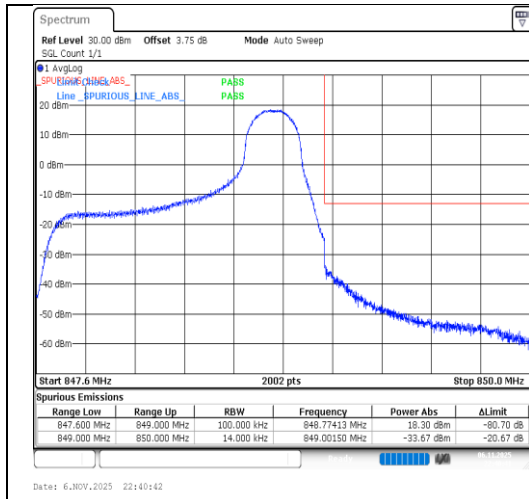
Band26(824-849)-1.4MHz-16QAM-27033-1RB#5-PASS
