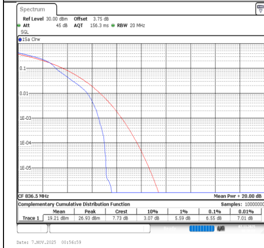
Band26(824-849)-15MHz-64QAM-26915- 1RB#0-PASS
