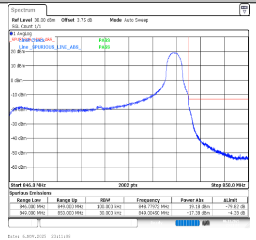
Band26(824-849)-3MHz-64QAM-27025-1RB#14-PASS
