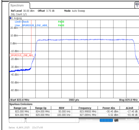
Band26(824-849)-5MHz-QPSK-26815-25RB#0-PASS
