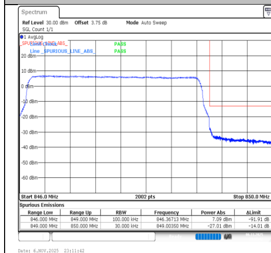
Band26(824-849)-3MHz-64QAM-27025-15RB#0-PASS
