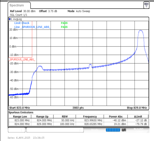
Band26(824-849)-5MHz-QPSK-26815-1RB#24-PASS
