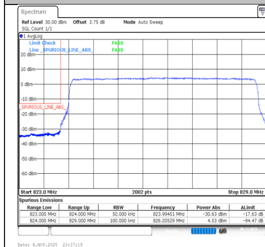
Band26(824-849)-5MHz-16QAM-26815-25RB#0-PASS
