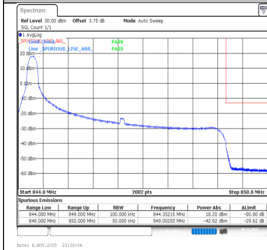
Band26(824-849)-5MHz-64QAM-27015-1RB#0-PASS
