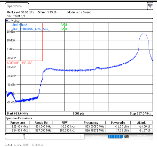
Band26(824-849)-3MHz-16QAM-26805-1RB#14-PASS
