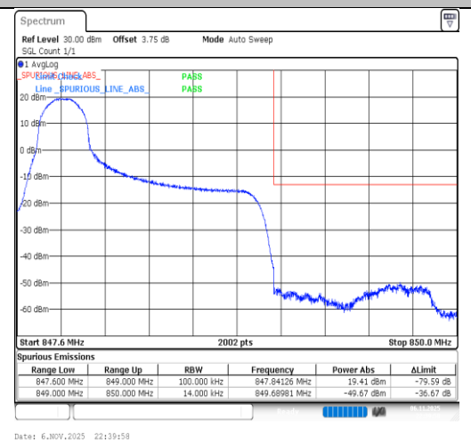
Band26(824-849)-1.4MHz-QPSK-27033-1RB#0- PASS
