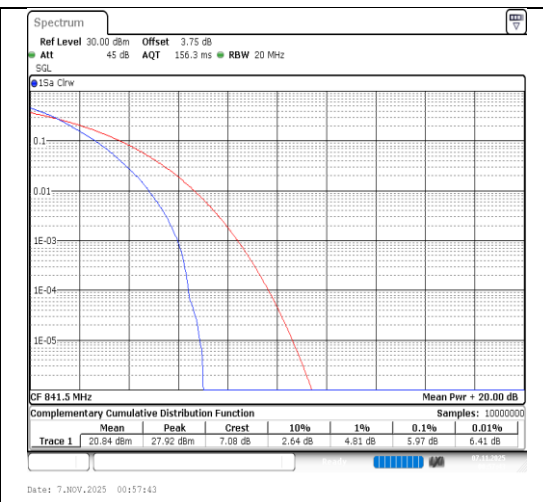
Band26(824-849)-15MHz-QPSK-26965-75RB#0- PASS
