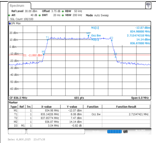
Band26(824-849)-3MHz-64QAM-26915-15RB#0-PASS
