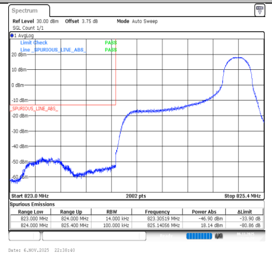
Band26(824-849)-1.4MHz-16QAM-26797- 1RB#5-PASS
