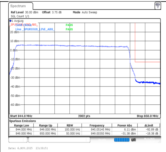
Band26(824-849)-5MHz-QPSK-27015-25RB#0-PASS
