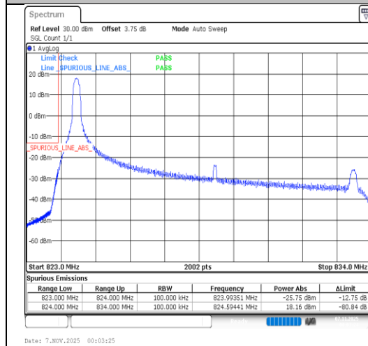
Band26(824-849)-10MHz-16QAM-26840-1RB#0-PASS
