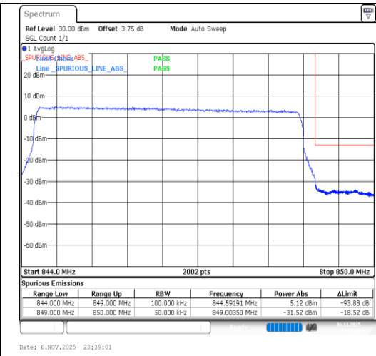
Band26(824-849)-5MHz-16QAM-27015-25RB#0-PASS
