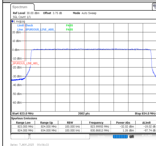
Band26(824-849)-10MHz-16QAM-26840-50RB#0-PASS
