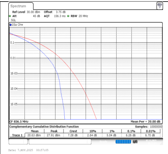
Band26(824-849)-15MHz-QPSK-26915-75RB#0- PASS
