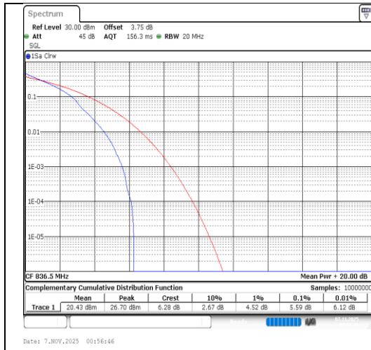
Band26(824-849)-15MHz-QPSK-26915-1RB#0- PASS
