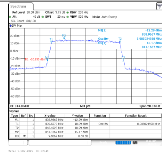
Band26(824-849)-10MHz-16QAM-26990-50RB#0-PASS
