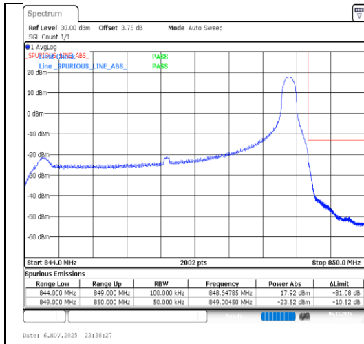
Band26(824-849)-5MHz-16QAM-27015-1RB#24-PASS
