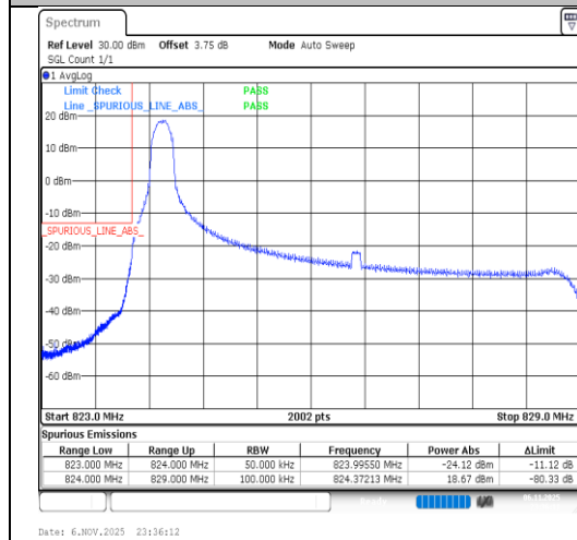
Band26(824-849)-5MHz-16QAM-26815-1RB#0-PASS
