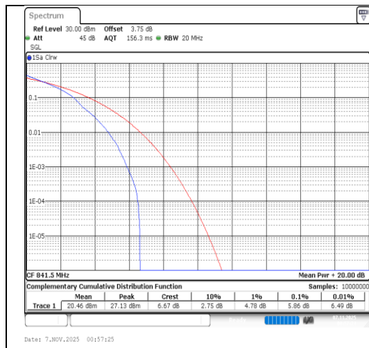
Band26(824-849)-15MHz-QPSK-26965-1RB#0- PASS
