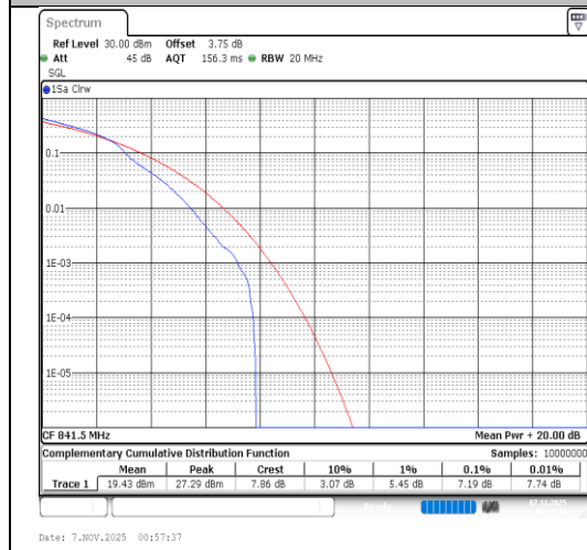
Band26(824-849)-15MHz-64QAM-26965- 1RB#0-PASS
