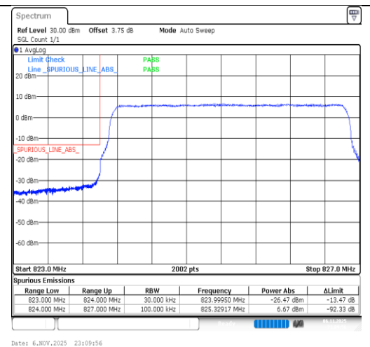
Band26(824-849)-3MHz-64QAM-26805-15RB#0-PASS
