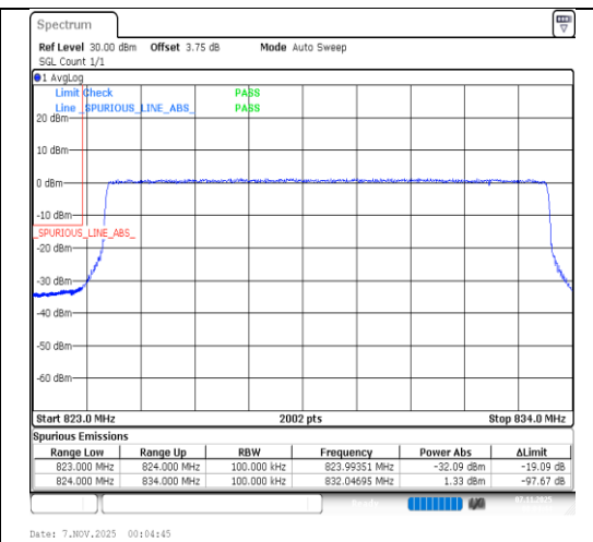
Band26(824-849)-10MHz-64QAM-26840-50RB#0-PASS
