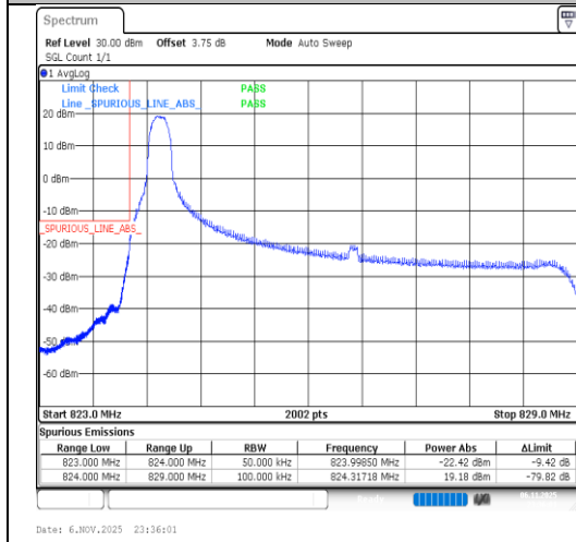
Band26(824-849)-5MHz-QPSK-26815-1RB#0-PASS
