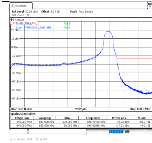
Band26(824-849)-3MHz-16QAM-27025-1RB#14-PASS
