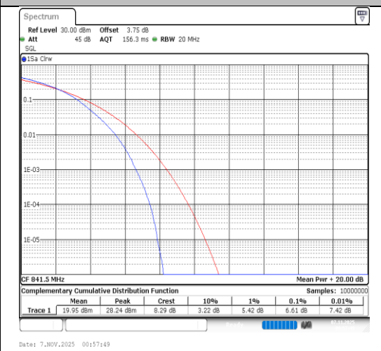
Band26(824-849)-15MHz-16QAM-26965- 75RB#0-PASS
