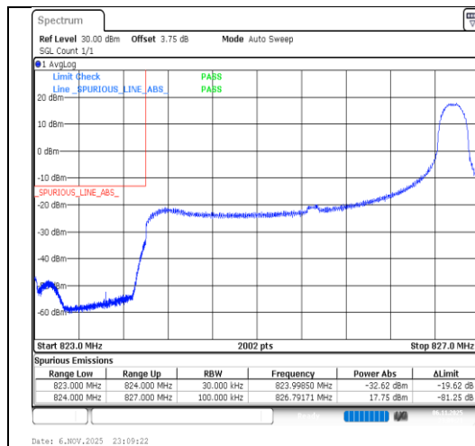
Band26(824-849)-3MHz-64QAM-26805-1RB#14-PASS
