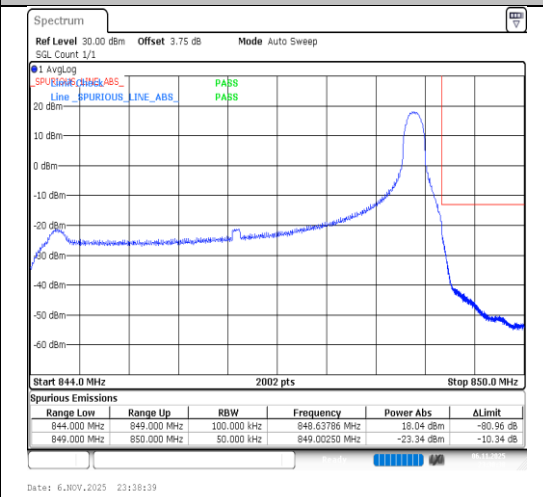
Band26(824-849)-5MHz-64QAM-27015-1RB#24-PASS
