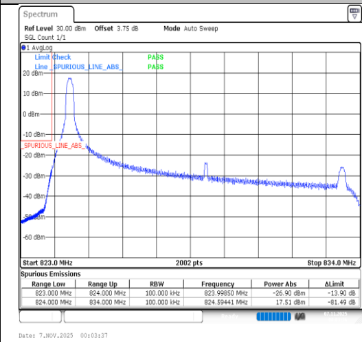
Band26(824-849)-10MHz-64QAM-26840-1RB#0-PASS
