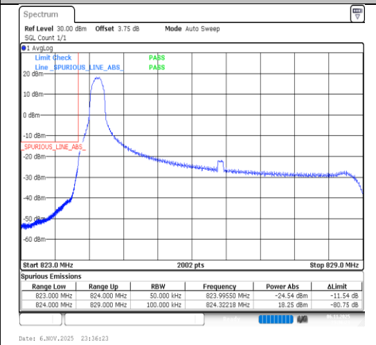
Band26(824-849)-5MHz-64QAM-26815-1RB#0-PASS
