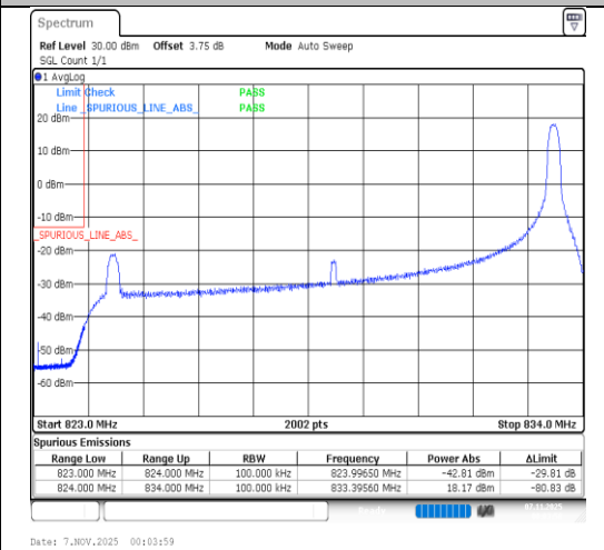
Band26(824-849)-10MHz-16QAM-26840-1RB#49-PASS
