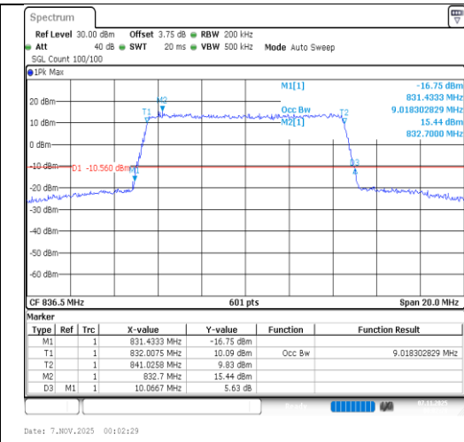
Band26(824-849)-10MHz-64QAM-26915-50RB#0-PASS
