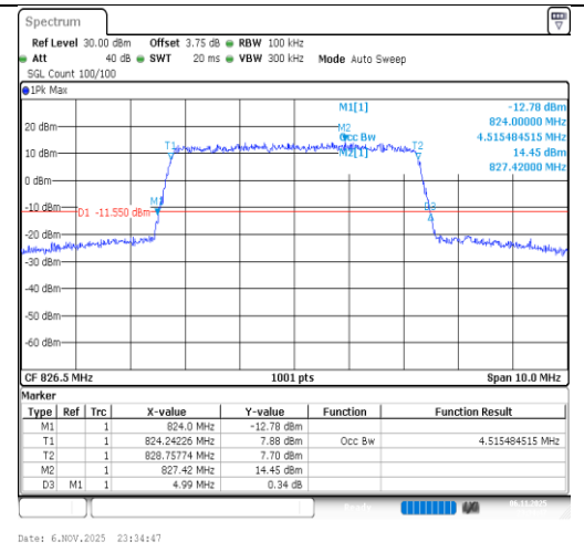
Band26(824-849)-5MHz-64QAM-26815- 25RB#0-PASS
