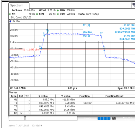
Band26(824-849)-10MHz-64QAM-26990-50RB#0-PASS
