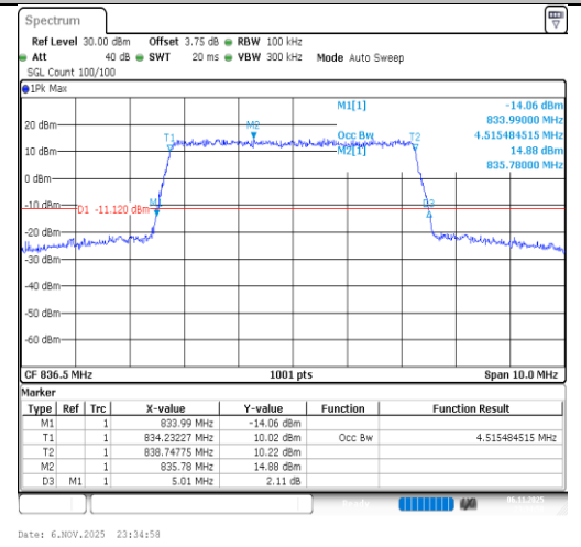
Band26(824-849)-5MHz-QPSK-26915-25RB#0- PASS
