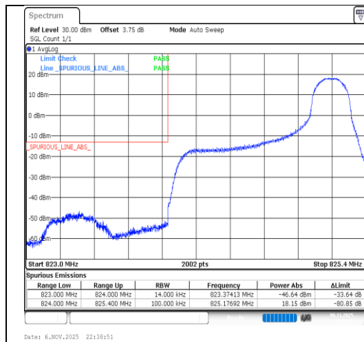
Band26(824-849)-1.4MHz-64QAM-26797- 1RB#5-PASS
