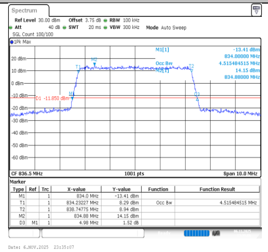
Band26(824-849)-5MHz-16QAM-26915- 25RB#0-PASS
