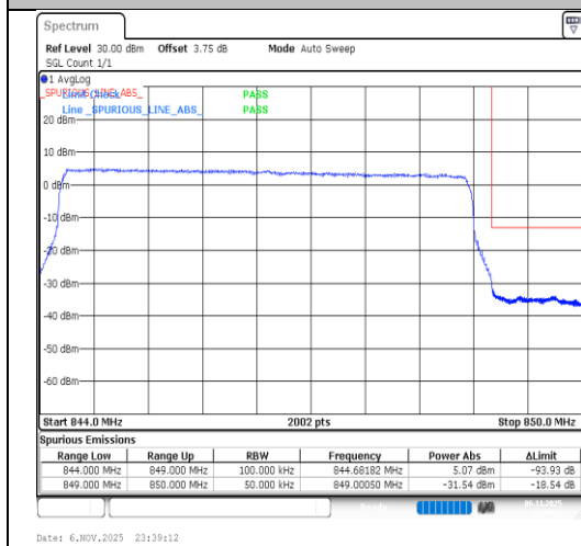
Band26(824-849)-5MHz-64QAM-27015-25RB#0-PASS
