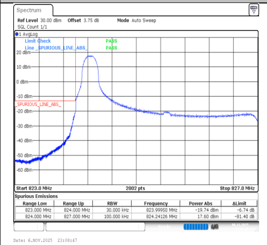
Band26(824-849)-3MHz-64QAM-26805-1RB#0-PASS
