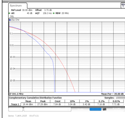
Band26(824-849)-15MHz-16QAM-26965- 1RB#0-PASS
