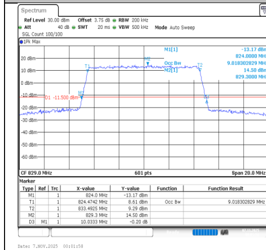
Band26(824-849)-10MHz-64QAM-26840- 50RB#0-PASS
