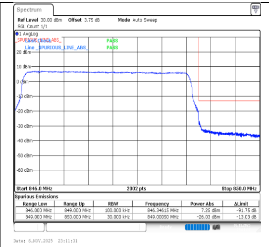
Band26(824-849)-3MHz-16QAM-27025-15RB#0-PASS
