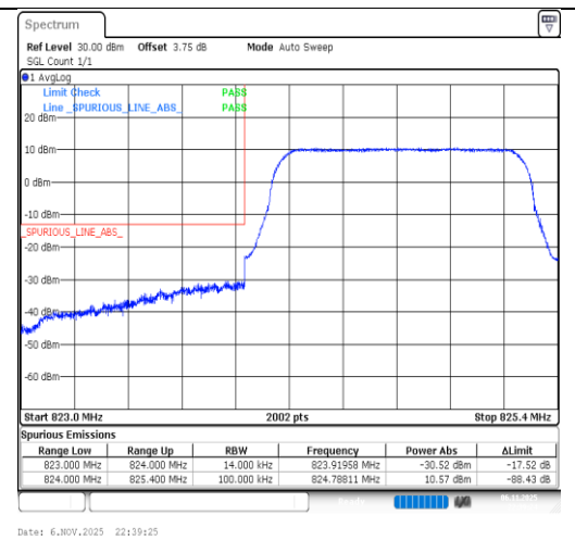
Band26(824-849)-1.4MHz-64QAM-26797- 6RB#0-PASS
