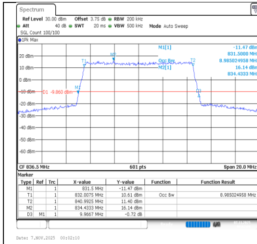
Band26(824-849)-10MHz-QPSK-26915-50RB#0-PASS
