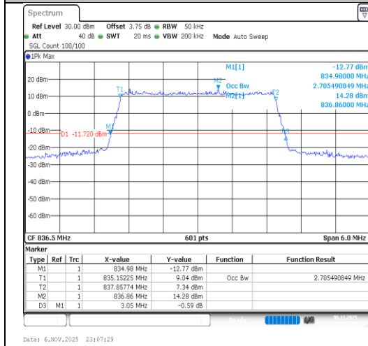
Band26(824-849)-3MHz-16QAM-26915-15RB#0-PASS
