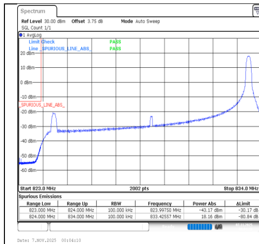
Band26(824-849)-10MHz-64QAM-26840-1RB#49-PASS
