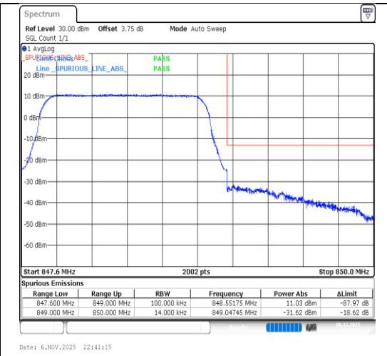
Band26(824-849)-1.4MHz-16QAM-27033-6RB#0-PASS
