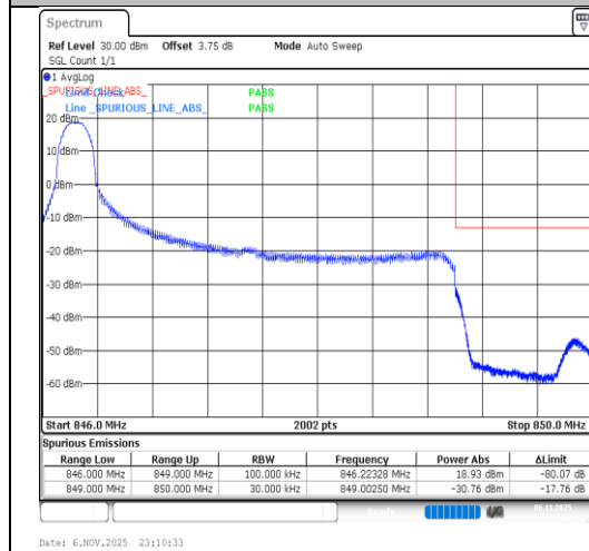
Band26(824-849)-3MHz-64QAM-27025-1RB#0-PASS
