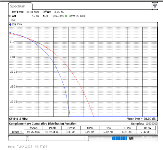
Band26(824-849)-15MHz-64QAM-26965- 75RB#0-PASS
