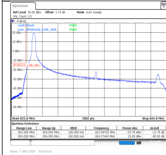
Band26(824-849)-10MHz-QPSK-26840-1RB#0-PASS
