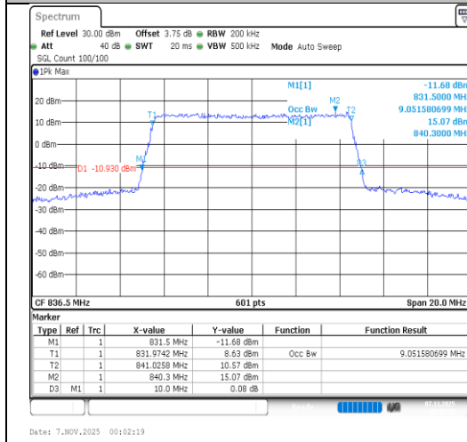
Band26(824-849)-10MHz-16QAM-26915-50RB#0-PASS
