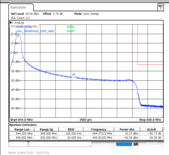
Band26(824-849)-5MHz-16QAM-27015-1RB#0-PASS
