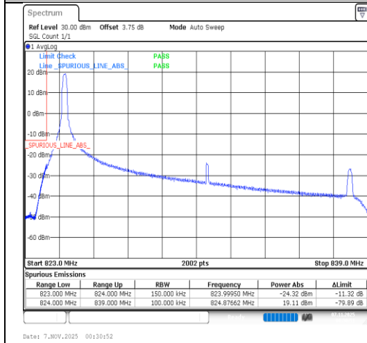
Band26(824-849)-15MHz-QPSK-26865-1RB#0-PASS
