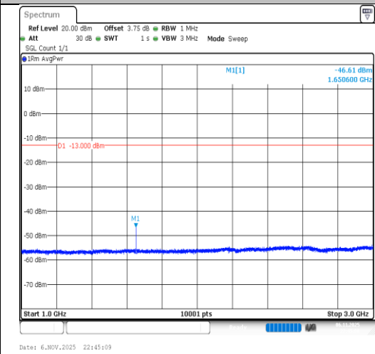
Band26(824-849)-1.4MHz-64QAM-26797- 1RB#5-1000~3000-PASS
