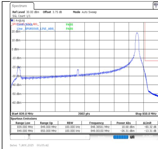
Band26(824-849)-10MHz-16QAM-26990-1RB#49-PASS
