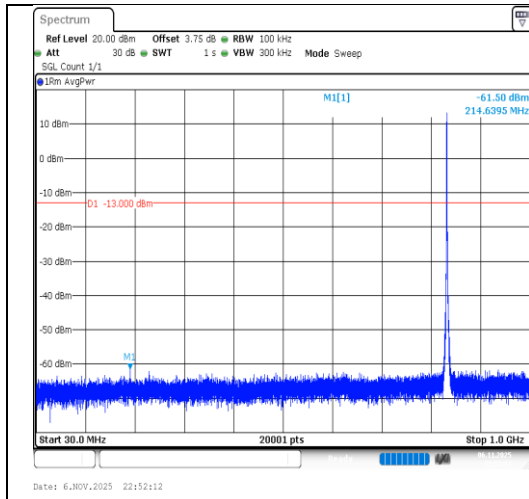
Band26(824-849)-1.4MHz-64QAM-26915- 6RB#0-30~1000-PASS
