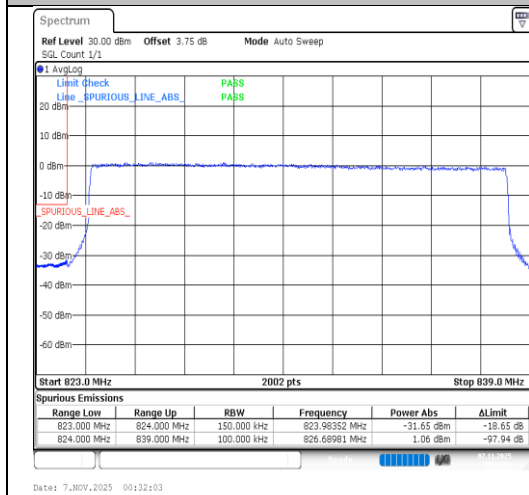
Band26(824-849)-15MHz-QPSK-26865-75RB#0-PASS
