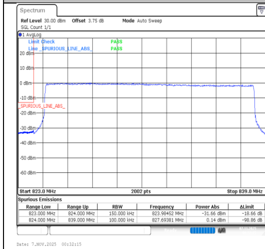
Band26(824-849)-15MHz-16QAM-26865-75RB#0-PASS
