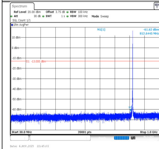
Band26(824-849)-1.4MHz-64QAM-26797- 1RB#5-30~1000-PASS
