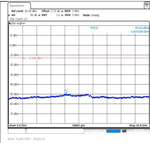
Band26(824-849)-1.4MHz-64QAM-26797- 1RB#0-3000~10000-PASS
