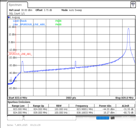
Band26(824-849)-15MHz-16QAM-26865-1RB#74-PASS
