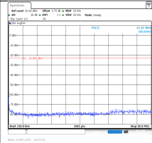
Band26(824-849)-1.4MHz-64QAM-27033- 1RB#5-0.15~30-PASS
