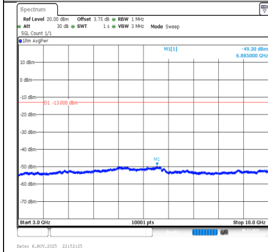
Band26(824-849)-1.4MHz-64QAM-26915- 6RB#0-3000~10000-PASS
