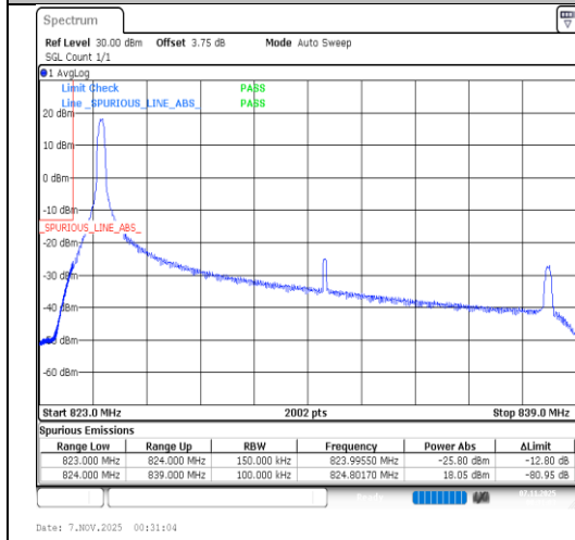
Band26(824-849)-15MHz-16QAM-26865-1RB#0-PASS
