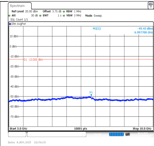
Band26(824-849)-1.4MHz-64QAM-27033- 1RB#0-3000~10000-PASS
