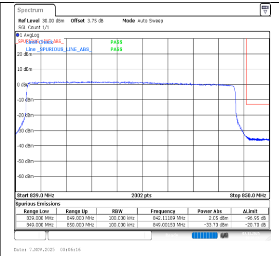
Band26(824-849)-10MHz-16QAM-26990-50RB#0-PASS
