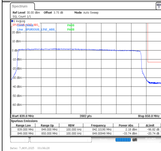
Band26(824-849)-10MHz-64QAM-26990-50RB#0-PASS
