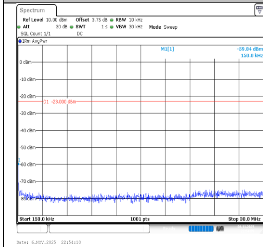
Band26(824-849)-1.4MHz-64QAM-27033-1RB#0-0.15~30-PASS
