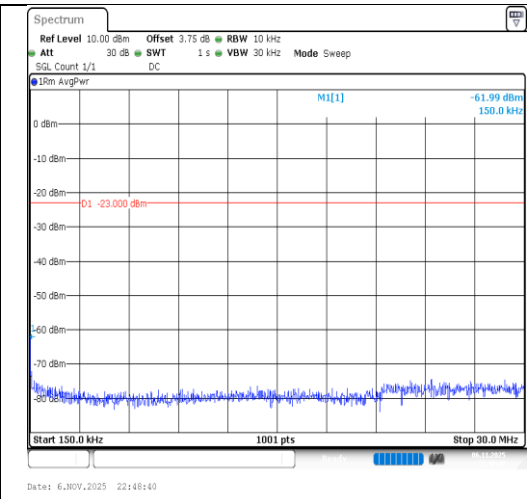
Band26(824-849)-1.4MHz-64QAM-26915- 1RB#0-0.15~30-PASS
