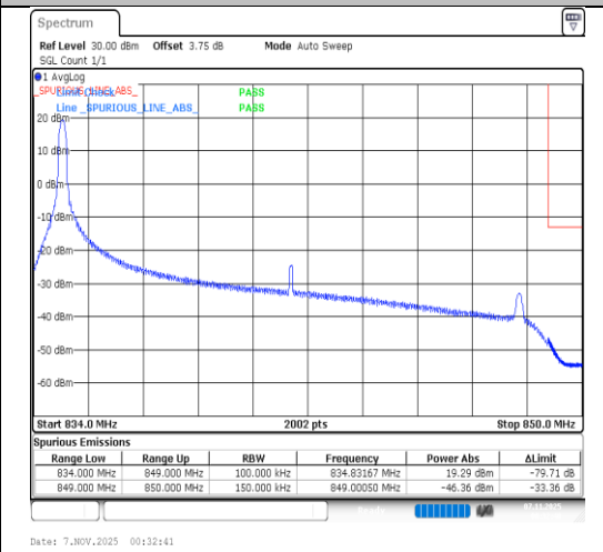
Band26(824-849)-15MHz-QPSK-26965-1RB#0-PASS
