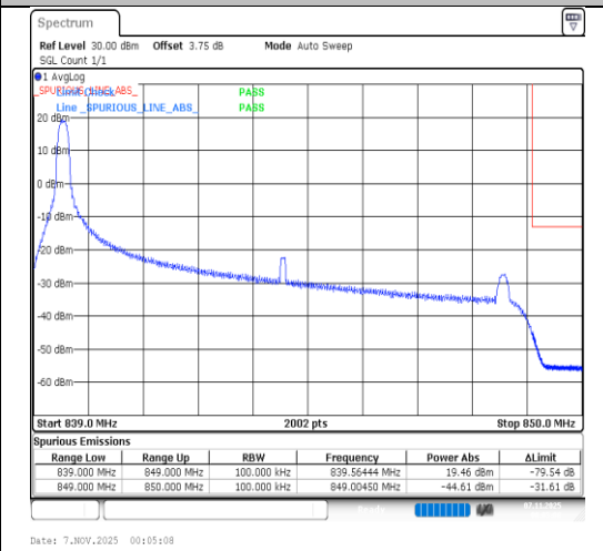
Band26(824-849)-10MHz-16QAM-26990-1RB#0-PASS
