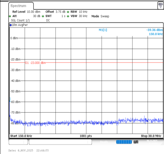
Band26(824-849)-1.4MHz-64QAM-26797- 1RB#5-0.15~30-PASS
