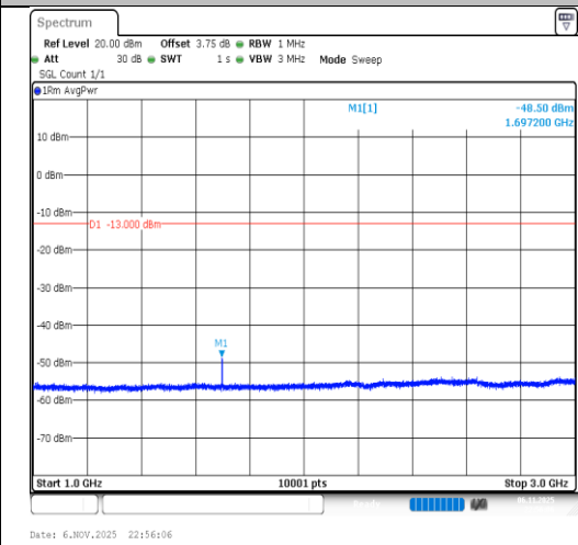
Band26(824-849)-1.4MHz-64QAM-27033- 1RB#5-1000~3000-PASS
