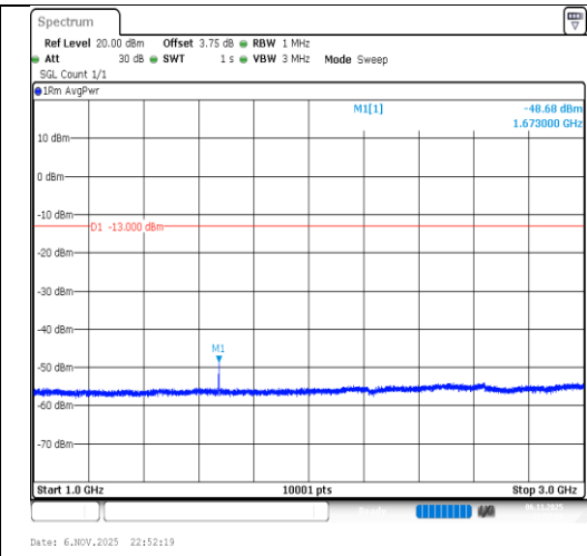
Band26(824-849)-1.4MHz-64QAM-26915- 6RB#0-1000~3000-PASS
