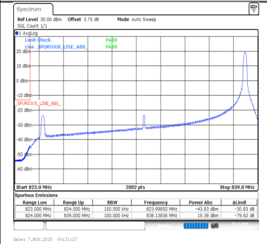
Band26(824-849)-15MHz-QPSK-26865-1RB#74-PASS
