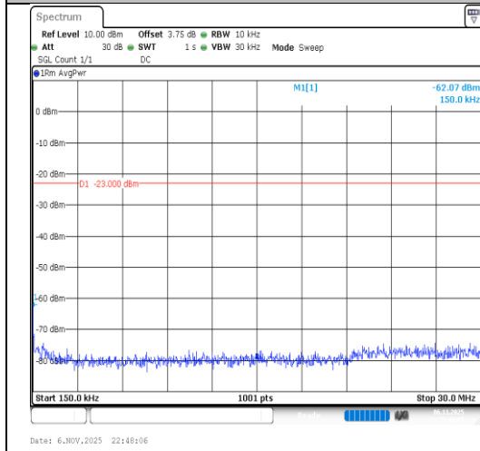
Band26(824-849)-1.4MHz-16QAM-26915- 1RB#0-0.15~30-PASS
