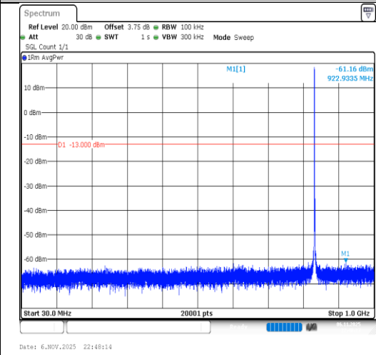
Band26(824-849)-1.4MHz-16QAM-26915- 1RB#0-30~1000-PASS
