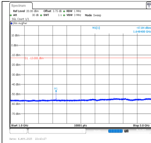
Band26(824-849)-1.4MHz-64QAM-26797- 1RB#0-1000~3000-PASS
