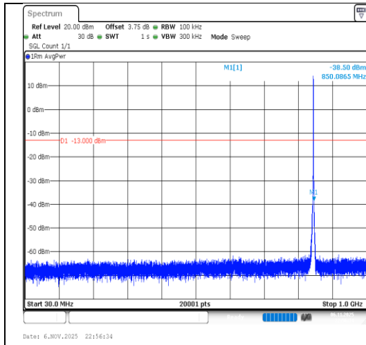
Band26(824-849)-1.4MHz-QPSK-27033-6RB#0-30~1000-PASS
