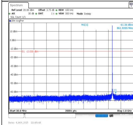
Band26(824-849)-1.4MHz-64QAM-26915- 1RB#0-30~1000-PASS
