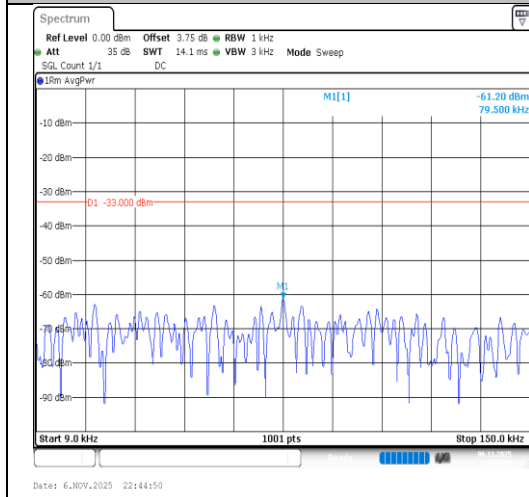
Band26(824-849)-1.4MHz-64QAM-26797- 1RB#5-0.009~0.15-PASS
