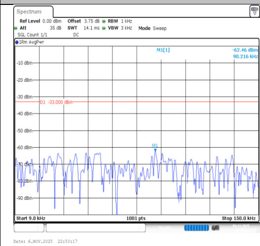
Band26(824-849)-1.4MHz-64QAM-26915- 1RB#5-0.009~0.15-PASS
