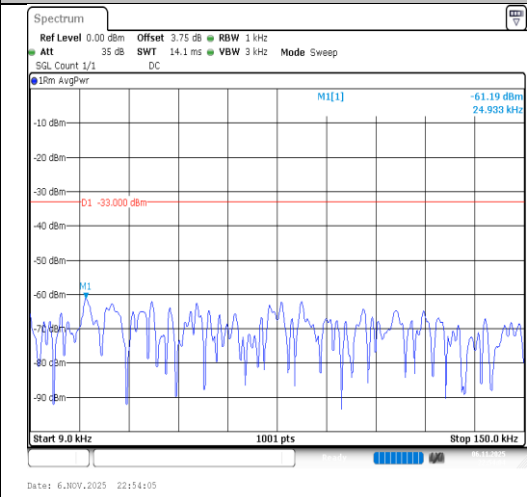
Band26(824-849)-1.4MHz-64QAM-27033-1RB#0-0.009~0.15-PASS
