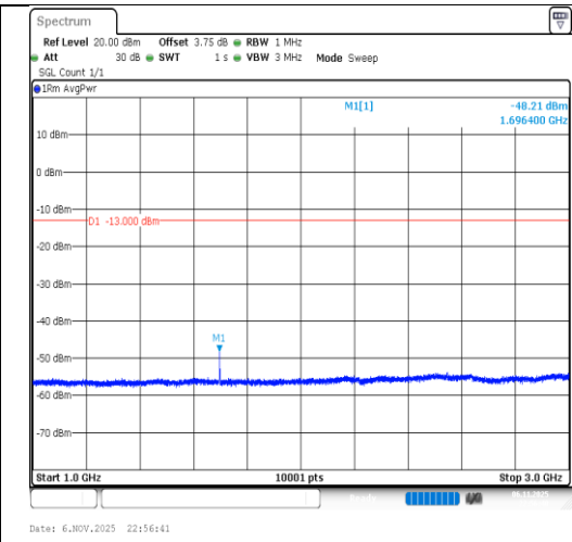
Band26(824-849)-1.4MHz-QPSK-27033-6RB#0-1000~3000-PASS
