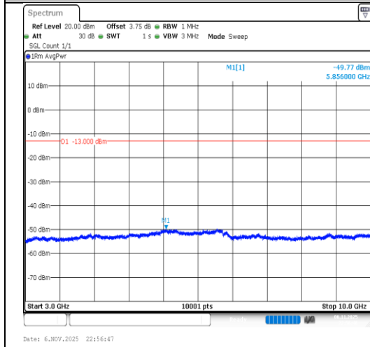
Band26(824-849)-1.4MHz-QPSK-27033-6RB#0-3000~10000-PASS
