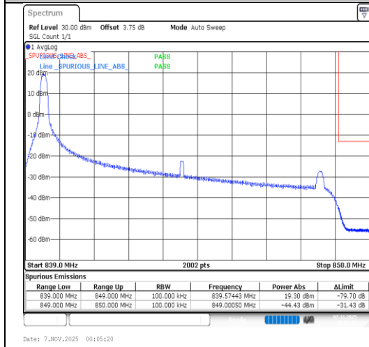
Band26(824-849)-10MHz-64QAM-26990-1RB#0-PASS
