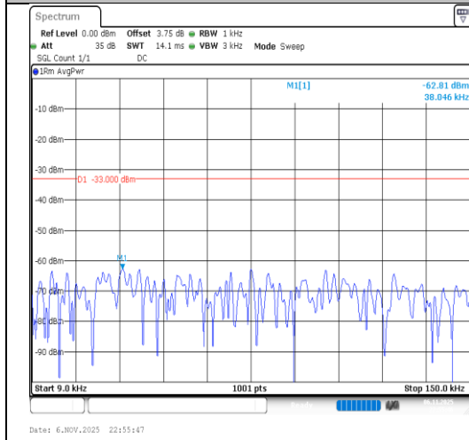
Band26(824-849)-1.4MHz-64QAM-27033- 1RB#5-0.009~0.15-PASS
