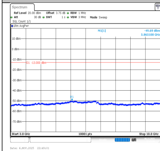
Band26(824-849)-1.4MHz-64QAM-26915- 1RB#0-3000~10000-PASS
