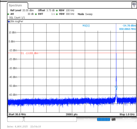
Band26(824-849)-1.4MHz-64QAM-27033-1RB#0-30~1000-PASS
