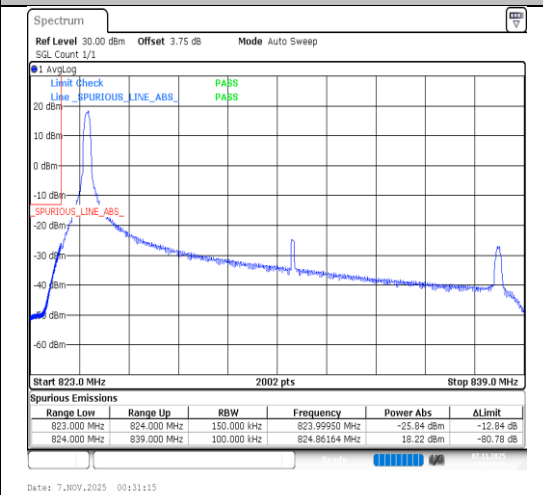
Band26(824-849)-15MHz-64QAM-26865-1RB#0-PASS
