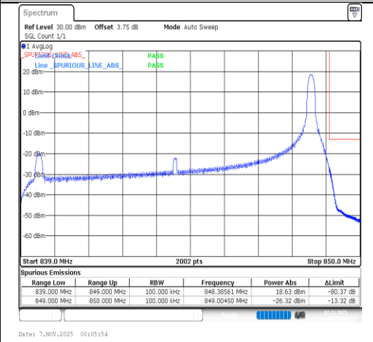
Band26(824-849)-10MHz-64QAM-26990-1RB#49-PASS
