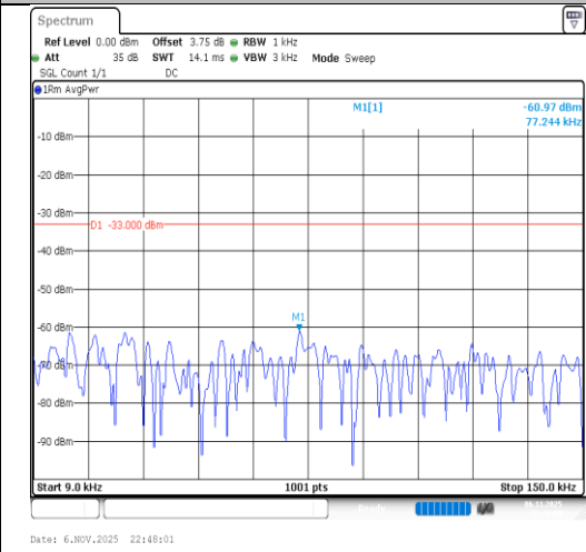
Band26(824-849)-1.4MHz-16QAM-26915- 1RB#0-0.009~0.15-PASS
