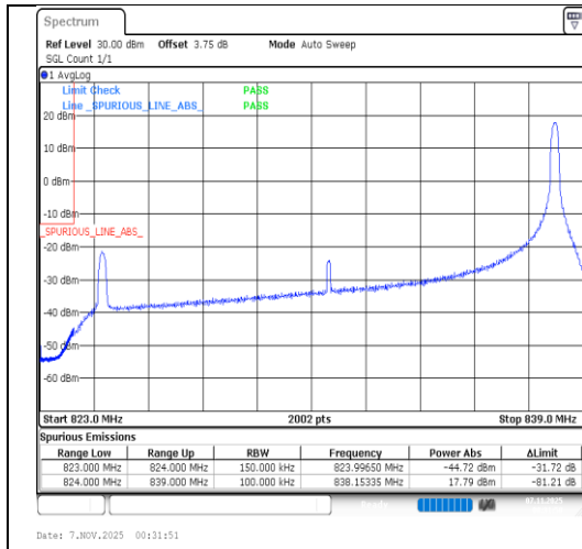
Band26(824-849)-15MHz-64QAM-26865-1RB#74-PASS
