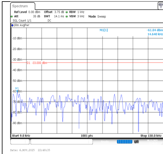
Band26(824-849)-1.4MHz-64QAM-26915- 1RB#0-0.009~0.15-PASS
