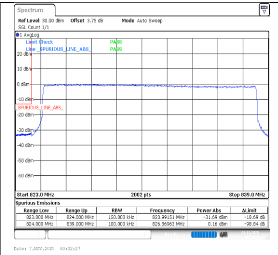
Band26(824-849)-15MHz-64QAM-26865-75RB#0-PASS
