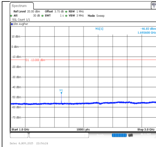
Band26(824-849)-1.4MHz-64QAM-27033- 1RB#0-1000~3000-PASS
