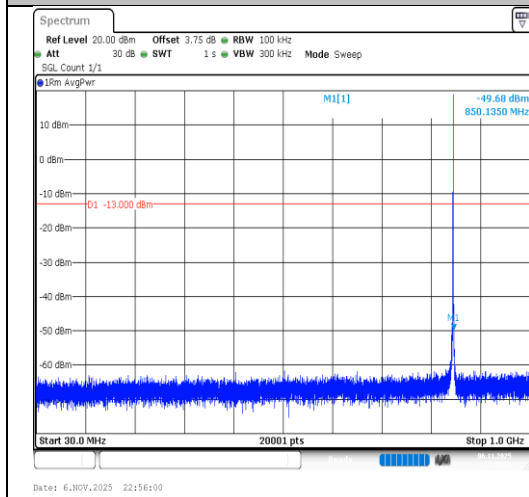
Band26(824-849)-1.4MHz-64QAM-27033- 1RB#5-30~1000-PASS
