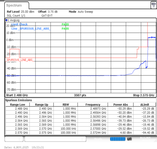
Band38-5MHz-64QAM-37775-25RB#0-PASS
