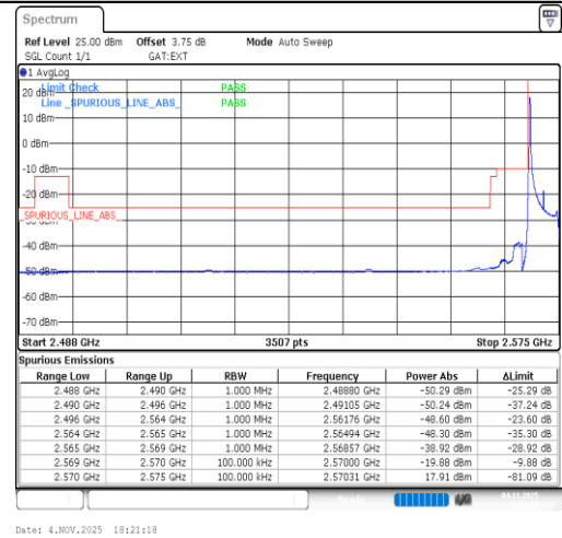
Band38-5MHz-64QAM-37775-1RB#0-PASS
