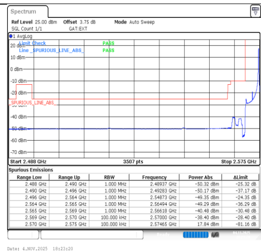
Band38-5MHz-QPSK-37775-1RB#24-PASS
