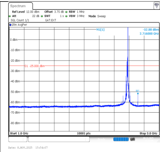
Band38-15MHz-64QAM-37825-1RB#74- 1000~3000-PASS
