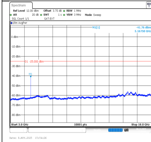
Band38-15MHz-64QAM-37825-1RB#74- 3000~18000-PASS
