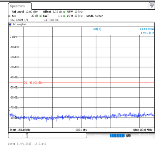
Band38-15MHz-64QAM-37825-75RB#0- 0.15~30-PASS
