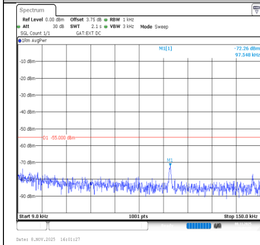
Band38-15MHz-64QAM-37825-75RB#0- 0.009~0.15-PASS
