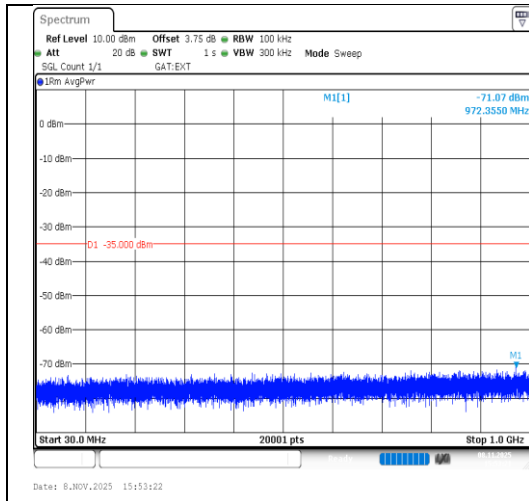
Band38-15MHz-64QAM-37825-1RB#74- 30~1000-PASS
