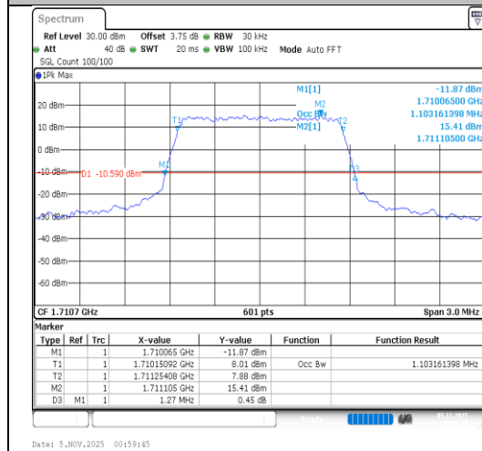
Band4-1.4MHz-16QAM-19957-6RB#0-PASS
