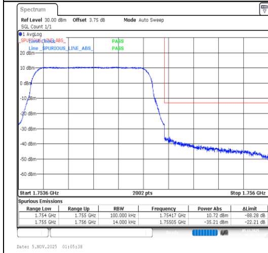
Band4-1.4MHz-64QAM-20393-6RB#0-PASS
