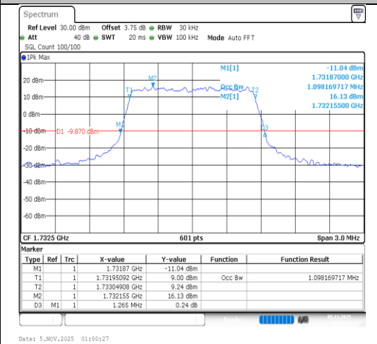
Band4-1.4MHz-QPSK-20175-6RB#0-PASS
