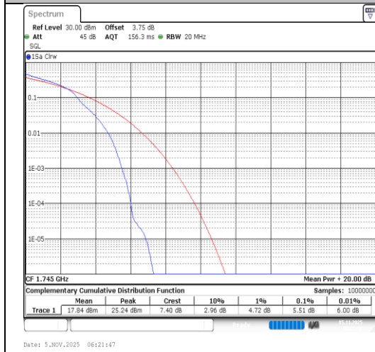
Band4-20MHz-16QAM-20300-1RB#0-PASS
