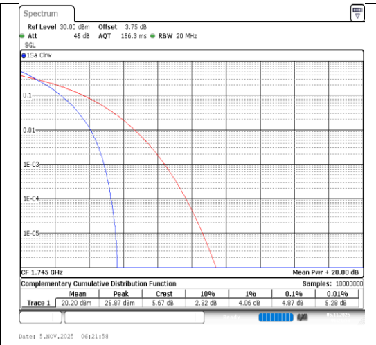
Band4-20MHz-QPSK-20300-100RB#0-PASS
