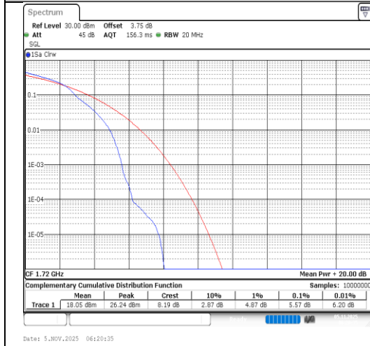
Band4-20MHz-16QAM-20050-1RB#0-PASS
