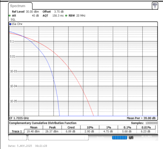
Band4-20MHz-16QAM-20175-100RB#0-PASS
