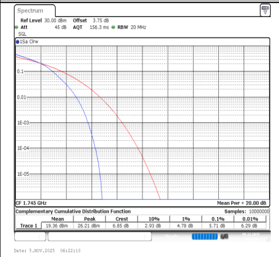
Band4-20MHz-64QAM-20300-100RB#0-PASS
