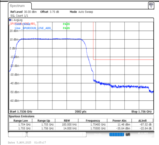
Band4-1.4MHz-QPSK-20393-6RB#0-PASS
