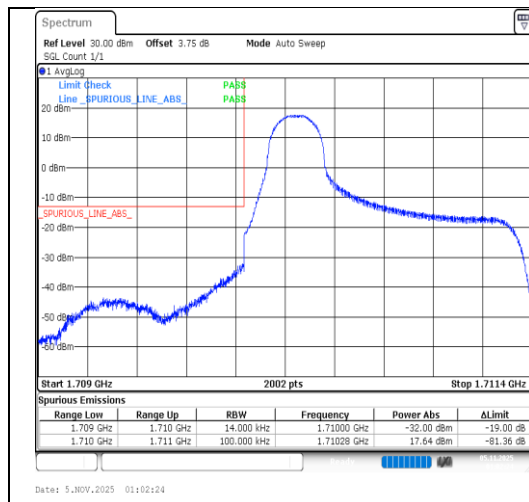
Band4-1.4MHz-16QAM-19957-1RB#0-PASS
