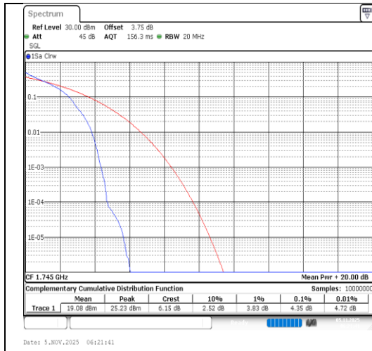
Band4-20MHz-QPSK-20300-1RB#0-PASS
