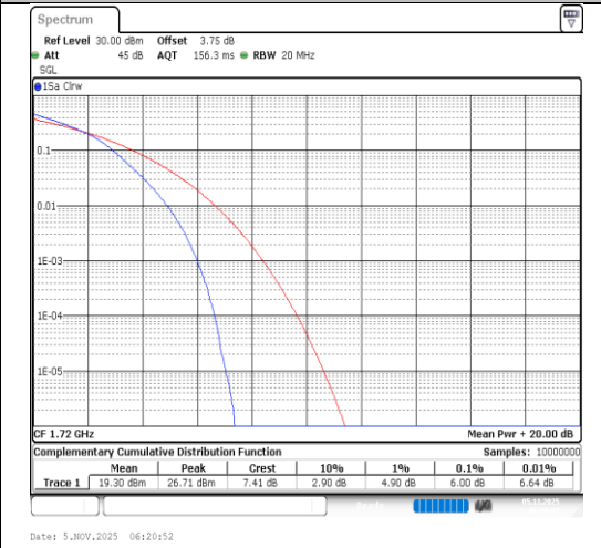
Band4-20MHz-16QAM-20050-100RB#0-PASS
