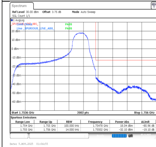
Band4-1.4MHz-16QAM-20393-1RB#5-PASS
