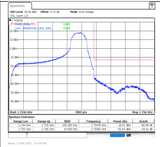
Band4-1.4MHz-64QAM-20393-1RB#5-PASS
