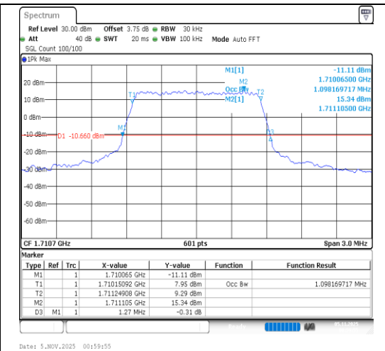
Band4-1.4MHz-64QAM-19957-6RB#0-PASS
