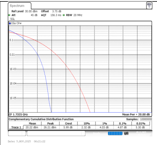
Band4-20MHz-QPSK-20175-100RB#0-PASS
