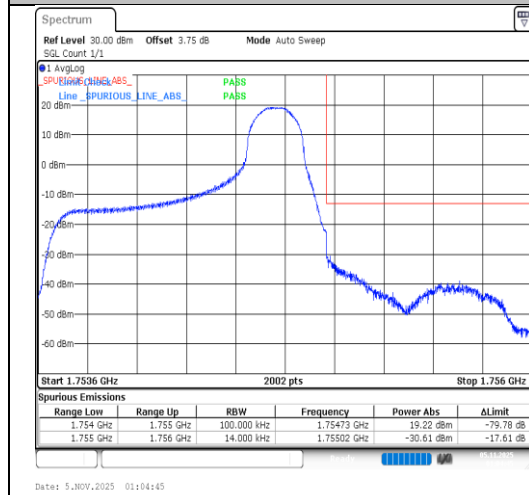
Band4-1.4MHz-QPSK-20393-1RB#5-PASS
