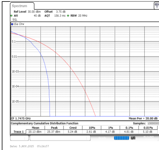
Band4-15MHz-QPSK-20325-1RB#0-PASS
