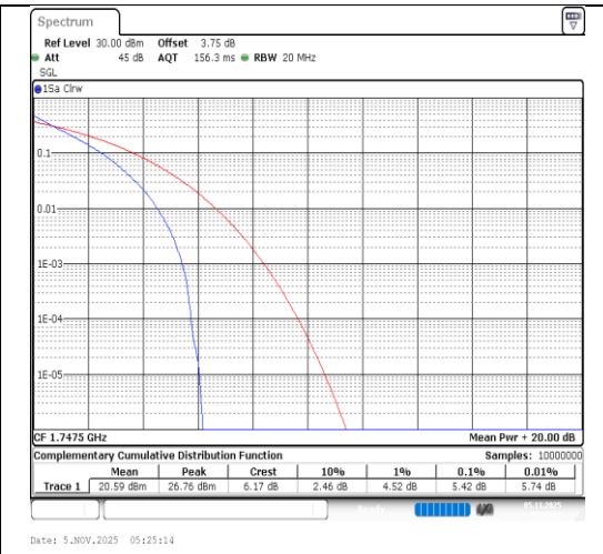
Band4-15MHz-QPSK-20325-75RB#0-PASS
