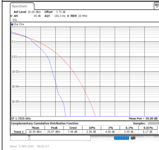
Band4-20MHz-64QAM-20175-1RB#0-PASS
