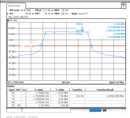
Band4-1.4MHz-16QAM-20175-6RB#0-PASS
