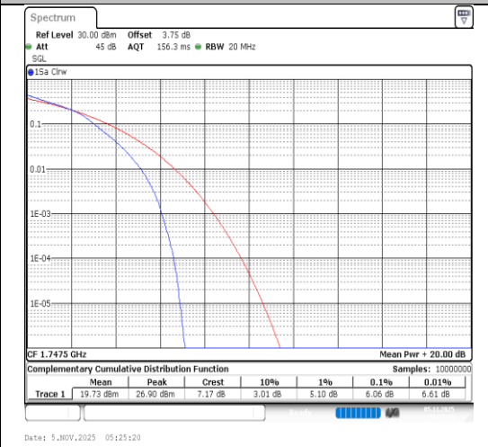
Band4-15MHz-16QAM-20325-75RB#0-PASS
