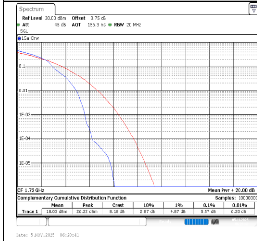
Band4-20MHz-64QAM-20050-1RB#0-PASS
