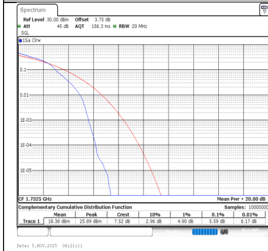
Band4-20MHz-16QAM-20175-1RB#0-PASS
