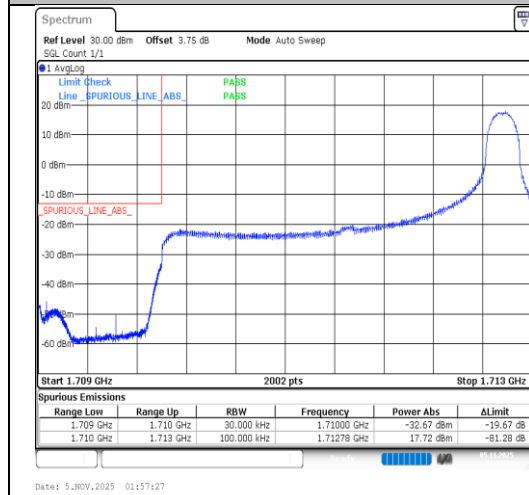
Band4-3MHz-64QAM-19965-1RB#14-PASS
