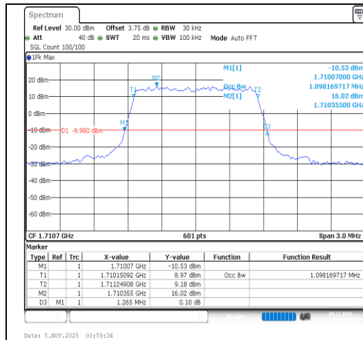
Band4-1.4MHz-QPSK-19957-6RB#0-PASS
