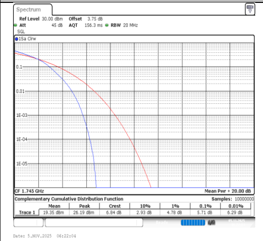
Band4-20MHz-16QAM-20300-100RB#0-PASS
