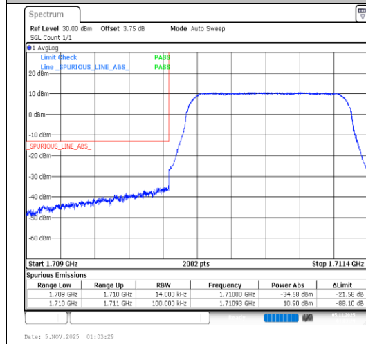
Band4-1.4MHz-16QAM-19957-6RB#0-PASS
