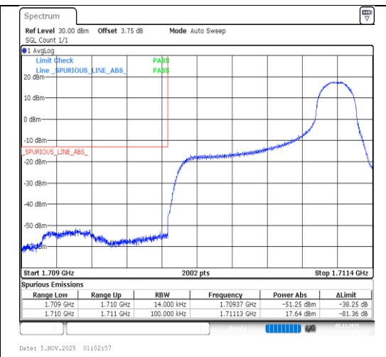
Band4-1.4MHz-16QAM-19957-1RB#5-PASS
