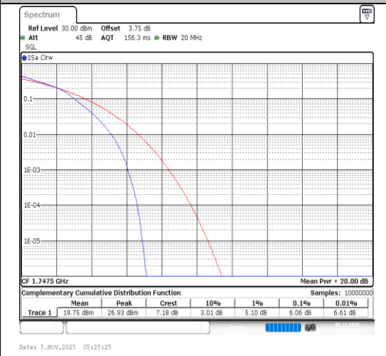
Band4-15MHz-64QAM-20325-75RB#0-PASS
