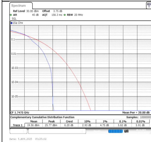
Band4-15MHz-16QAM-20325-1RB#0-PASS
