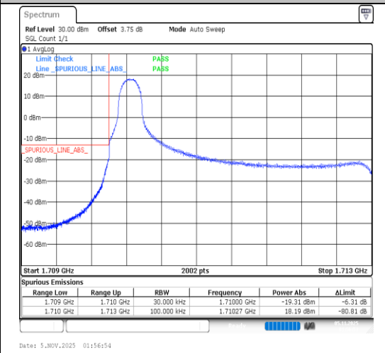
Band4-3MHz-64QAM-19965-1RB#0-PASS
