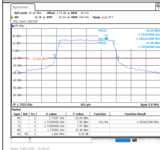
Band4-1.4MHz-64QAM-20175-6RB#0-PASS
