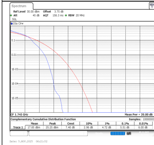
Band4-20MHz-64QAM-20300-1RB#0-PASS
