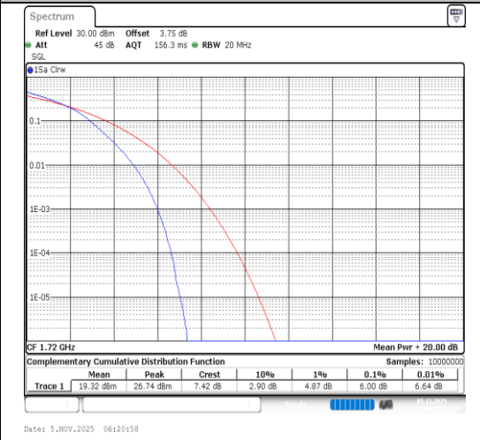
Band4-20MHz-64QAM-20050-100RB#0-PASS
