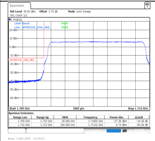
Band4-3MHz-64QAM-19965-15RB#0-PASS
