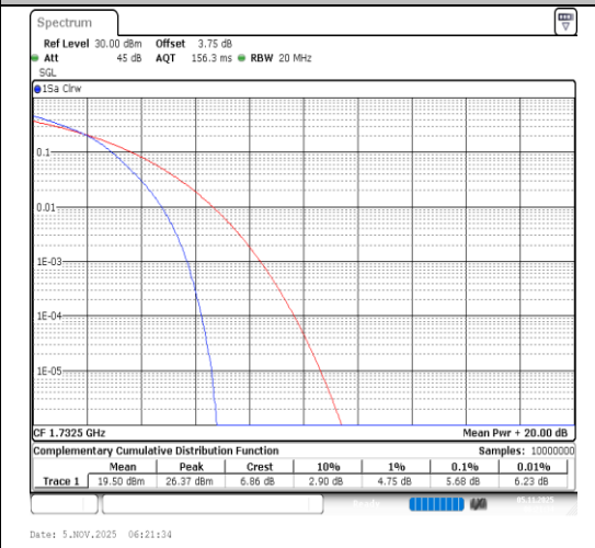
Band4-20MHz-64QAM-20175-100RB#0-PASS
