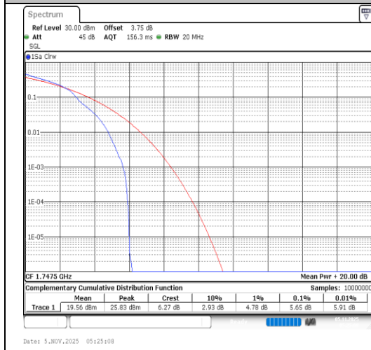
Band4-15MHz-64QAM-20325-1RB#0-PASS
