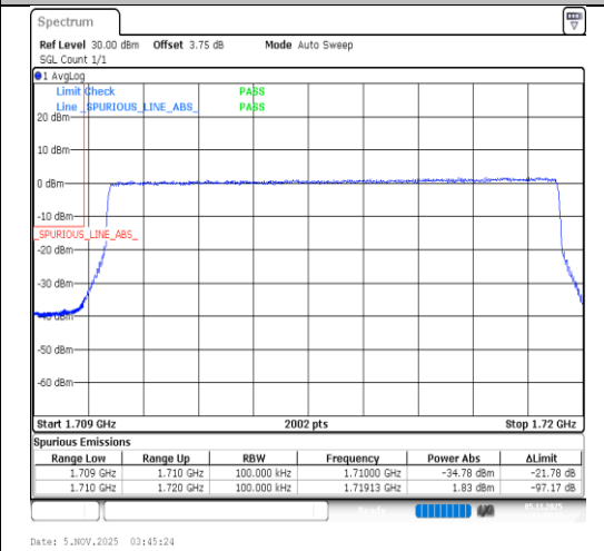
Band4-10MHz-64QAM-20000-50RB#0-PASS
