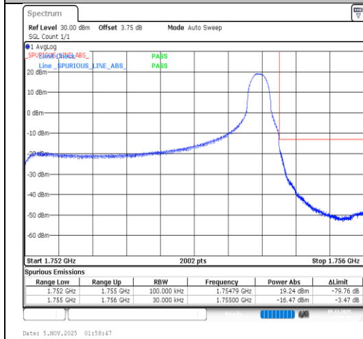
Band4-3MHz-QPSK-20385-1RB#14-PASS
