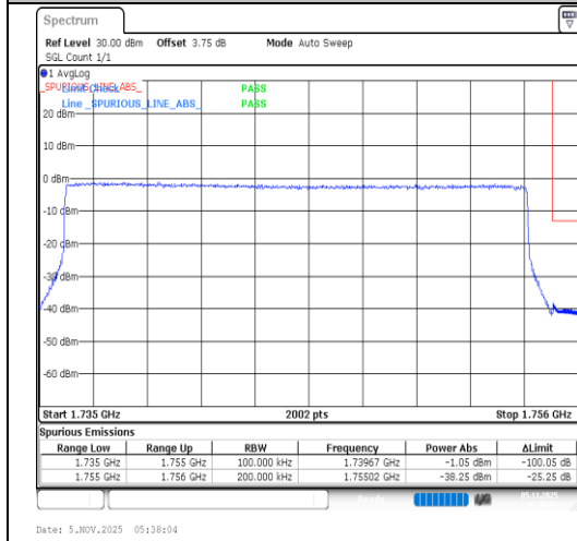
Band4-20MHz-64QAM-20300-100RB#0-PASS
