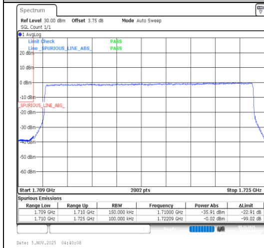
Band4-15MHz-16QAM-20025-75RB#0-PASS
