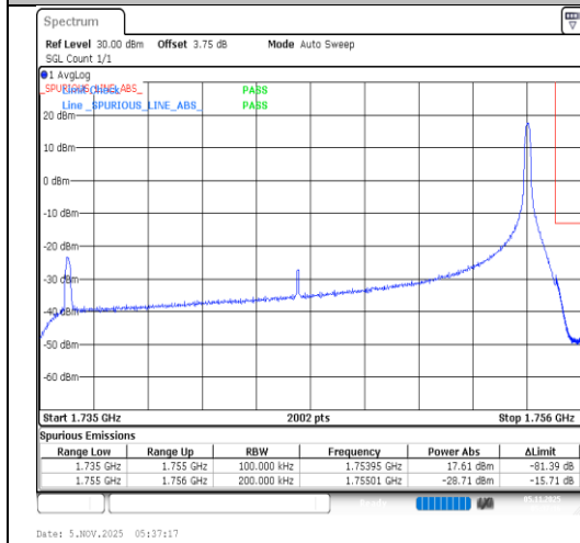
Band4-20MHz-16QAM-20300-1RB#99-PASS
