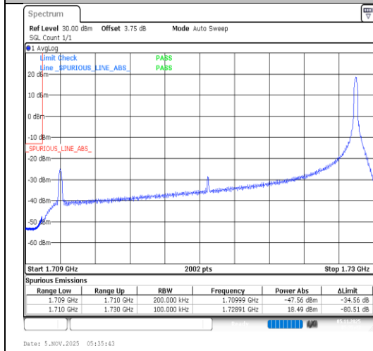
Band4-20MHz-64QAM-20050-1RB#99-PASS
