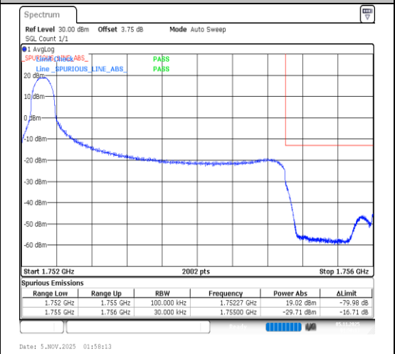
Band4-3MHz-QPSK-20385-1RB#0-PASS
