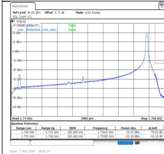
Band4-15MHz-QPSK-20325-1RB#74-PASS
