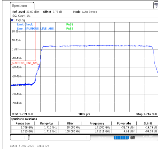
Band4-5MHz-16QAM-19975-25RB#0-PASS
