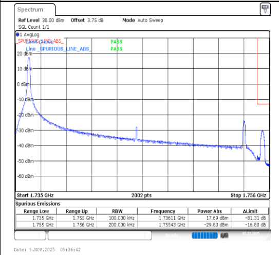
Band4-20MHz-16QAM-20300-1RB#0-PASS
