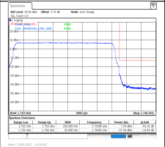
Band4-3MHz-QPSK-20385-15RB#0-PASS
