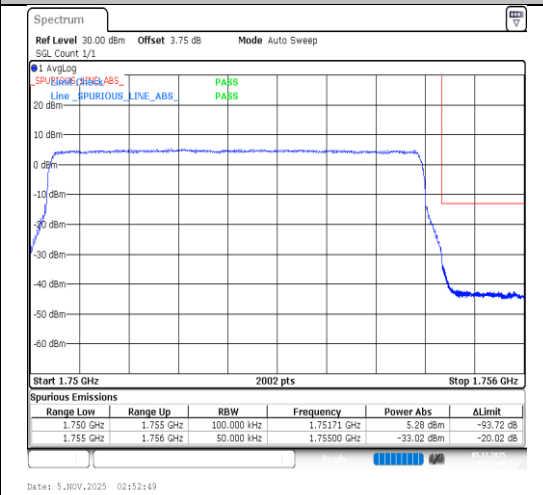
Band4-5MHz-QPSK-20375-25RB#0-PASS
