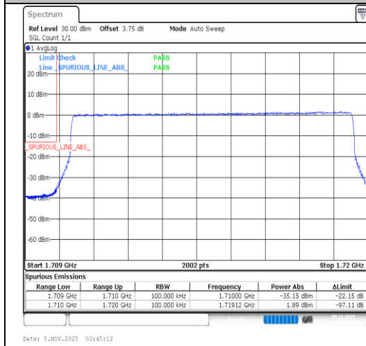
Band4-10MHz-16QAM-20000-50RB#0-PASS
