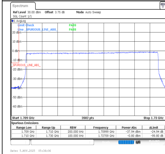
Band4-20MHz-16QAM-20050-100RB#0-PASS
