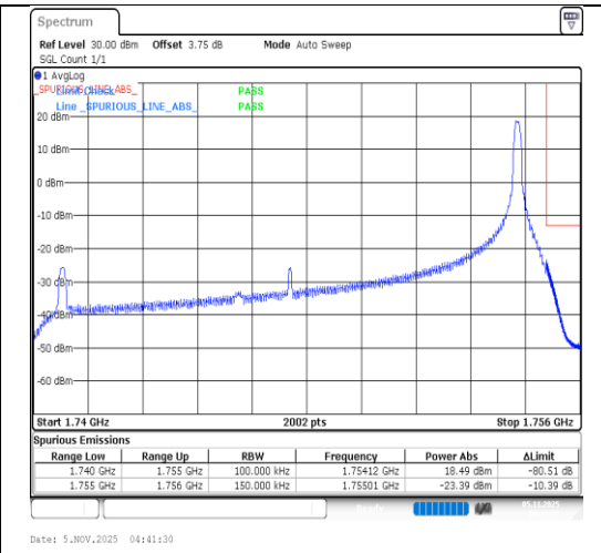
Band4-15MHz-64QAM-20325-1RB#74-PASS
