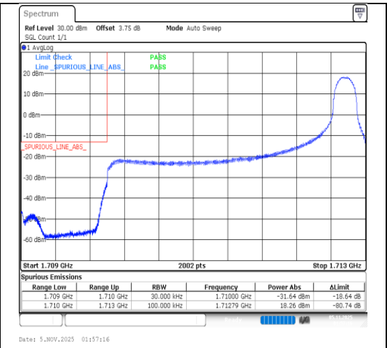
Band4-3MHz-16QAM-19965-1RB#14-PASS
