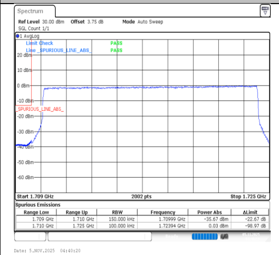
Band4-15MHz-64QAM-20025-75RB#0-PASS
