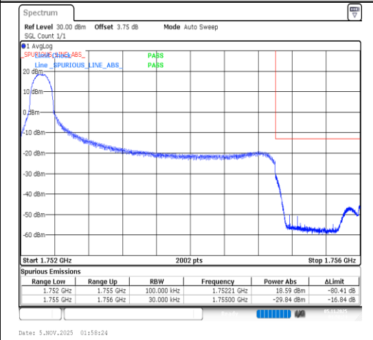
Band4-3MHz-16QAM-20385-1RB#0-PASS
