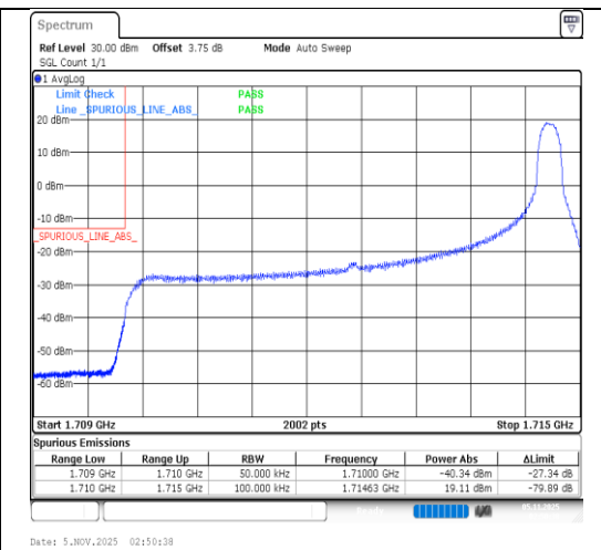
Band4-5MHz-QPSK-19975-1RB#24-PASS
