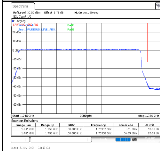
Band4-10MHz-64QAM-20350-50RB#0-PASS
