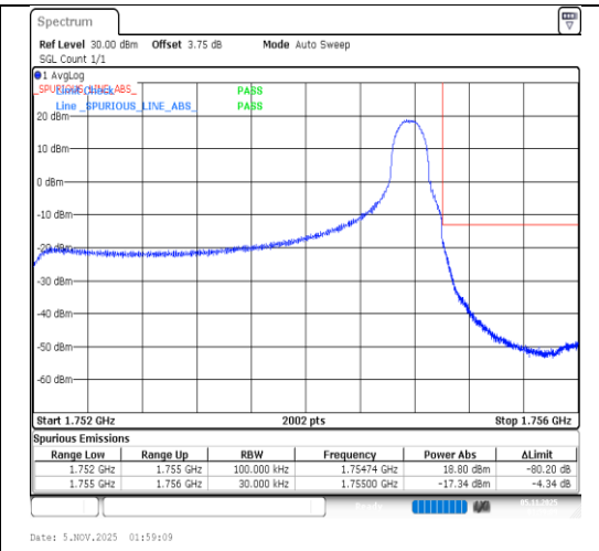
Band4-3MHz-64QAM-20385-1RB#14-PASS
