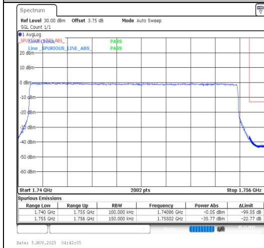
Band4-15MHz-64QAM-20325-75RB#0-PASS
