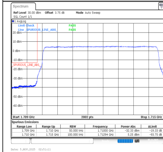
Band4-5MHz-QPSK-19975-25RB#0-PASS
