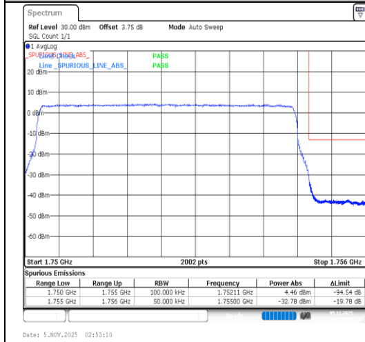
Band4-5MHz-64QAM-20375-25RB#0-PASS
