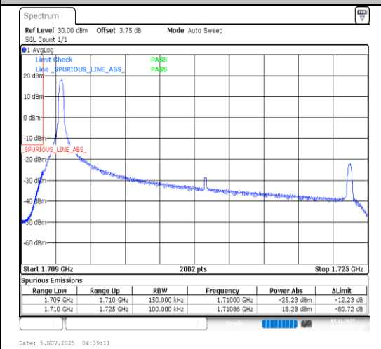
Band4-15MHz-64QAM-20025-1RB#0-PASS
