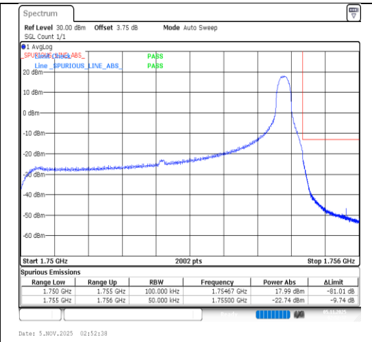
Band4-5MHz-64QAM-20375-1RB#24-PASS
