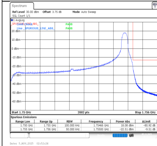
Band4-5MHz-16QAM-20375-1RB#24-PASS
