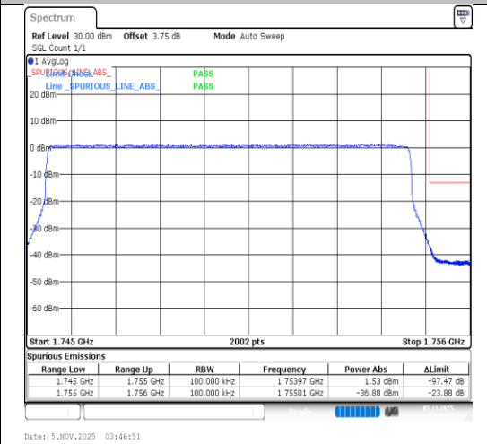
Band4-10MHz-16QAM-20350-50RB#0-PASS
