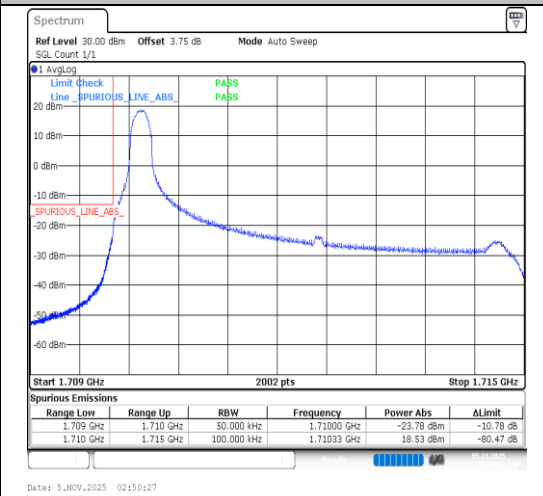
Band4-5MHz-64QAM-19975-1RB#0-PASS
