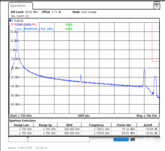
Band4-20MHz-QPSK-20300-1RB#0-PASS
