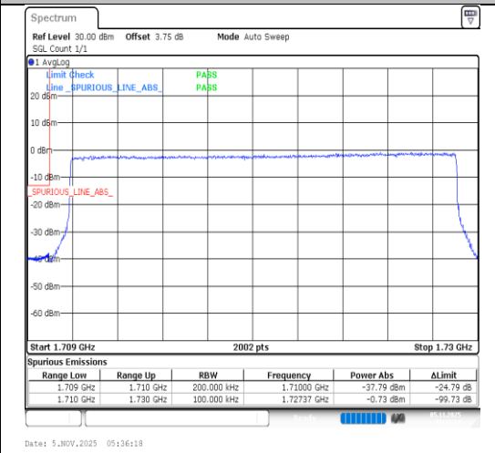
Band4-20MHz-64QAM-20050-100RB#0-PASS
