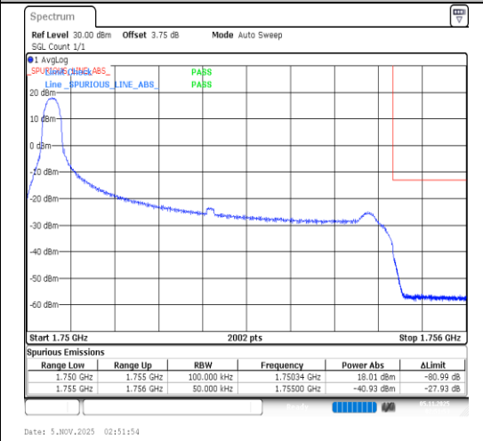
Band4-5MHz-16QAM-20375-1RB#0-PASS
