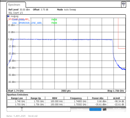
Band4-15MHz-QPSK-20325-75RB#0-PASS
