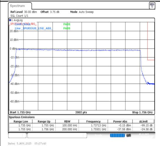
Band4-20MHz-QPSK-20300-100RB#0-PASS
