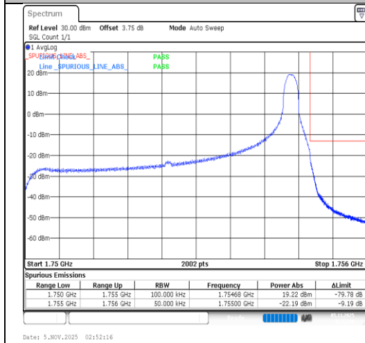
Band4-5MHz-QPSK-20375-1RB#24-PASS
