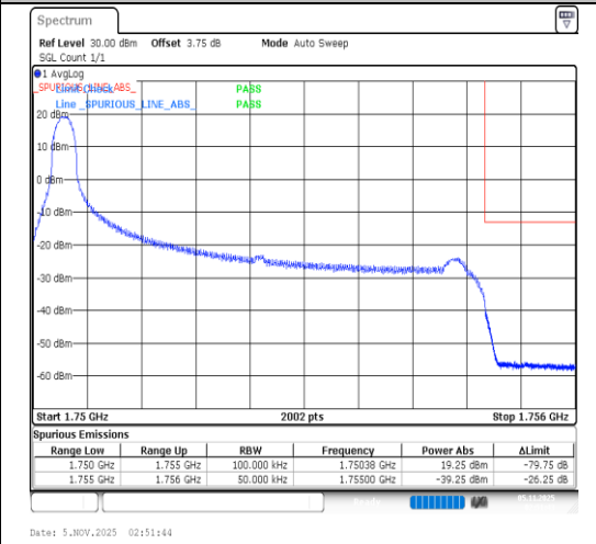
Band4-5MHz-QPSK-20375-1RB#0-PASS
