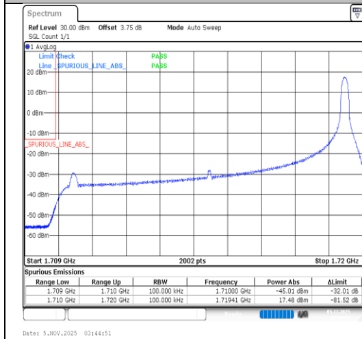
Band4-10MHz-64QAM-20000-1RB#49-PASS
