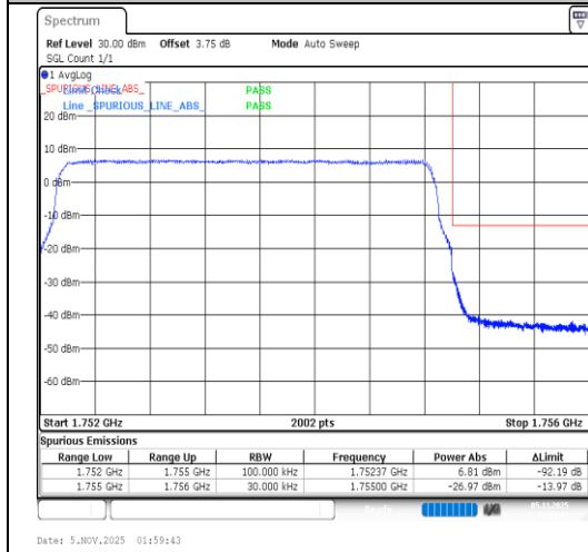
Band4-3MHz-64QAM-20385-15RB#0-PASS
