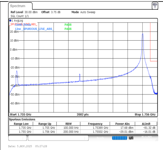
Band4-20MHz-64QAM-20300-1RB#99-PASS
