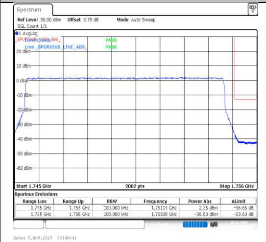
Band4-10MHz-QPSK-20350-50RB#0-PASS
