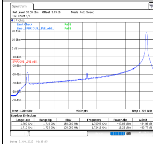
Band4-15MHz-64QAM-20025-1RB#74-PASS
