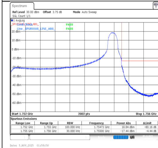
Band4-3MHz-16QAM-20385-1RB#14-PASS
