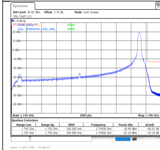
Band4-10MHz-16QAM-20350-1RB#49-PASS
