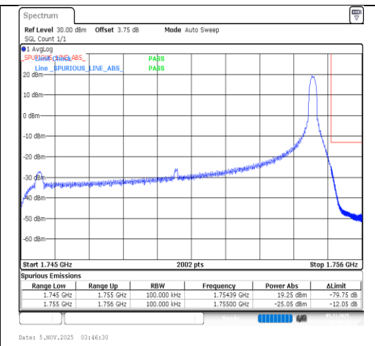
Band4-10MHz-64QAM-20350-1RB#49-PASS
