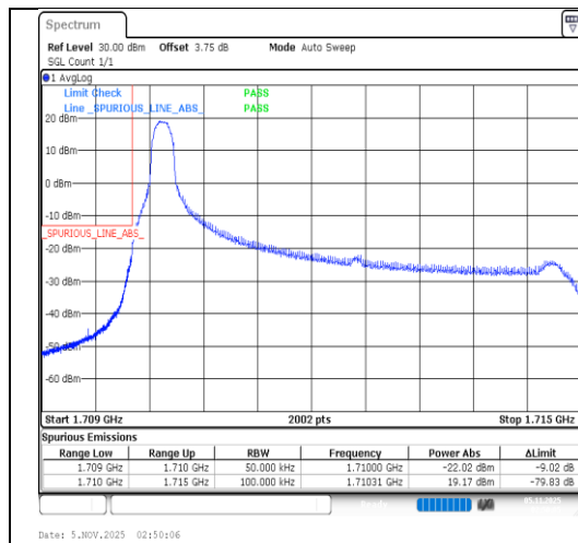
Band4-5MHz-QPSK-19975-1RB#0-PASS
