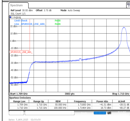
Band4-5MHz-64QAM-19975-1RB#24-PASS
