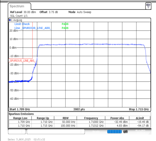
Band4-5MHz-64QAM-19975-25RB#0-PASS
