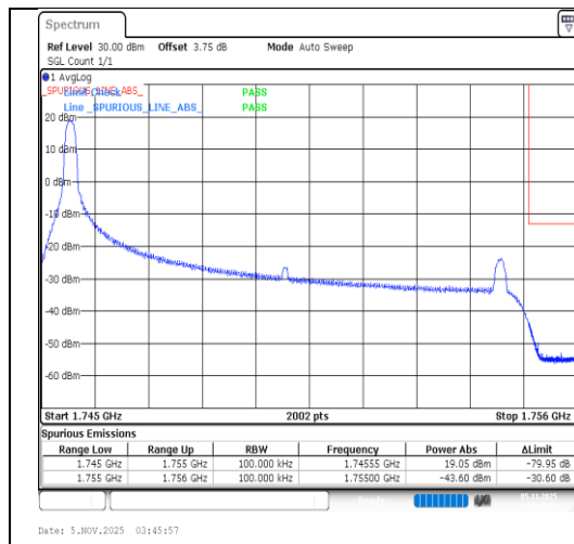
Band4-10MHz-64QAM-20350-1RB#0-PASS
