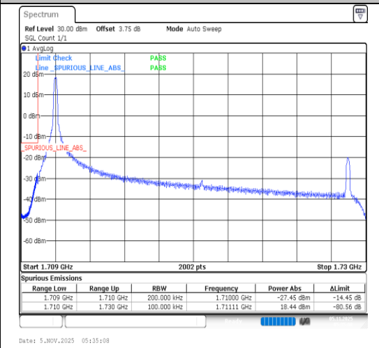
Band4-20MHz-64QAM-20050-1RB#0-PASS
