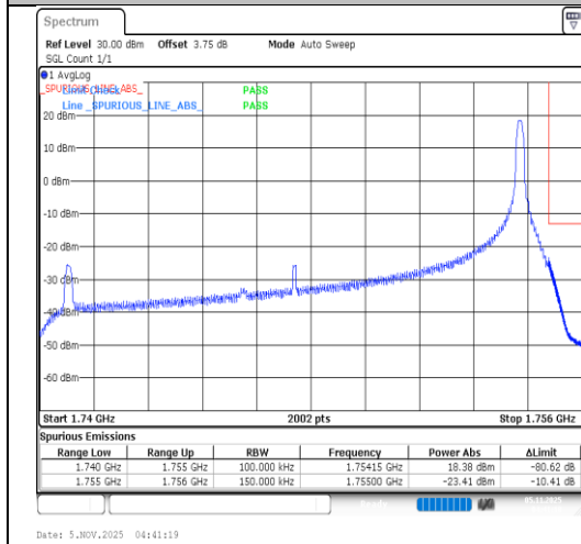
Band4-15MHz-16QAM-20325-1RB#74-PASS
